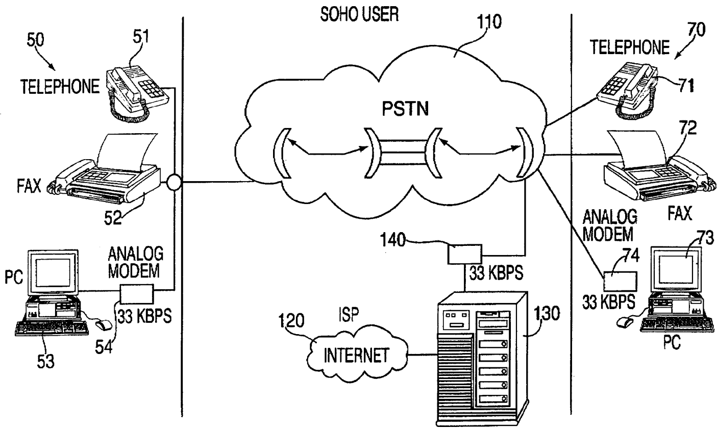
PSTN=PUBLIC SWITCHED TELEPHONE NETWORK FIG. 1
