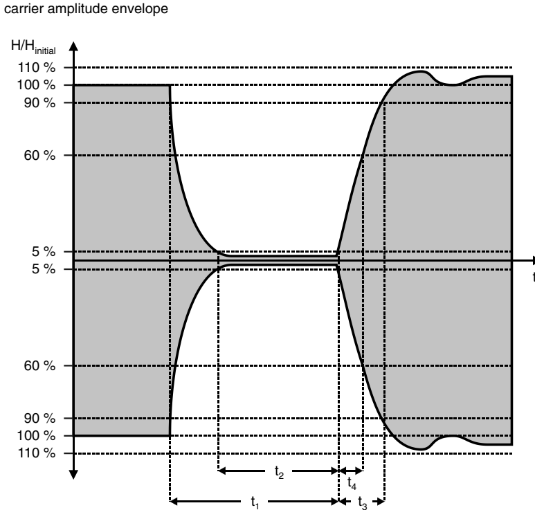
Figure 3.87 Specification of the blanking interval (gap) according to ISO/IEC 14433-2. The maximum duration of the gap is limited to 3\ \mu\text{s} in order to interrupt the energy supply to the card as briefly as possible. Here 2.0\ \mu\text{s} \leq t_1 \leq 3.0\ \mu\text{s} ; 0.5\ \mu\text{s} \leq t_2 \leq t_1 if t_1 > 2.5\ \mu\text{s} , or 0.7\ \mu\text{s} \leq t_2 \leq t_1 if t_1 \leq 2.5\ \mu\text{s} ; and 0\ \mu\text{s} \leq t_4 \leq 0.4\ \mu\text{s}
