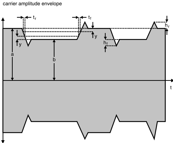
Figure 3.90 Type-B carrier modulation. A continuous supply of energy is made possible by the small modulation index (10 %). Here t_f, t_r \leq 2 \mu\text{s} , y = 0.1 \cdot (a - b) and h_f, h_r \leq 0.1 \cdot (a - b)
