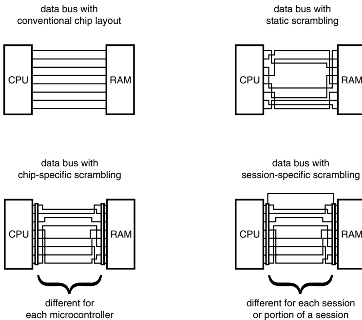
Figure 8.28 Bus scrambling in a smart card microcontroller, illustrated using an 8-bit data bus between the CPU and the RAM. The data bus lines shown here represent information flows rather than electrical leads. The encryption units are shown as separate components for the sake of clarity, but they are actually intermingled with the rest of the components in such a manner that they cannot be recognized as separate components, thus making them immune to attack
