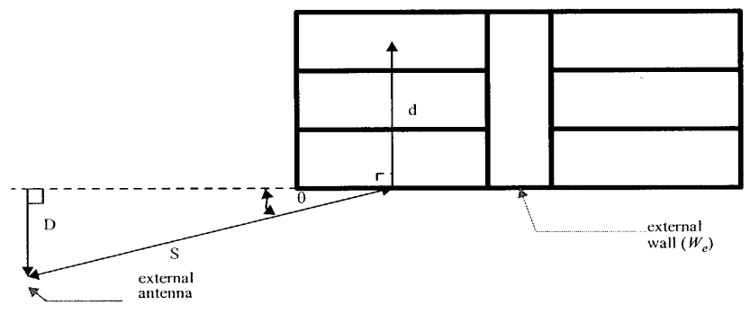
Figure 12 Model for COST 231 building penetration loss model. From E. Damosso and L. Correia, eds., .
