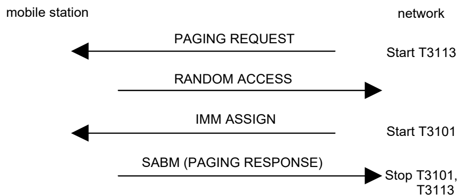
Figure 3.3.2.3.1: Paging sequence
