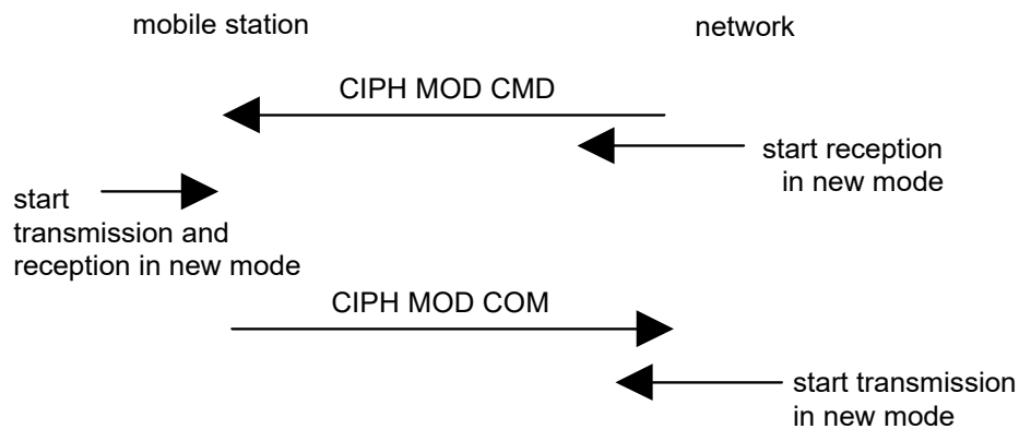
Figure 3.4.7.2.1: Ciphering mode setting sequence
