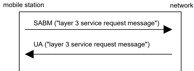
Figure 3.1.5.1: Service request and contention resolution
