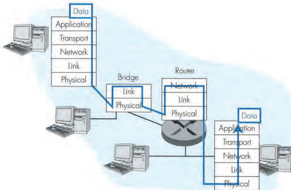
Figure 1.25 + Hosts, routers, and bridges; each contains a different set of layers, reflecting their differences in functionality
