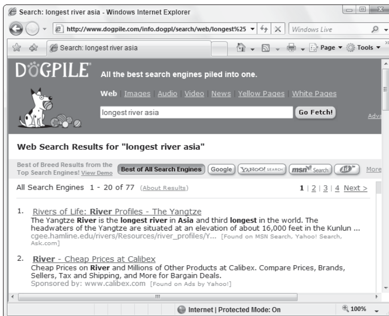
Figure 6-2: Dogpile's search.
