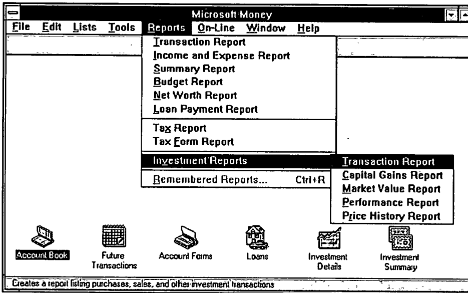
Figure 4.32: Cascading menu.
