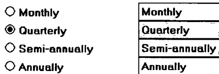
Figure 7.24: Radio buttons.
