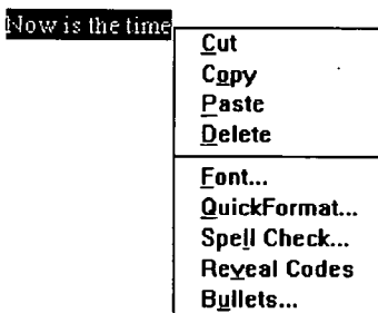
Figure 4.34: Pop-up menu.
