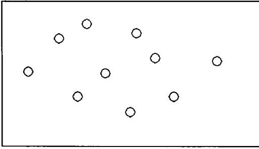
Figure 3.78: A scatterplot.
