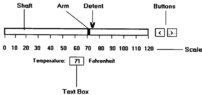
Figure 7.79: Slider.
