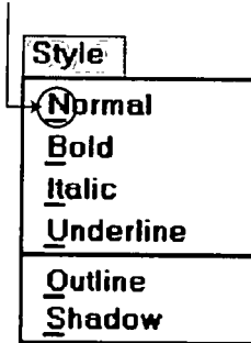
Figure 4.13: Keyboard equivalents.
