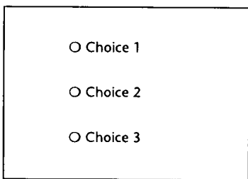
Figure 4.1: Single menu.
