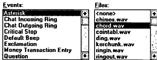
Figure 7.60: List boxes.
