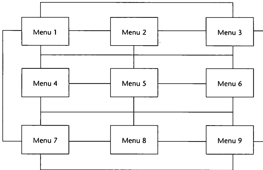
Figure 4.5: Connected menus.
