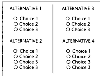
Figure 4.3: Simultaneous menus.
