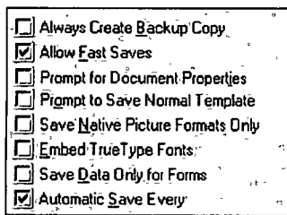
Figure 7.40: Check boxes.
