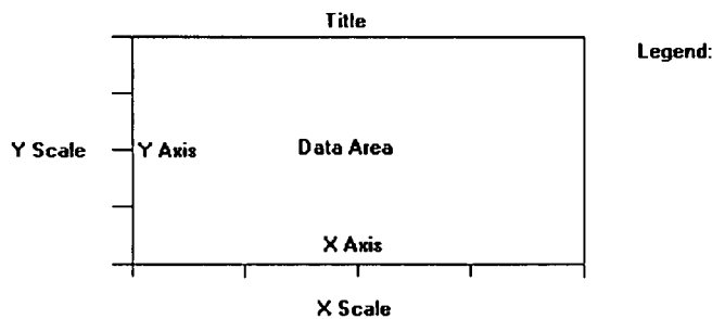
Figure 3.71: Components of a statistical graphic.
