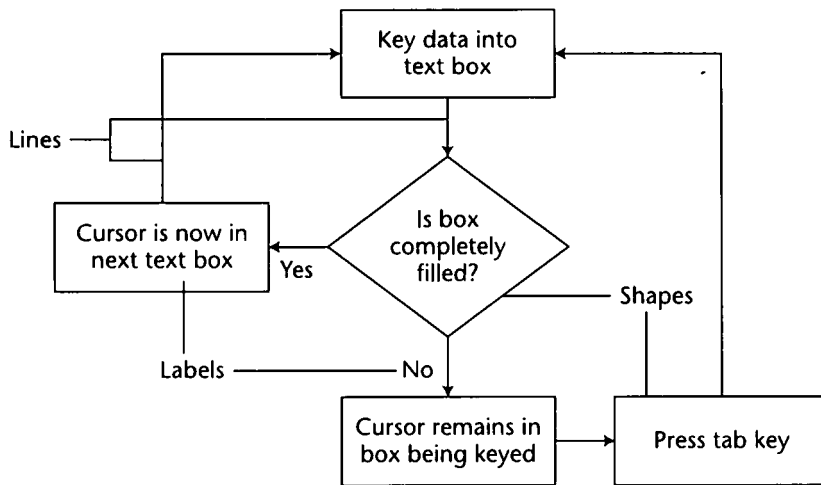
Figure 11.8: Diagram elements.
