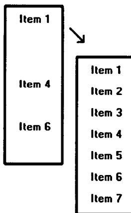
Figure 4.11: Temporal menu.
