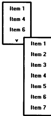
Figure 4.10: Folded menu.
