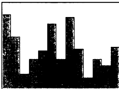
Figure 3.81: A histogram or step chart.
