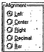
Figure 7.25: Radio buttons.
