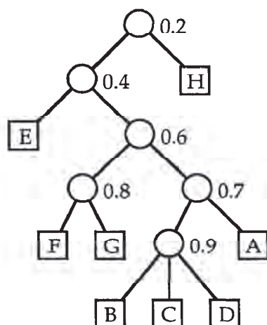
Fig. 1 A sample single link hierarchy
