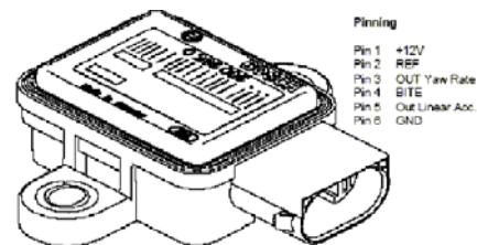
Figure 9; Bosch's gyroscope package with integral connector and mounting brackets
