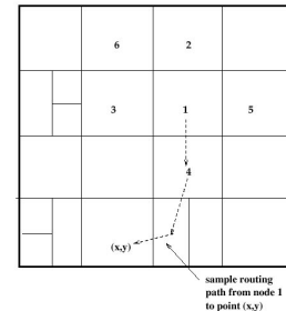
Fig. 6. Example 2-d space
