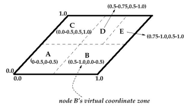
Fig. 5. Example 2-d coordinate overlay with 5 nodes
