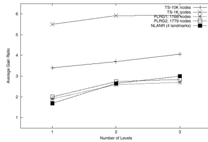
Fig. 2. Effect of number of levels (#landmarks = 12)
