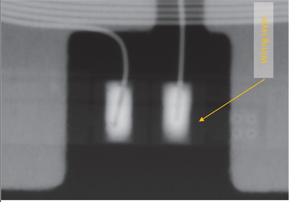
X-ray of the wireless power receiver from the exemplary Apple AirPods Pro showing a wiring layer connected to the third connection terminal and the fourth terminal.
