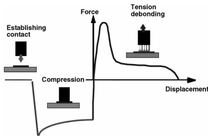
Figure 1. Schematic illustration of a tack test performed with a cylindrical, flat-ended probe.
