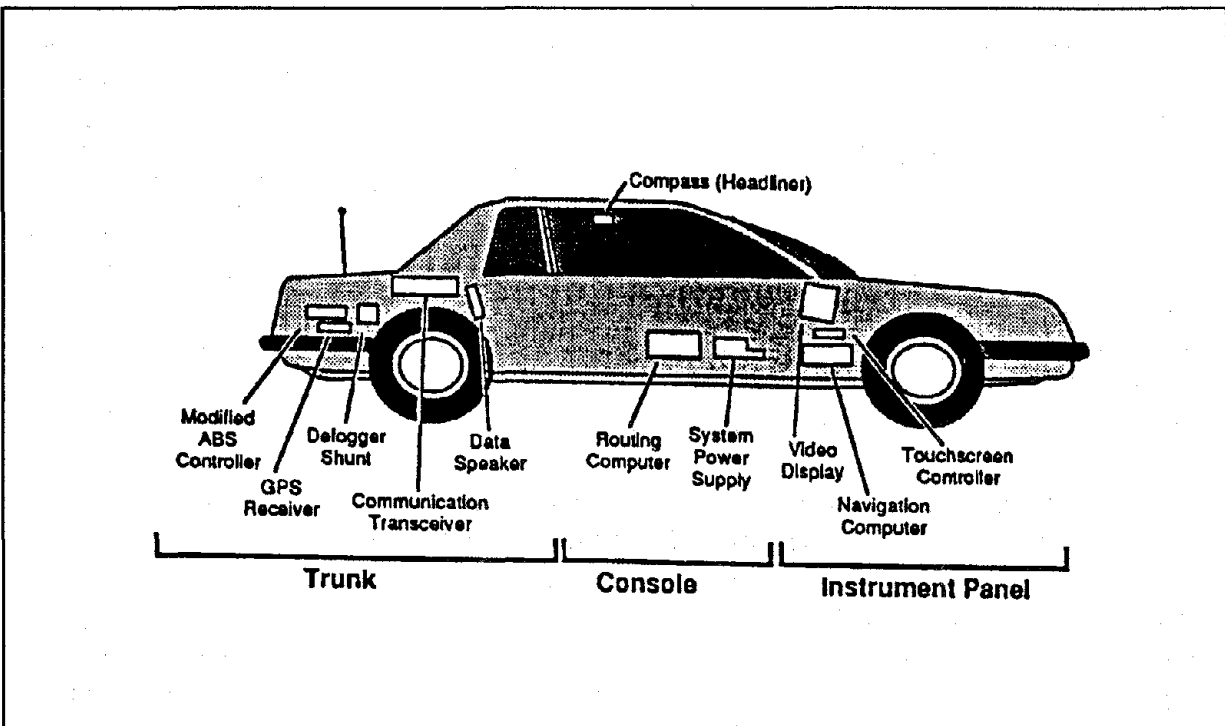
Figure 28. Layout of the TravTek equipment in the vehicle. (11)
