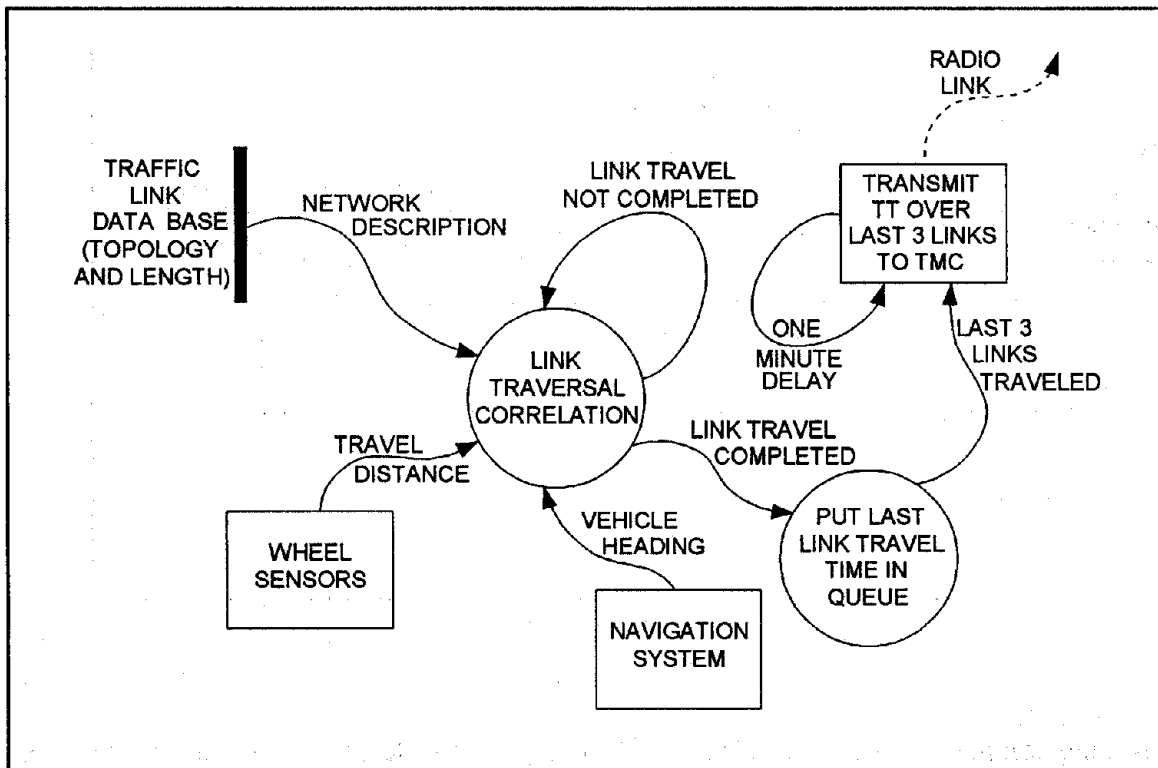
Figure 42. Probe report data flow.
