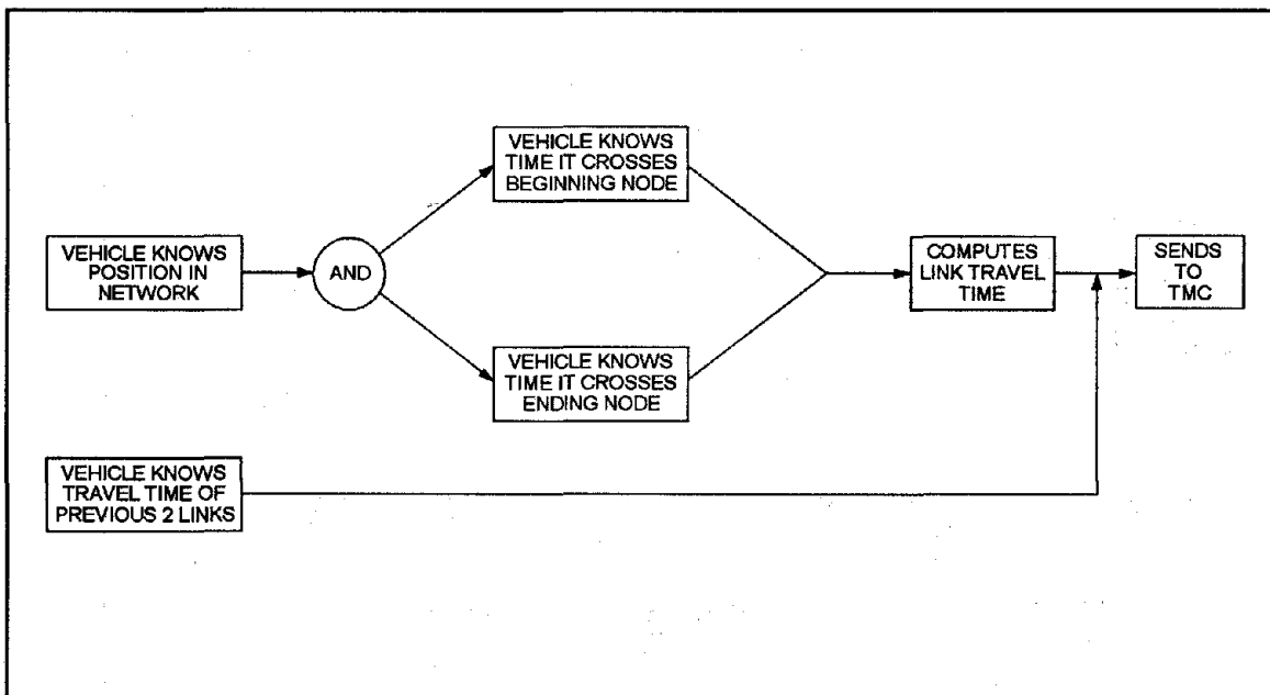
Figure 41. Vehicle probe function.
