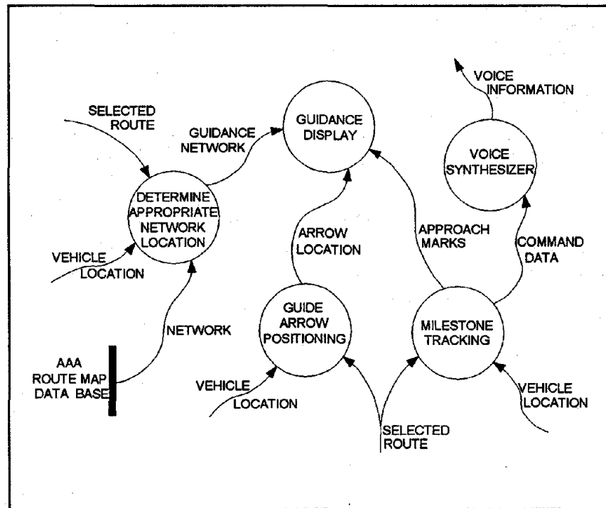
Figure 36. Route guidance data flow.
