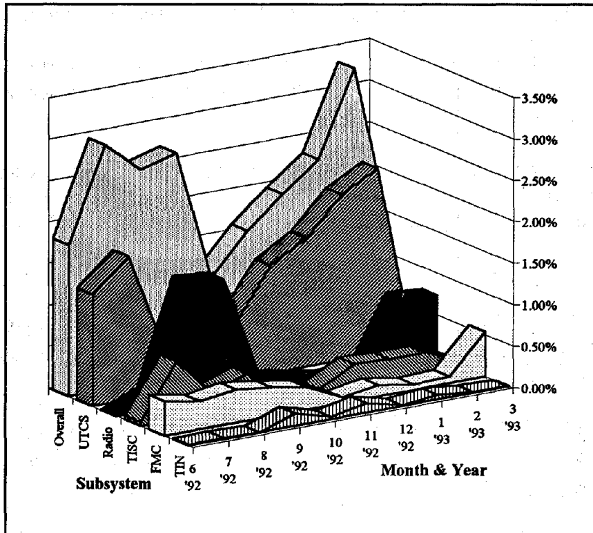
Figure 121. Percent downtime by subsystem by month.
