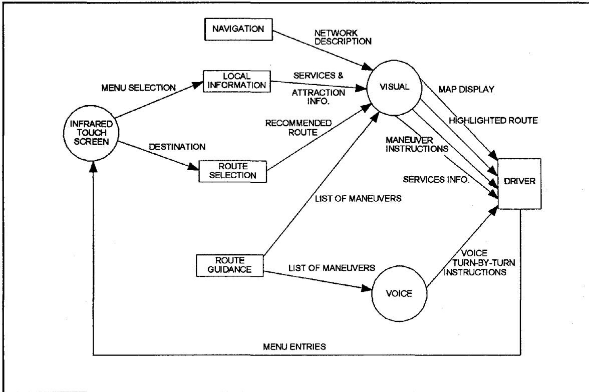
Figure 40. Data flow diagram for driver interface function.
