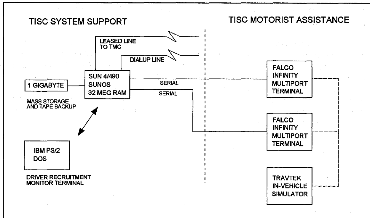
Figure 13. TISC system configuration.
