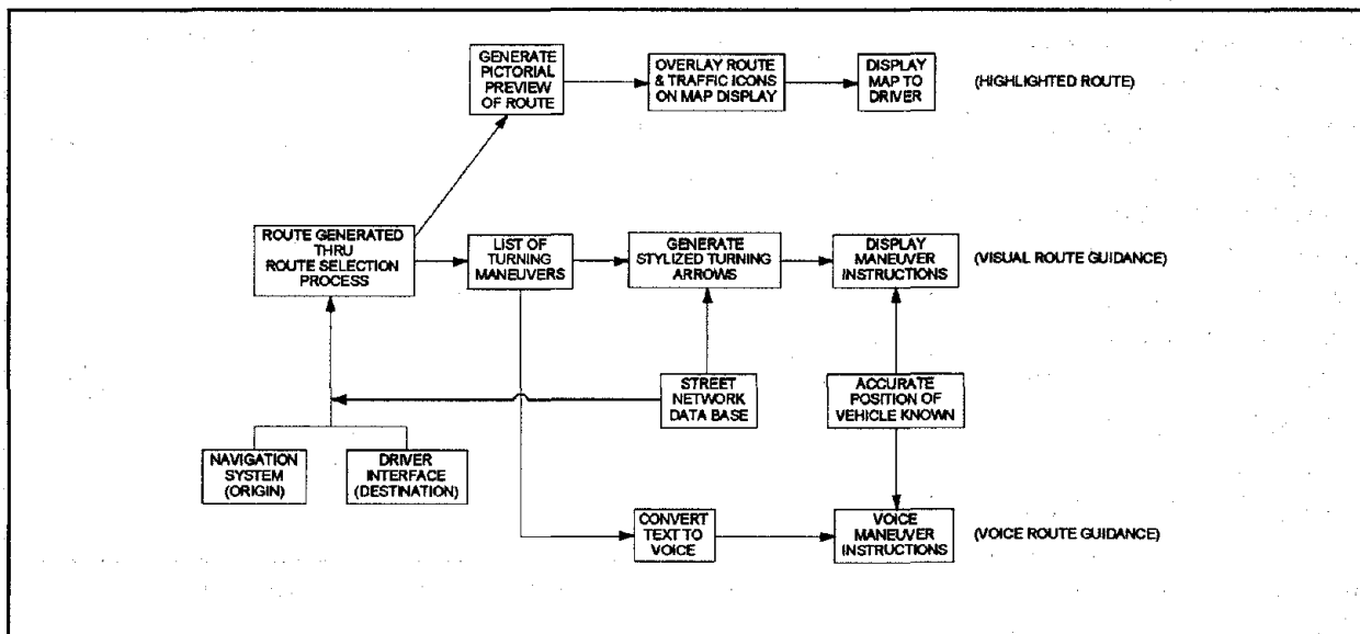
Figure 35. Route guidance functional diagram.
