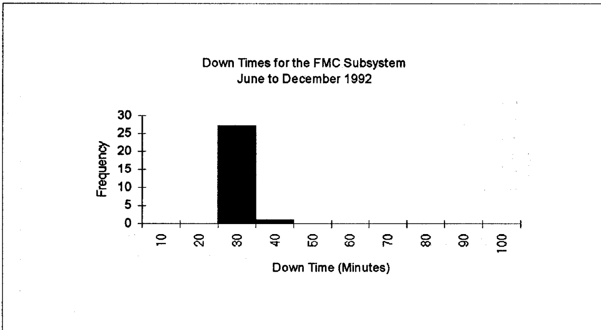
Figure 81. Down times for the FMC subsystem, 6/92 - 12/92.
