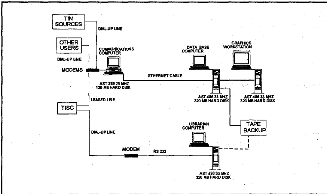
Figure 15. TMC computer configuration. (1)
