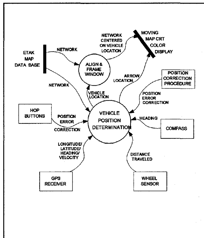
Figure 31. Vehicle navigation data flow.
