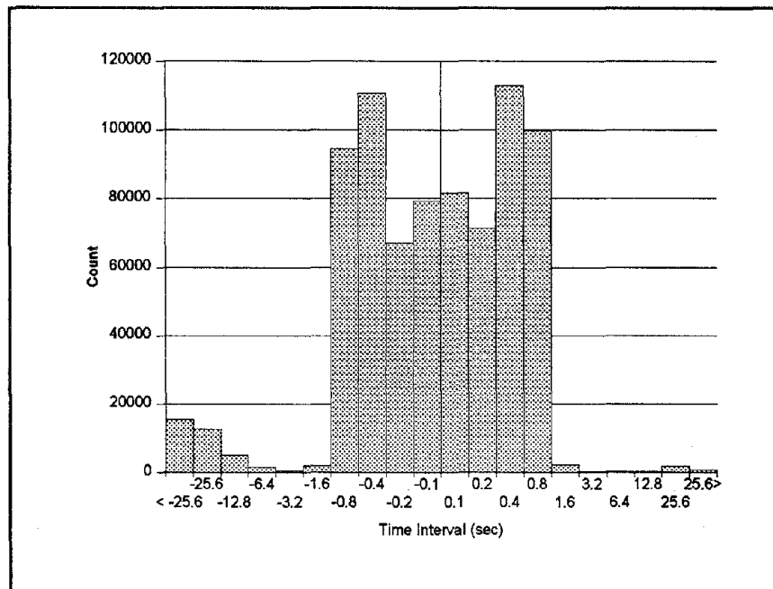
Figure 126. Vehicle transmit time slot accuracy.
