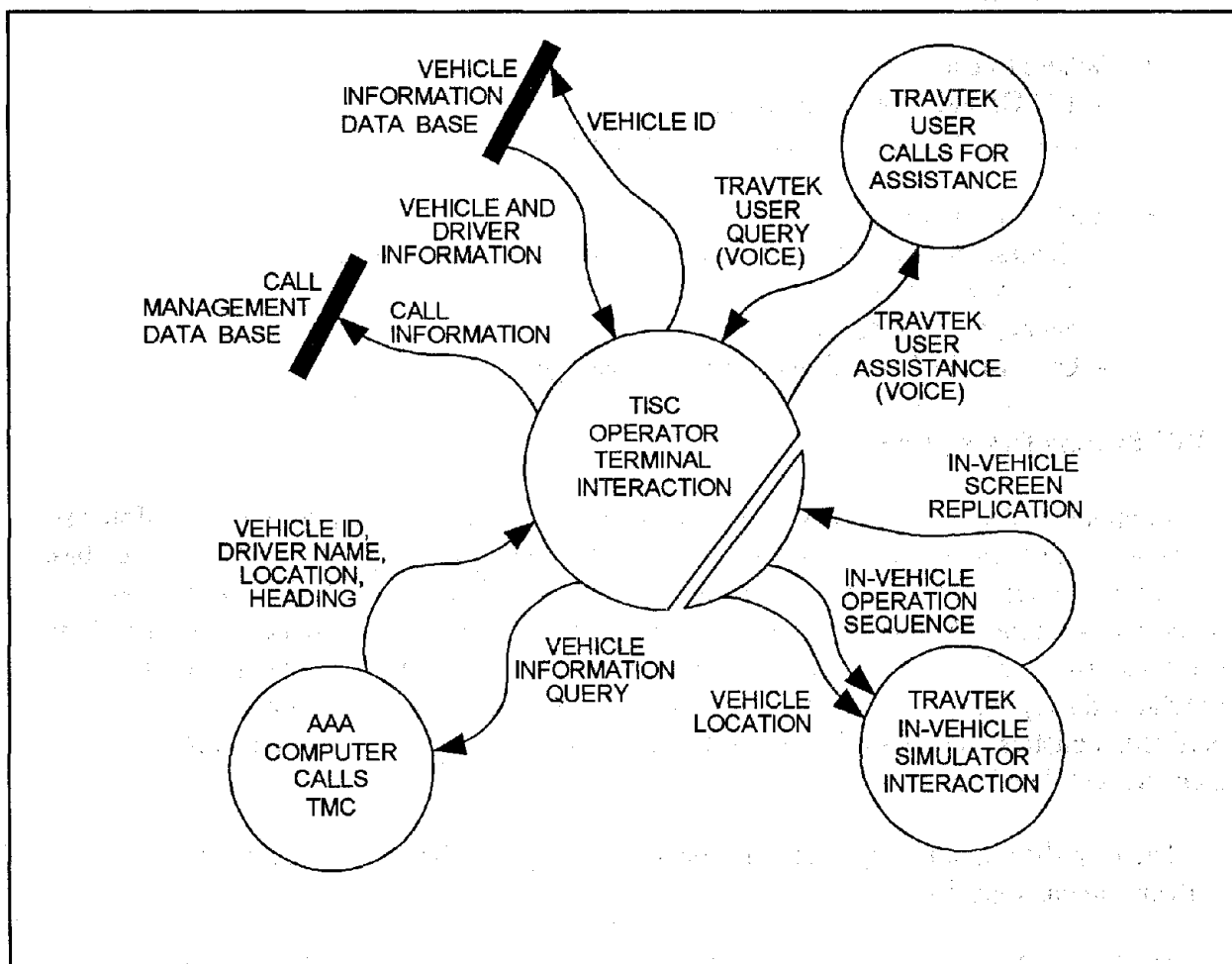
Figure 14. TISC help desk information flow.
