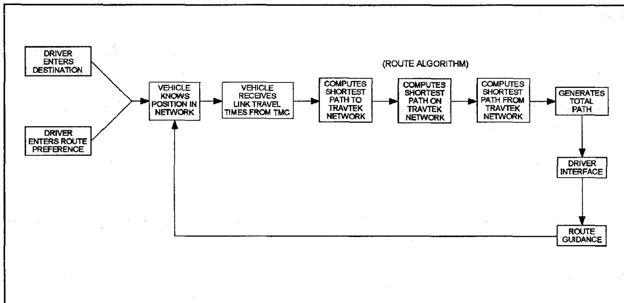
Figure 32. Vehicle route planning/route selection function.
