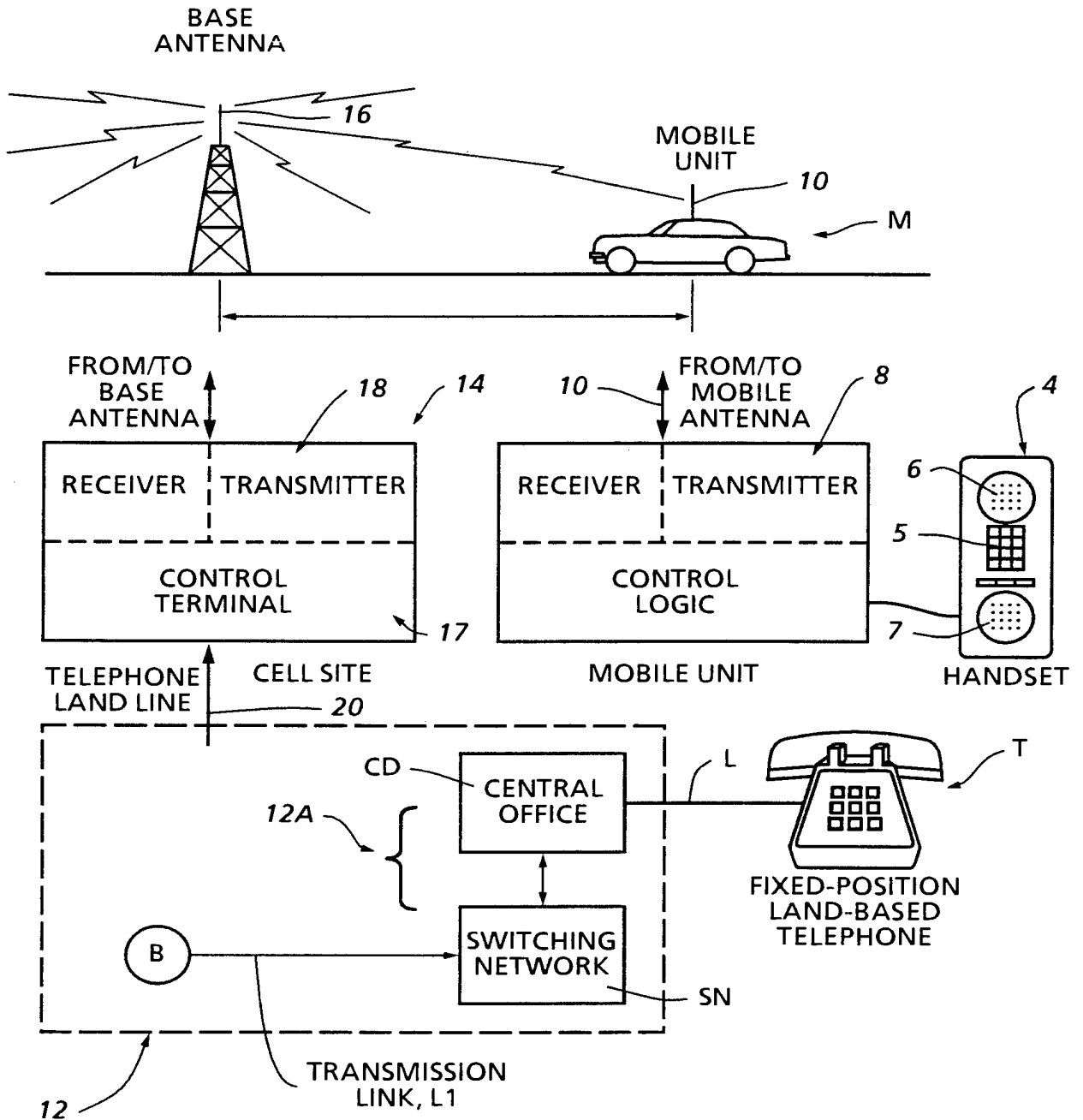
FIG. 4 (PRIOR ART)
