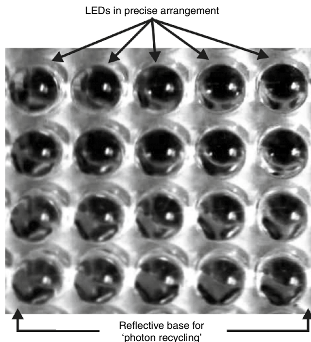
Fig. 3 Close-up view of dome-type LEDs mounted in an actual array from a therapeutic system. Note the precise x-y spacing of the LEDs, ( cf Fig. 6 and associated text), and the reflective backing into which they are mounted. When light is incident on living skin, a certain amount will be reflected from the outer layer of skin, the stratum corneum. The longer the wavelength, the greater this reflection will be. In addition, some light is always back-scattered out of skin. The purpose of the reflective backing of the array is to capture these photons and reflect them back into the skin, known as 'photon recycling'
