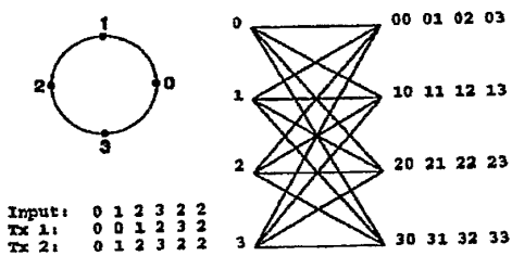
4-PSK 4-State Space-Time Code with 2 Tx Antennas
