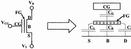
Fig. 9.10. Floating gate NMOS coupling capacitors
