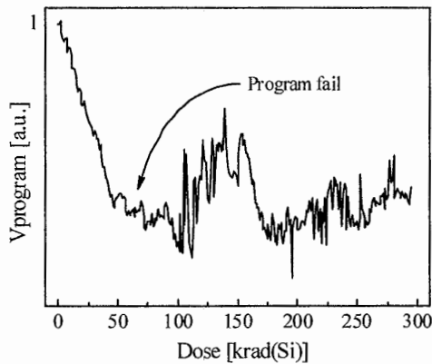
Fig. 19.8. Average voltage generated by the program charge pump during TID exposure (normalized to V_{\text{program}} before irradiation) 43 © IEEE, 2009
