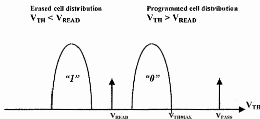
Fig. 8.2. Threshold voltage distributions for erased and programmed cells
