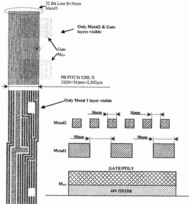
Fig. 8.21. 36 nm technology node: BL and BLINT layout in BLSEL circuitry
