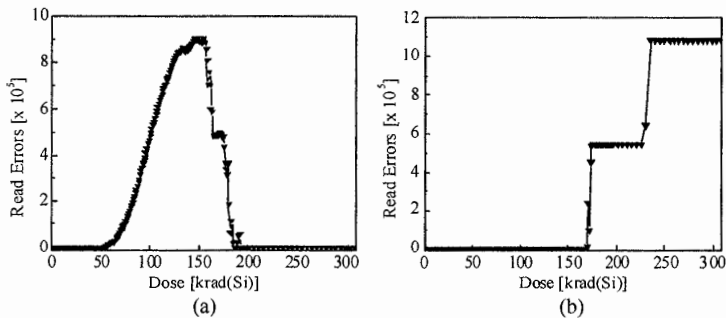
Fig. 19.9. Number of read errors during x-ray exposure of FG array and row decoder as a function of x-ray dose, for a block that was programmed (a) and a block that was erased (b) prior to irradiation 43 © IEEE, 2009
