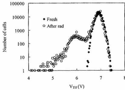
Fig. 19.19. Probability density of threshold voltages before and after irradiation with 2 \times 10^7 iodine ions/cm 2 [59] © IEEE, 2001
