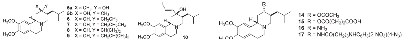
Figure 4. Structures of tetrabenazine analogs ( 5a-b and 6-10 ).
