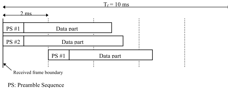
Figure 21 Possible transmission timing for parallel Random-Access attempts
