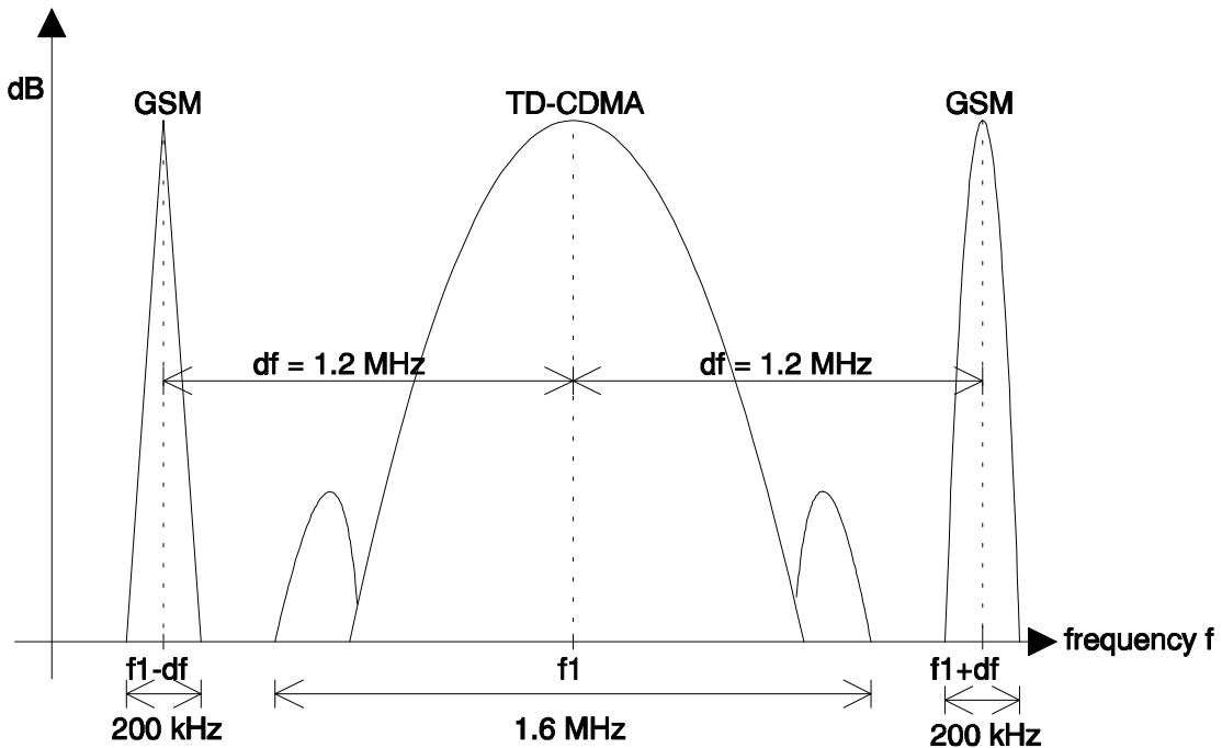
Figure 2-1 WB-TDMA/CDMA and GSM900/1800 carriers use adjacent channels
