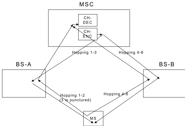
Figure 22 MSC handover
