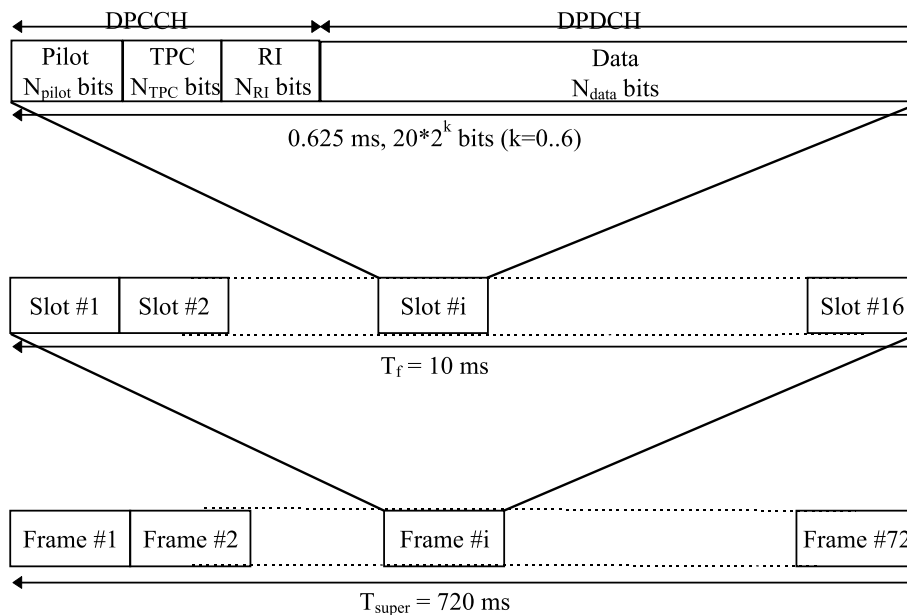
Figure 2 Frame structure for downlink dedicated physical channels.
