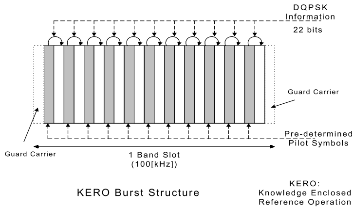
Figure 2: KERO burst structure
