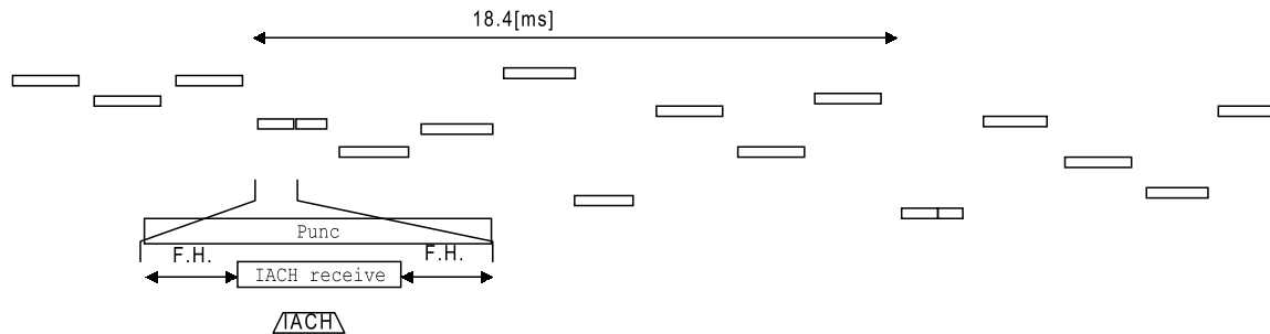
Figure 19 Puncturing Scheme (1 of 4 Time slot usage)
