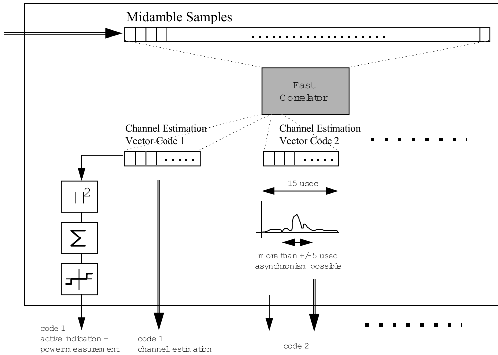
Figure 23 WB-TDMA/CDMA Channel Estimator Function
