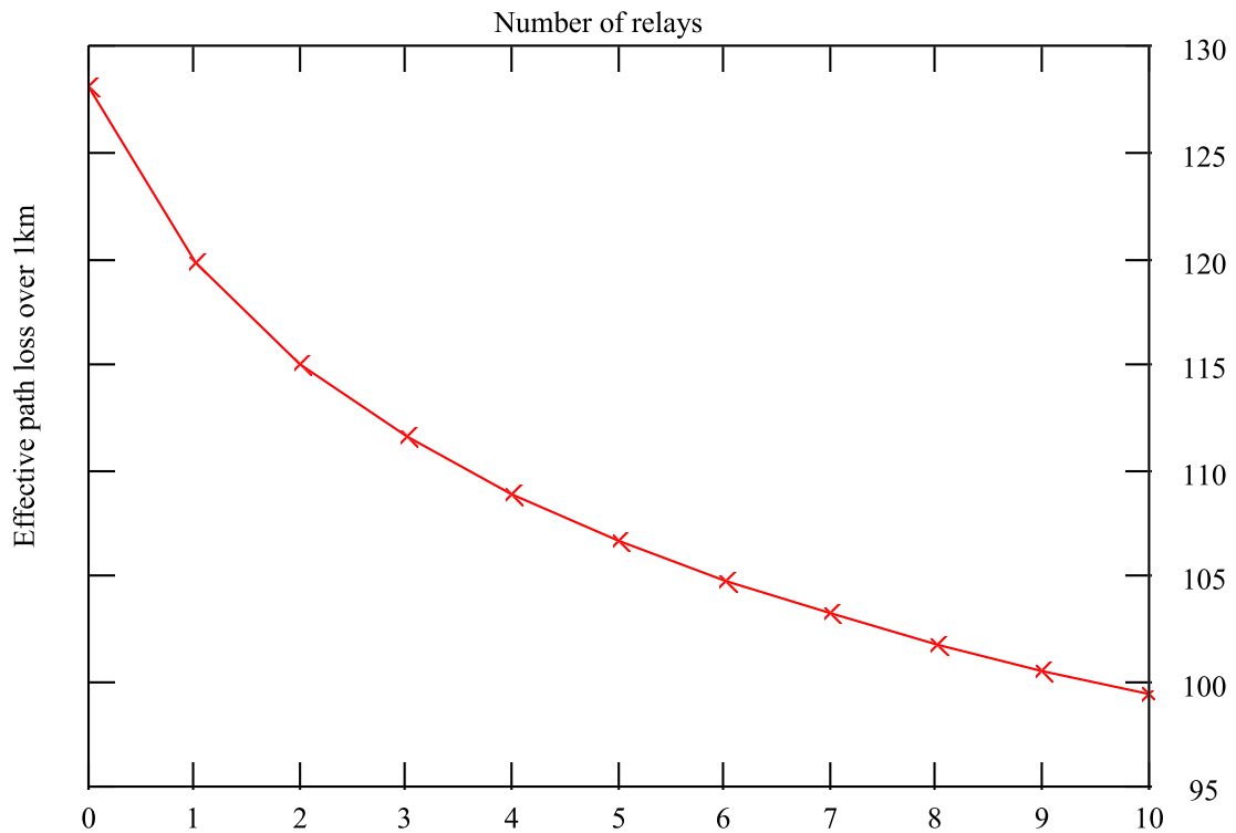
Figure 3 Effective Pathloss v Number of Relays
