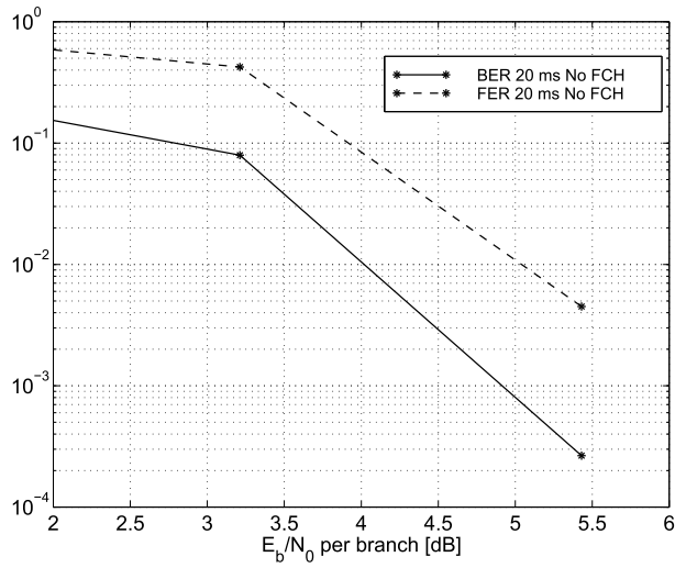
Figure 7. Speech, Vehicular B 120 km/h, with antenna diversity.
