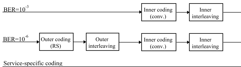
Figure 10 Basic FEC coding for WCDMA
