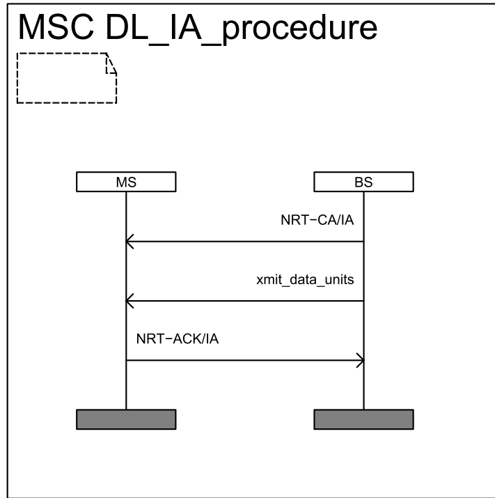
Figure 4-7. Downlink Immediate Allocation transmission
