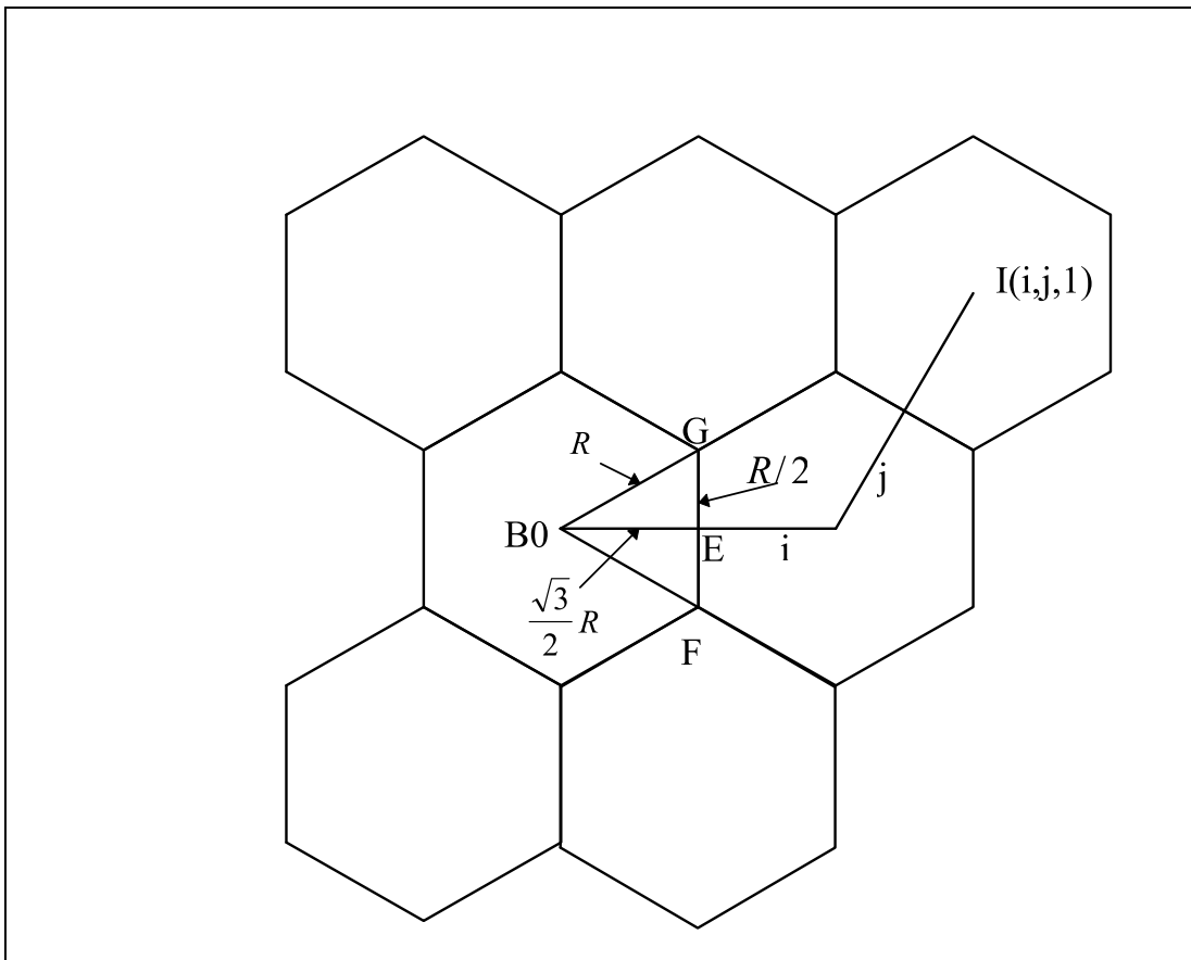
Figure 7: Geometry of interferers
