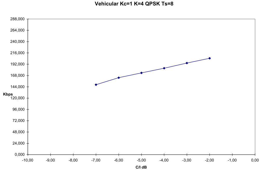
Figure 1-18 UDD 144 kbit/s UL Vehicular 120 km/h, 4 Users per TS, 1 Code and 8 TS per user, QPSK, code rates 1, 2/3, 1/2, 1/3 and 1/4
