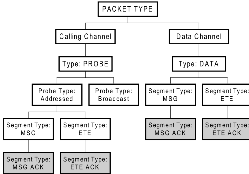
Figure 12 ODMA Packet Structures
