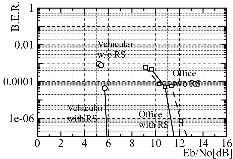
Figure 29: Eb/No vs BER (LCD384)
