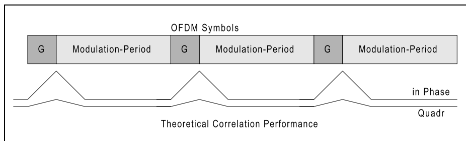
Figure 15: Theoretical Time Synchronisation Performance (Correlation)
