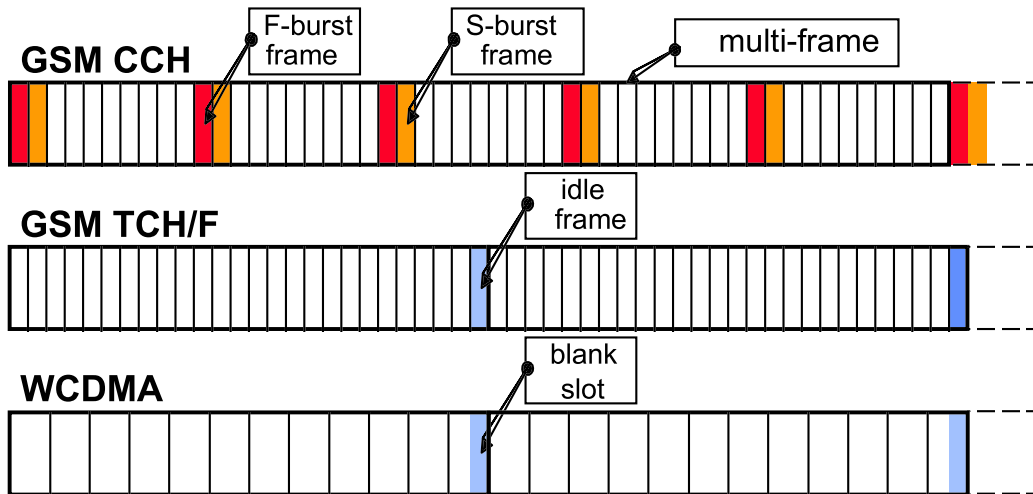
Figure 27. GSM measurement timing from WCDMA operation mode.
