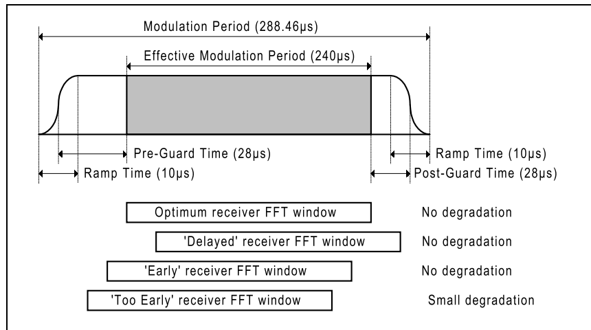
Figure 17: OFDMA burst and synchronisation requirements
