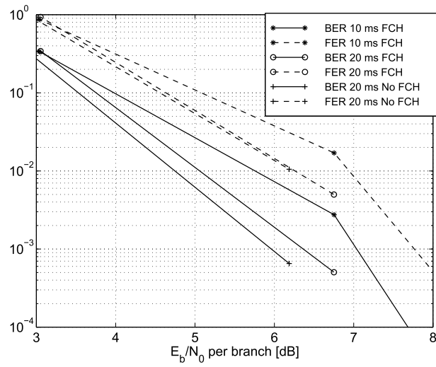
Figure 9. Speech, Vehicular B 250 km/h, with antenna diversity.
