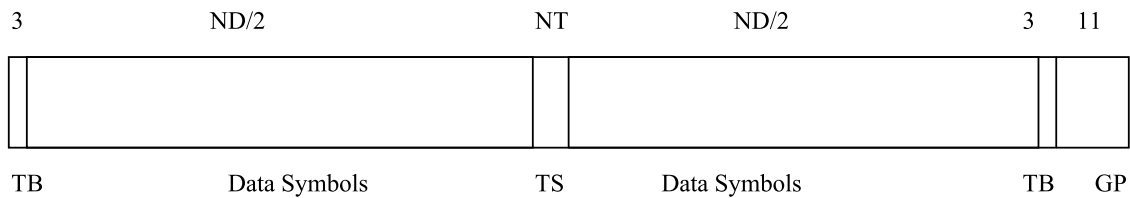
Figure 3-9 Structure of Flexible Burst
