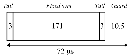
Figure 3-12 The Frequency correction burst.
