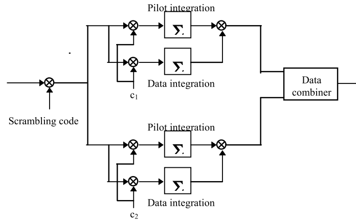
Figure 37 Rake finger processing with OTD
