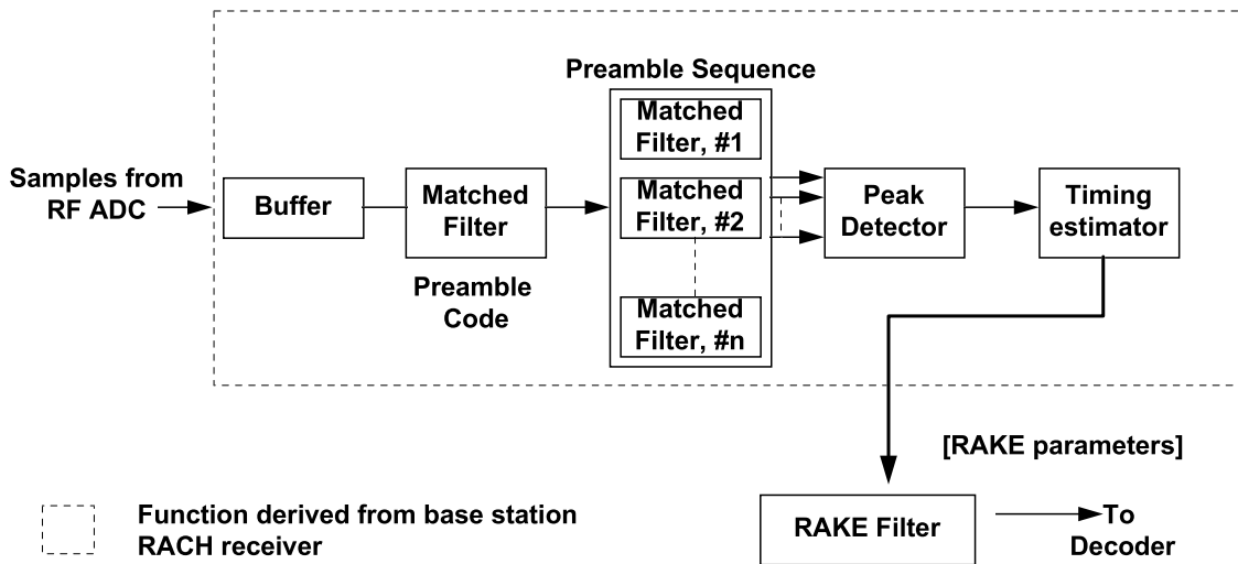
Figure 22 Synchronisation Function
