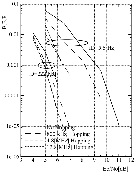
Figure 4: BER versus E_b/N_0
