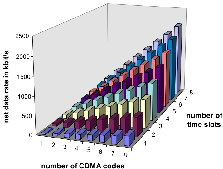
Figure 3: Flexibility of data rates in WB-TDMA/CDMA
