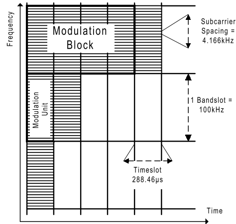
Figure 5: Time and frequency grid
