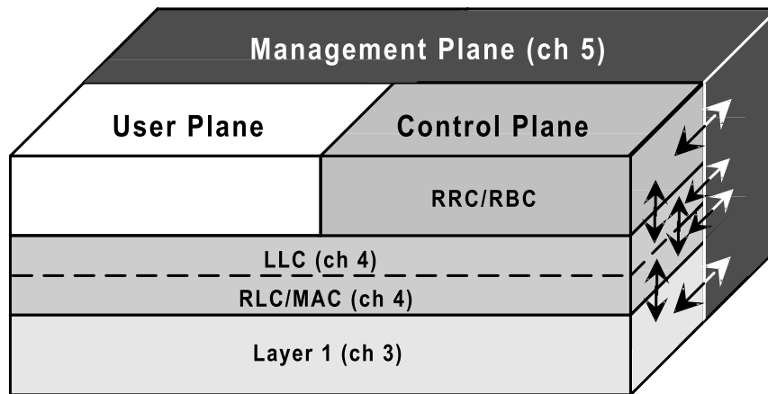
Figure 1-1 The Layered Structure of WB-TDMA Radio Interface
