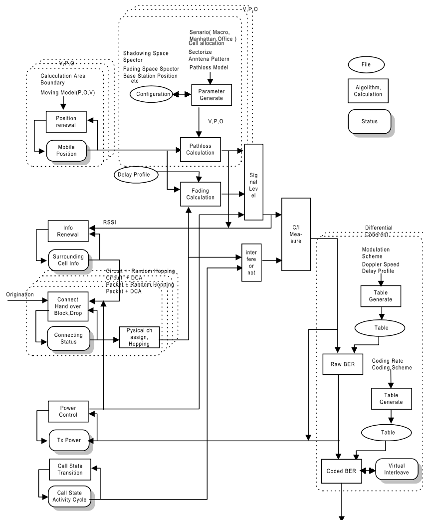
Figure 40: Structure of System Level Simulation
