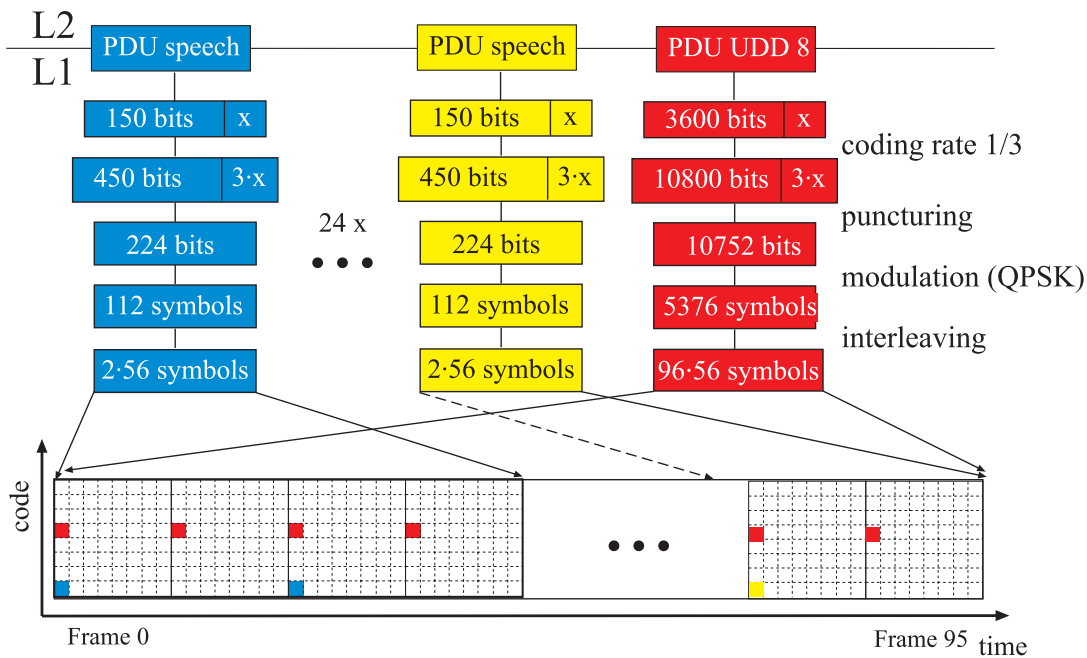
Figure 3.6 50% speech + 50% UDD 8 (long UDD 8 packets)
