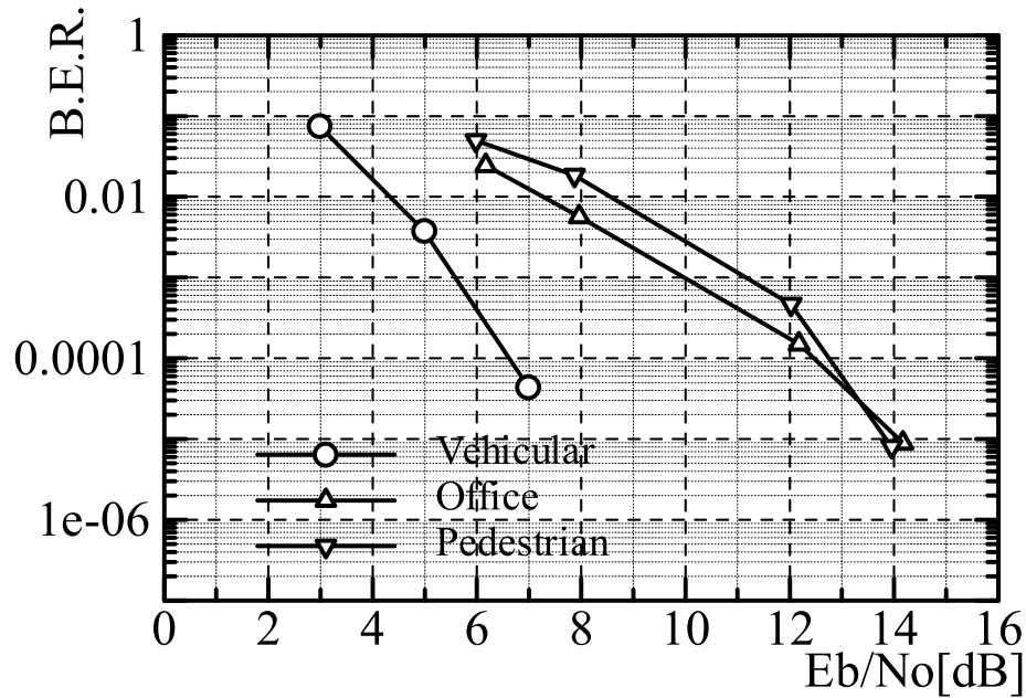
Figure 27: Eb/No vs BER (SPEECH)
