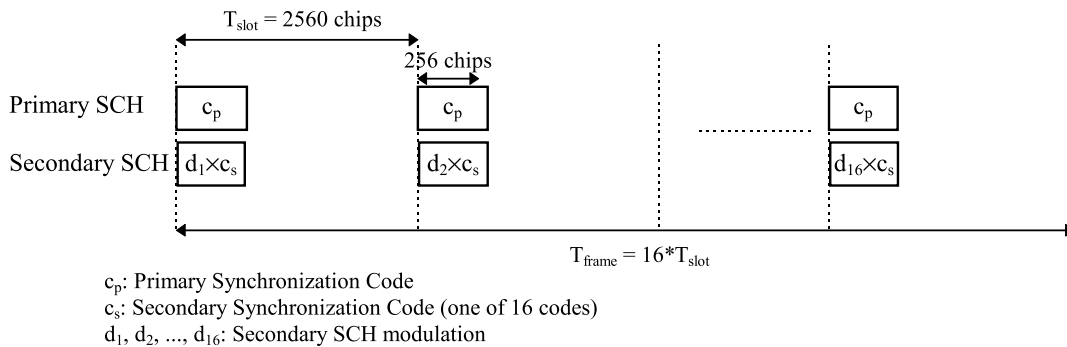
Figure 8 Structure of Synchronisation Channel (SCH)
