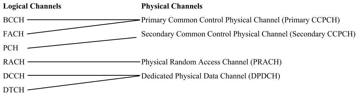
Figure 1 Logical-channel to physical-channel mapping
