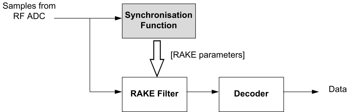
Figure 21 WCDMA Receiver
