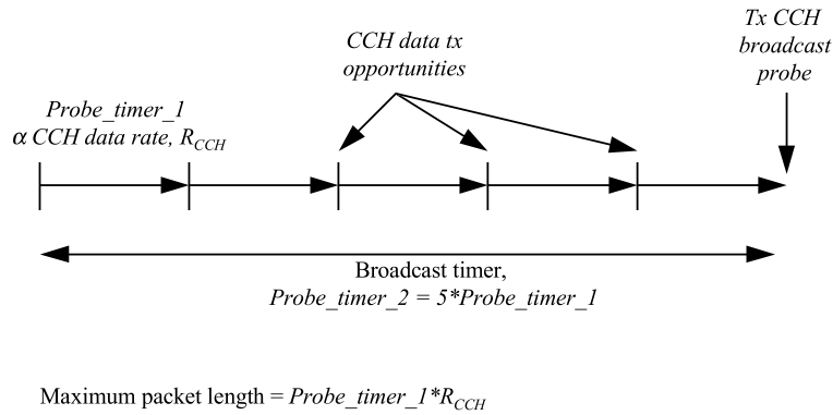
Figure 11. CCH Timer Relationships.
