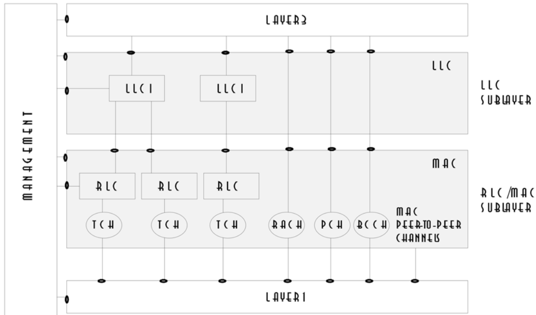
Figure 4-2. Layer 2 internal structure
