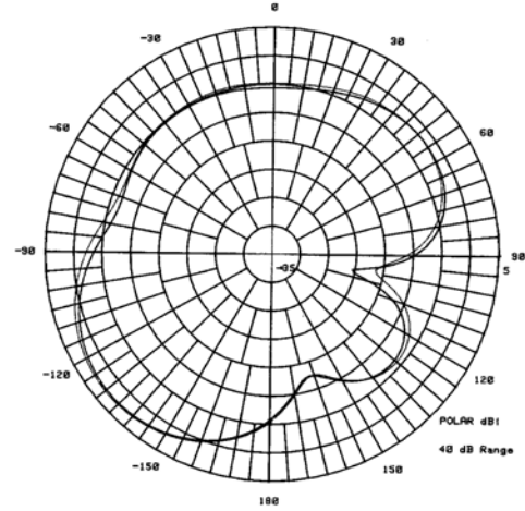
Figure 7: Antenna Pattern (Patch)
