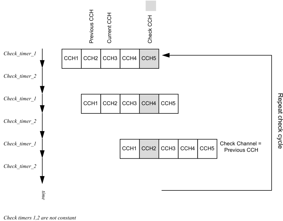
Figure 11. Check channel cycle.
