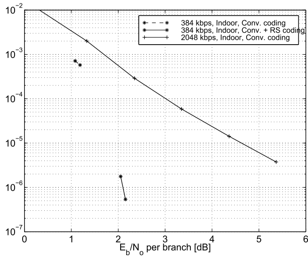
Figure 12. LCD 2048, with antenna diversity.
