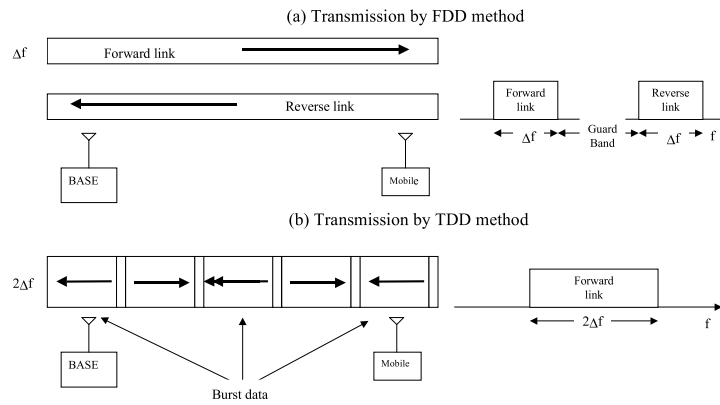
Figure 32 Principle for FDD and TDD operation
