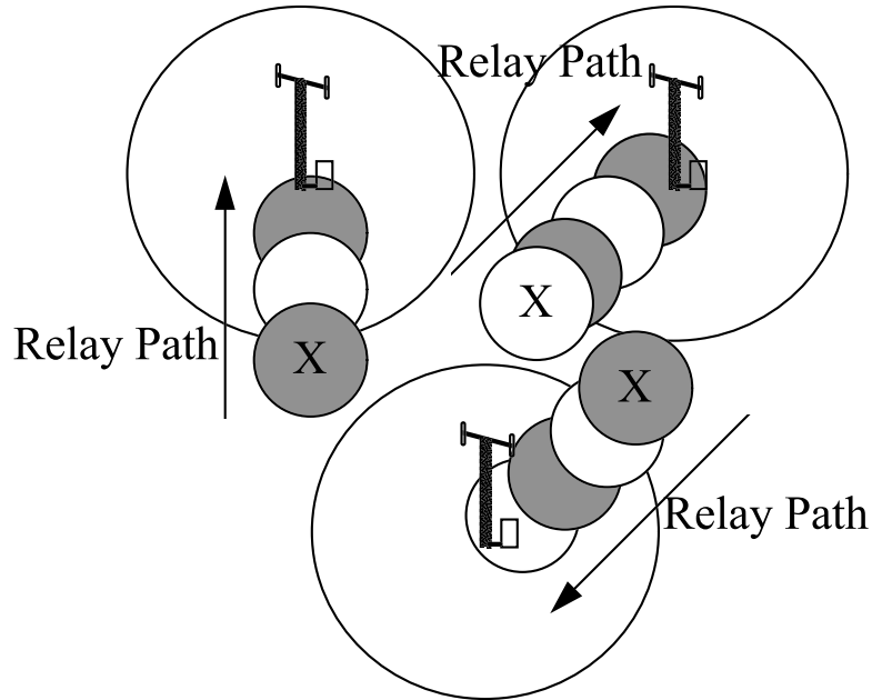
Figure 7 Discontinuous Cell Coverage
