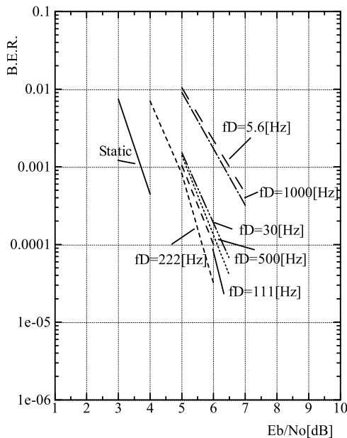
Figure 1: B.E.R. versus speed (doppler) for speech service
