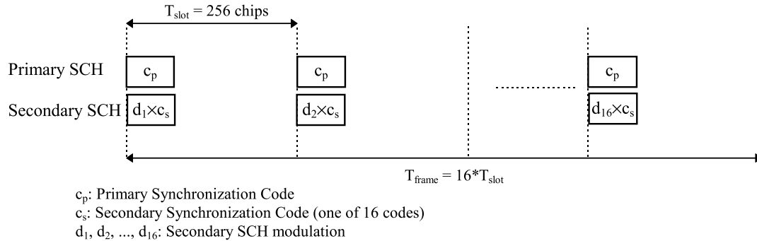
Figure 23 Structure of synchronization channel (SCH)
