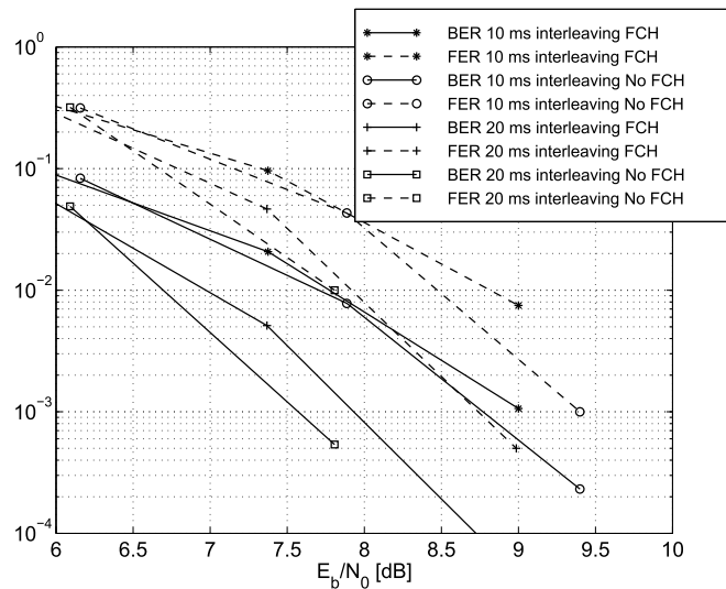
Figure 6. Speech, Vehicular A 120 km/h, without antenna diversity.
