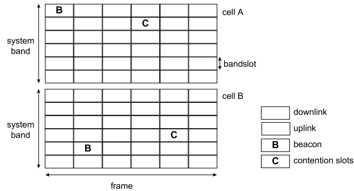
Figure 25: Example of Frame Layout
