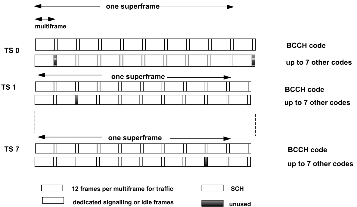
Figure 3-1: Mapping of the SCH channel
