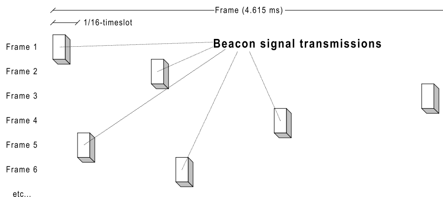
Figure 2-2 An example about beacon signal.
