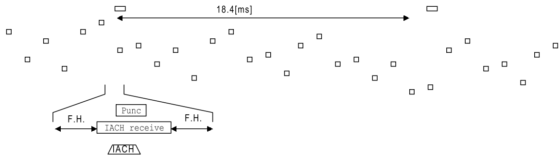
Figure 12 Puncturing Scheme ( 1 of 4 time slot usage )
