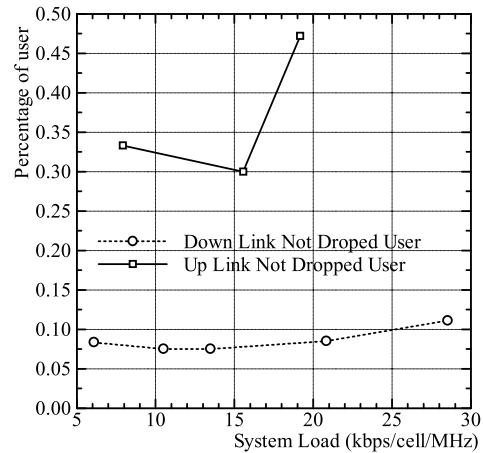
Figure 52: Not Dropped User Rate
