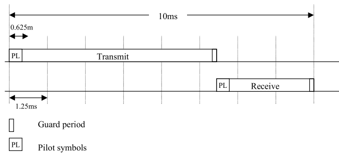
Figure 36 Suggested Rx/Tx cycle for unlicensed private use.
