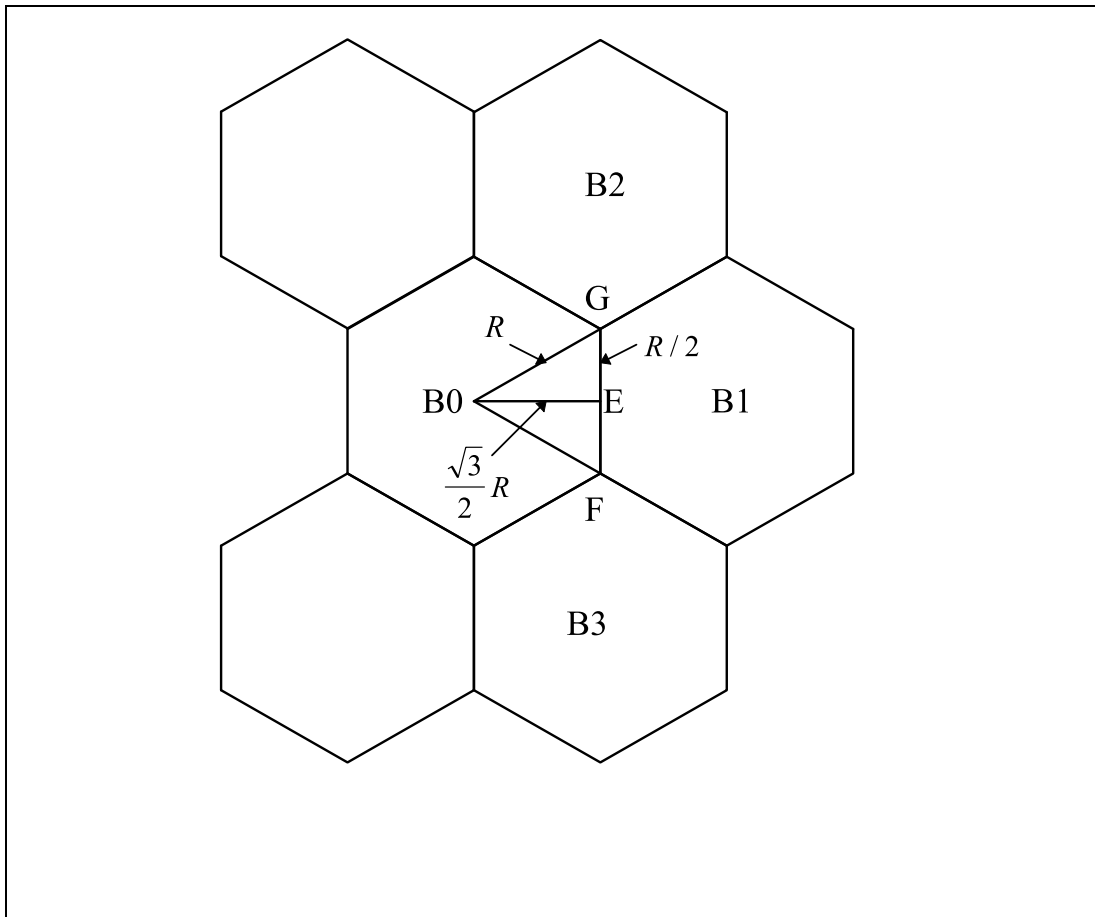
Figure 8: Geometry of handover to adjacent cells
