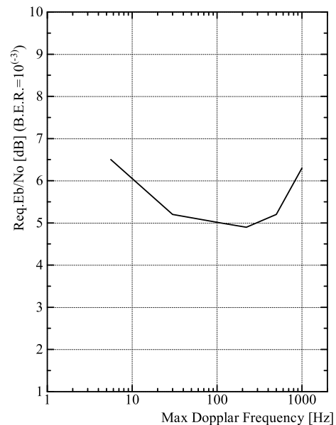
Figure 2: Required E_b/N_0 versus speed (doppler frequency)
