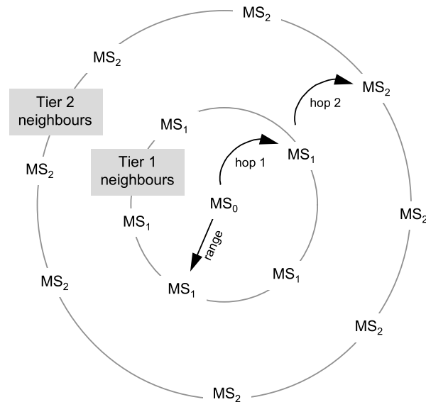
Figure 15. Localised connectivity through probing.
