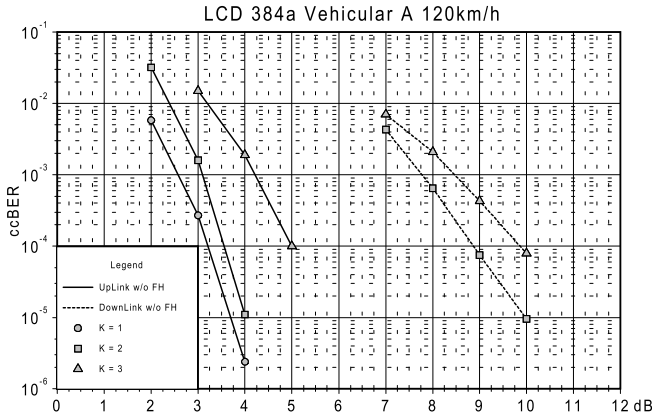
Figure 1-10 LCD 384 a UL and DL Vehicular 120 km/h, 1, 2 and 3 Users per TS, 3 Codes and 8 TS per user
