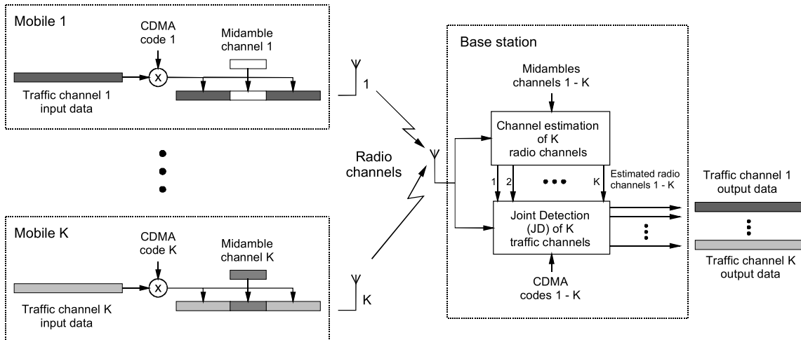
Figure 2: Uplink of WB-TDMA/CDMA
