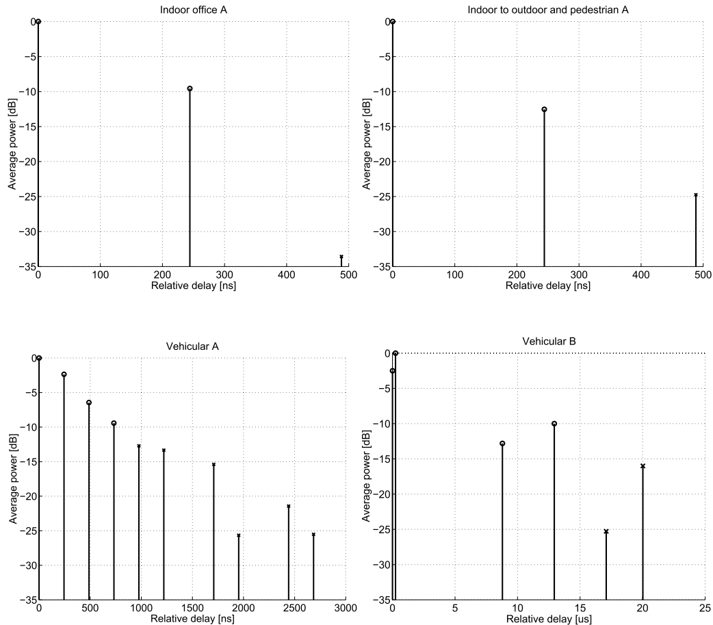
Figure 38. Modified channel models used in the simulations.
