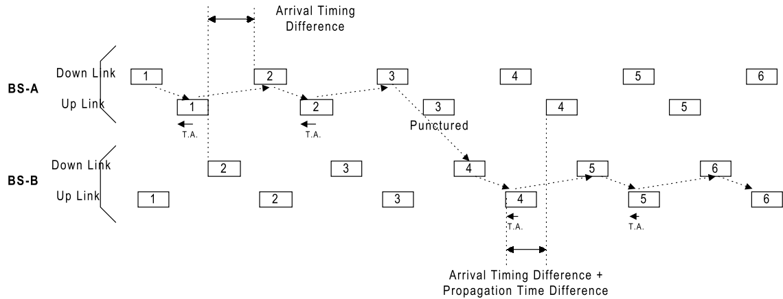
Figure 21 MSC Puncturing Scheme
