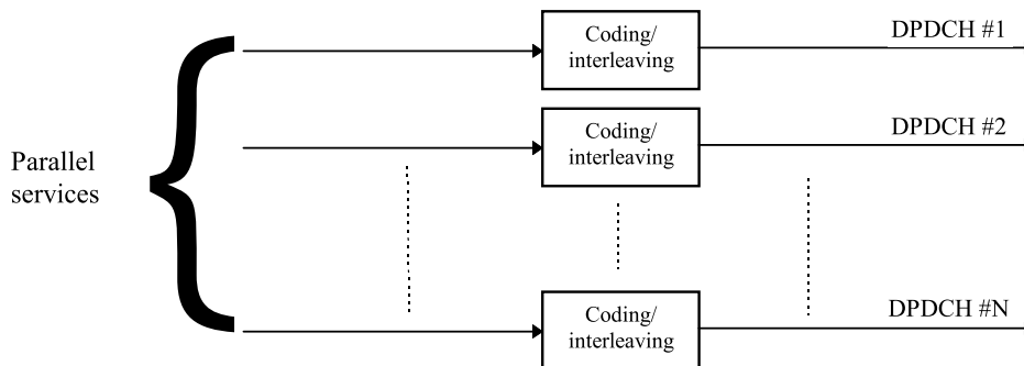
Figure 12 Alternative service multiplexing
