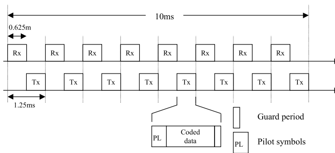
Figure 35 Suggested Rx/Tx cycle for cellular public applications
