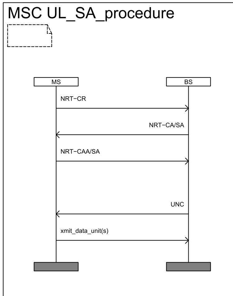
Figure 4-6. Uplink Scheduled Allocation transmission
