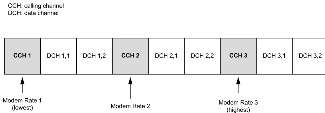
Figure 10. Logical Channels in ODMA.
