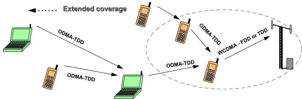
Figure 1 Scenario for WCDMA with ODMA enhancement
