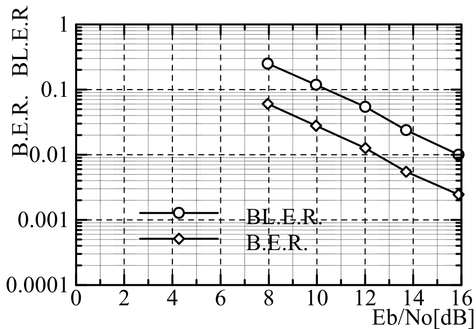
Figure 36 Eb/No vs B.L.E.R. ( UUD2048, Office )
