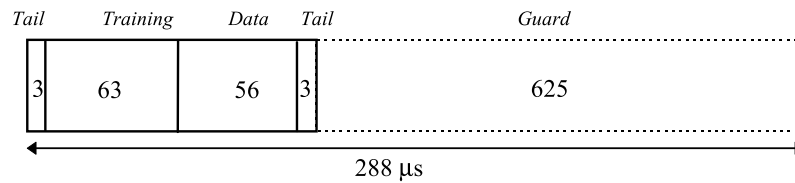
Figure 3-15 The 1/16-slot Access burst.
