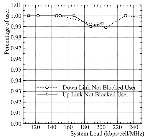
Figure 54: Not blocked User Rate
