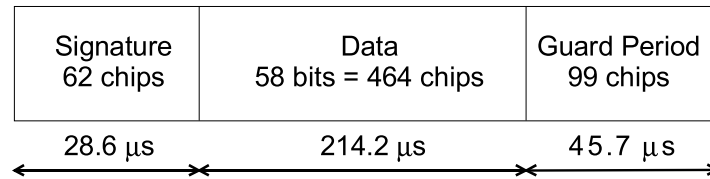
Figure 1 : Short access burst
