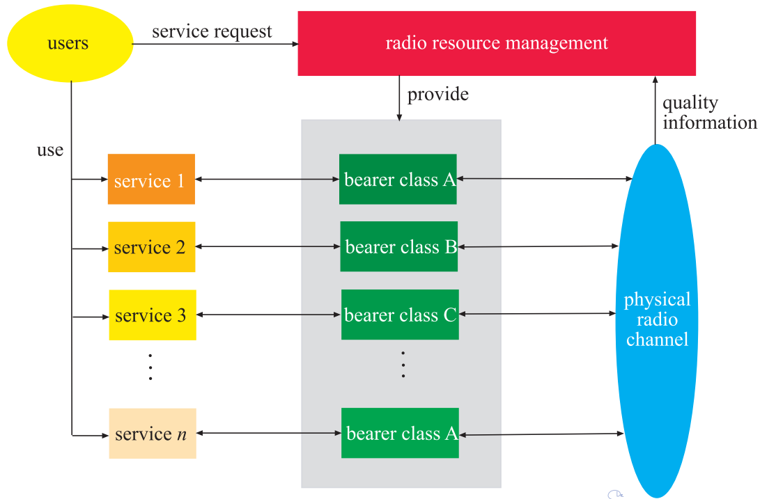
Figure 2.2 Generic radio resource allocation for ASD
