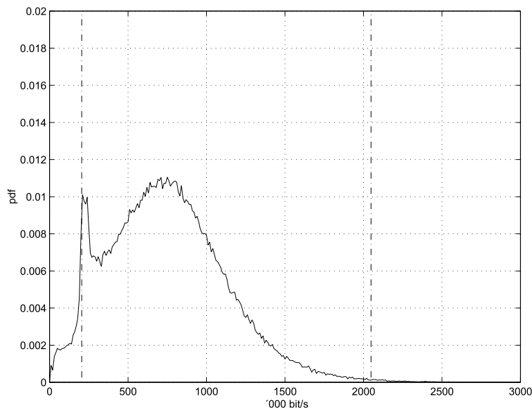
Figure 5. Histogram for session throughputs.
