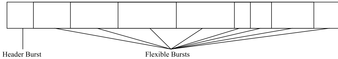
Figure 3-8 Multiplexed burst
