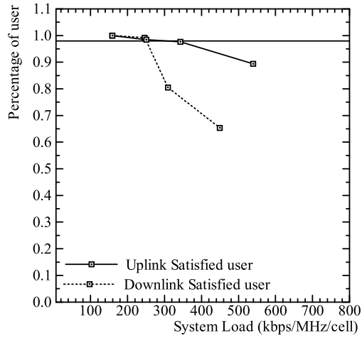
Figure 56 System Bandwidth 15 MHz
