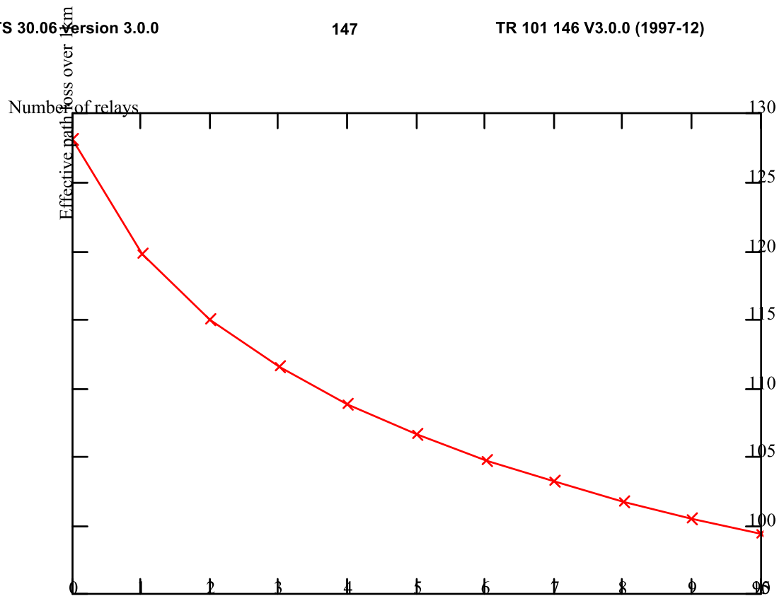
Figure 2 Effective Pathloss v Number of Relays
