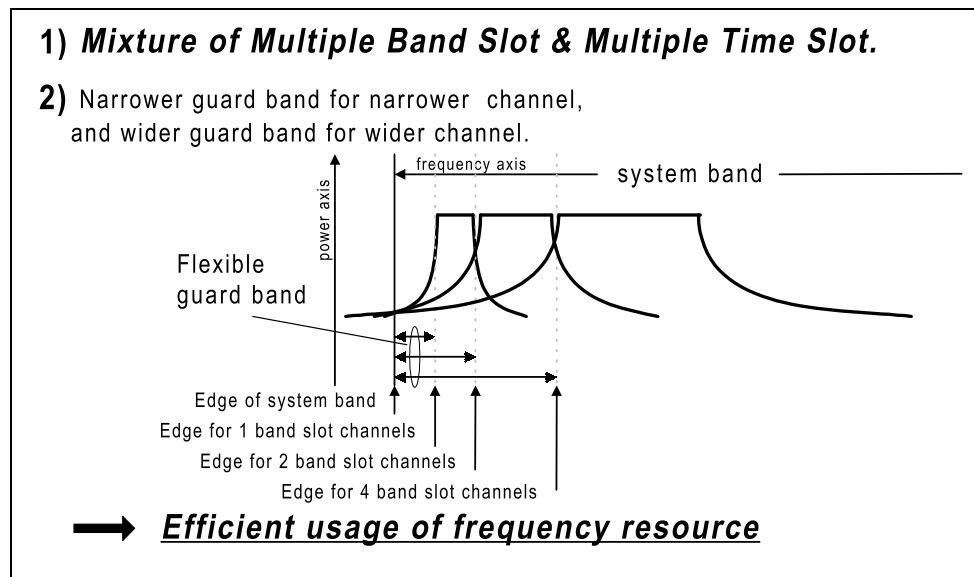
Figure 26: Flexible OFDMA Structure
