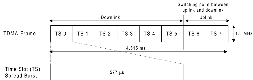
Figure 4-3 The unit TDD frame structure of WB-TDMA/CDMA.
