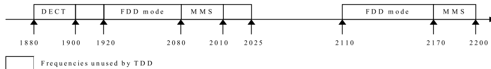
Figure 33 Spectrum allocation for UMTS
