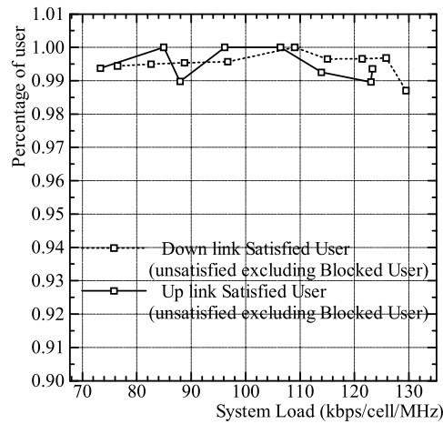
Figure 44: System Bandwidth 15MHz
