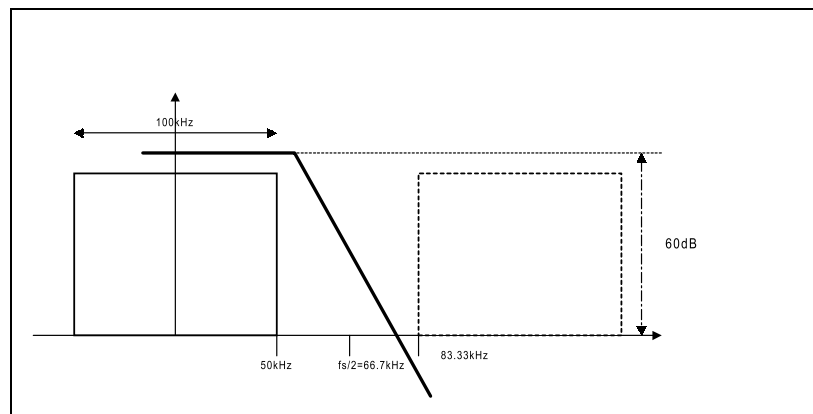
Figure 15: OFDMA filter requirements
