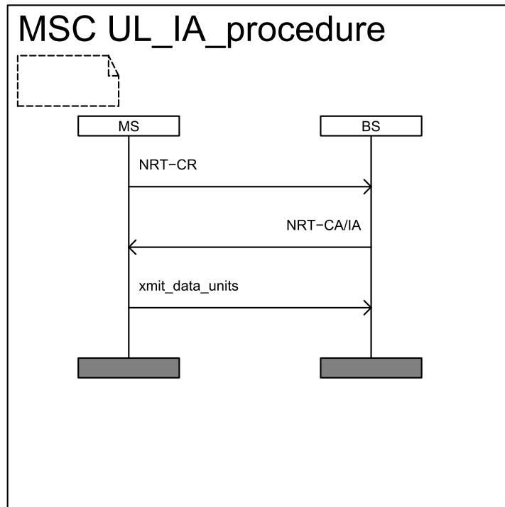
Figure 4-8. Uplink Immediate Allocation transmission
