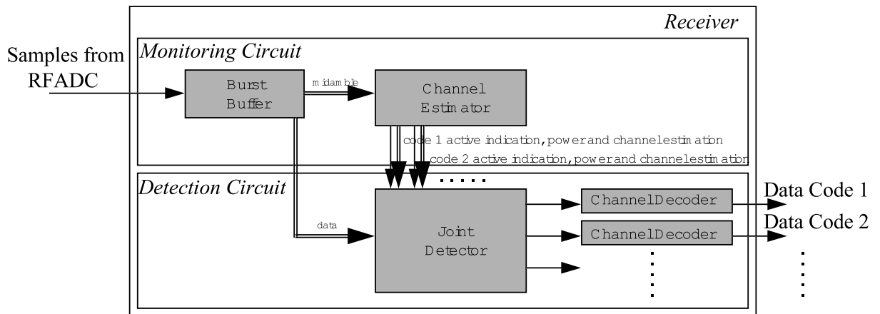
Figure 22 WB-TDMA/CDMA - ODMA Enabled Receiver
