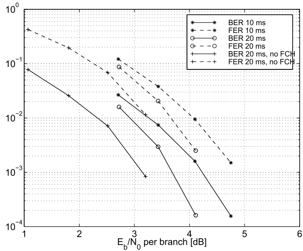
Figure 1. Speech, Indoor office A, with antenna diversity.
