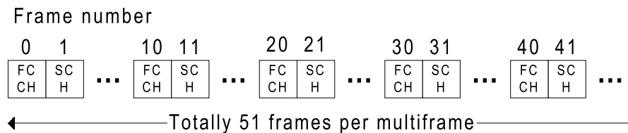
Figure 2-1 GSM multiframe for BCCH-timeslot
