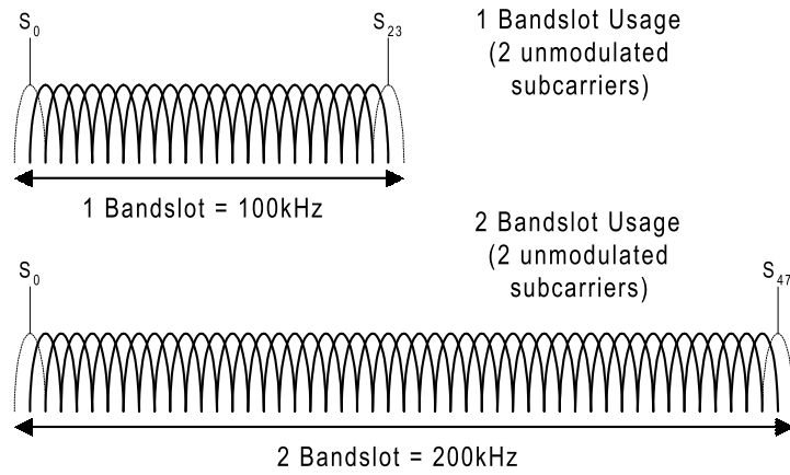
Figure 9 : Guard Carrier Allocation
