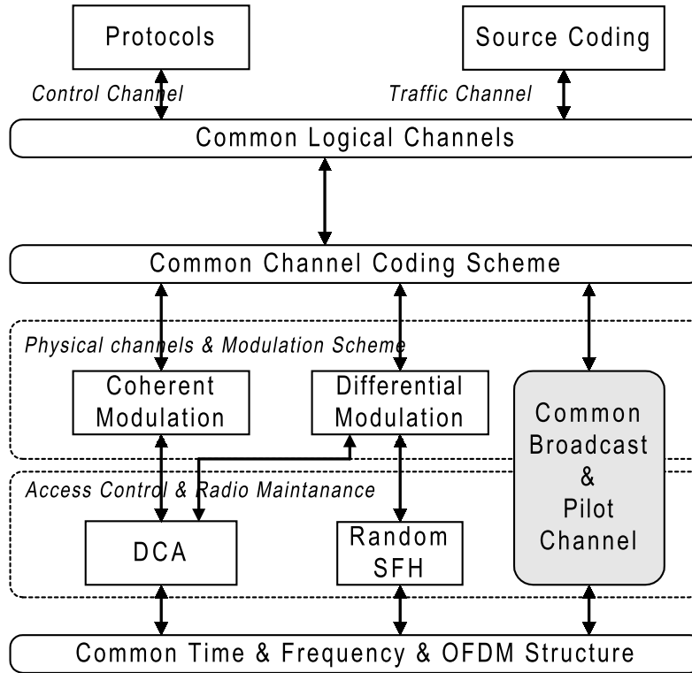
Figure 3: Harmonised RTT platform
