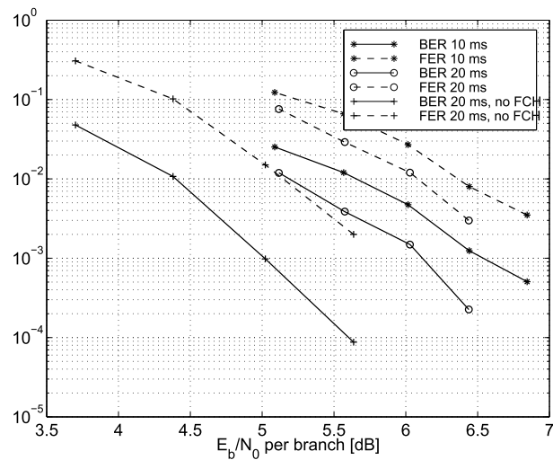
Figure 5. Speech, Vehicular A 120km/h, with antenna diversity.
