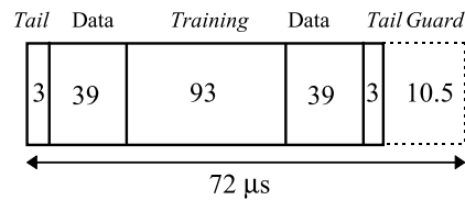
Figure 3-14 The 1/64-slot Synchronisation burst
