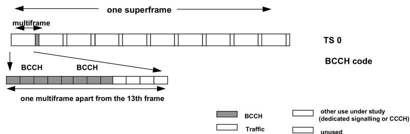
Mapping of the BCCH logical channel
