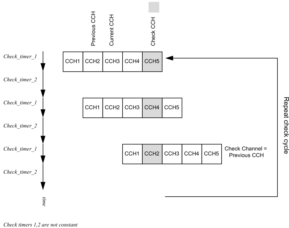
Figure 10. Check channel cycle.
