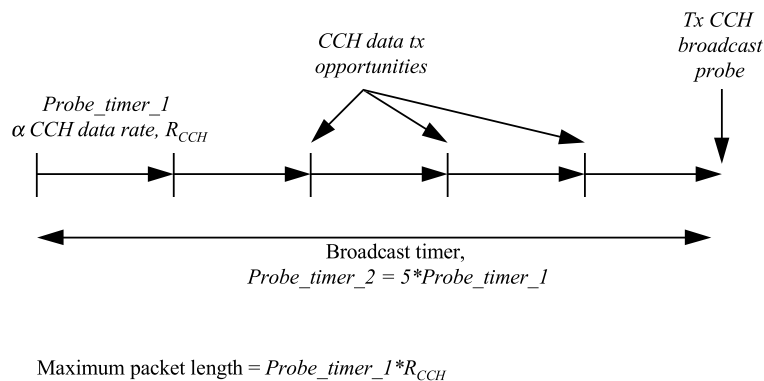
Figure 12. CCH Timer Relationships.
