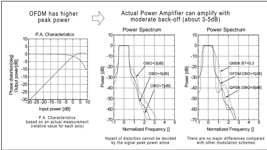
Figure 18: Comparison of OFDM, GMSK and OFDM with non-linear PA
