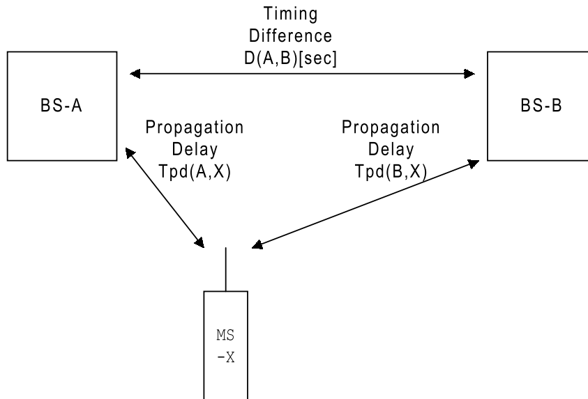
Figure 11: Pseudo Synchronisation
