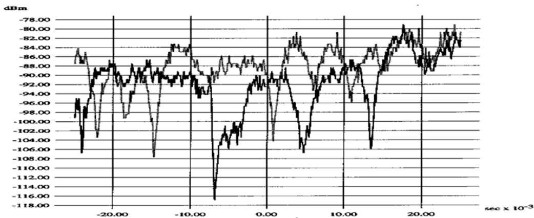
Figure 8: RSSI of Both Antennas ( Vehicular speed = 80[km/h] )
