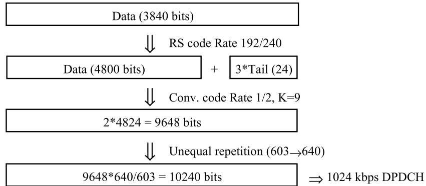
Figure 15 Channel coding and service mapping for a 384 kbps bearer (384 kbps LCD service)
