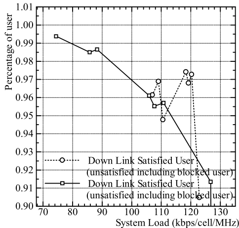
Figure 46: System Bandwidth 3.2MHz
