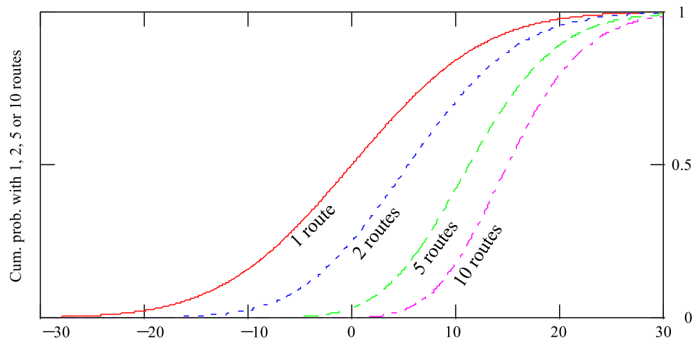
Figure 5 Benefits of Path Selection - Space Diversity
