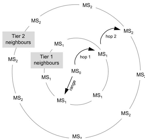
Figure 14. Localised connectivity through probing.
