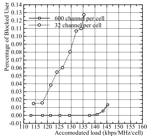
Figure 41: Blocking versus Load
