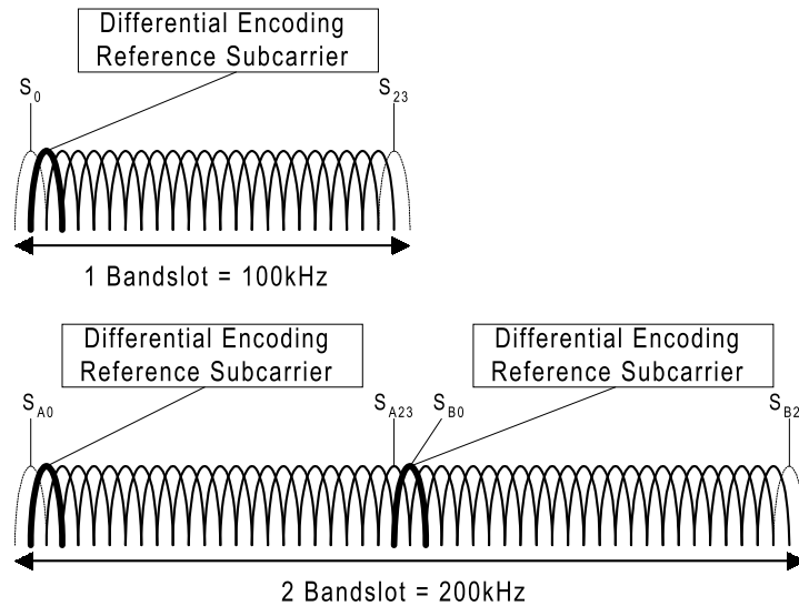
Figure 12: Reference Subcarrier Allocation
