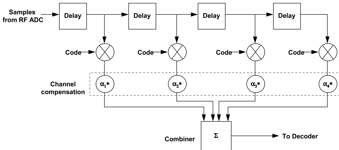
Figure 24 WCDMA Rake Receiver
