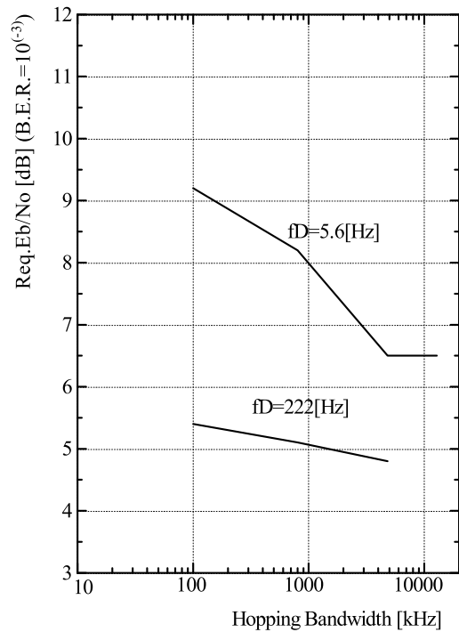
Figure 3: Required E_b/N_0 versus Hopping Bandwidth
