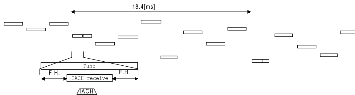
Figure 12 Puncturing Scheme ( 1 of 4 time slot usage )
