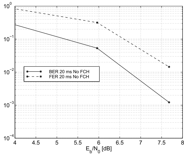
Figure 8. Speech, Vehicular B 120 km/h, without antenna diversity.
