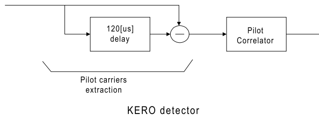
Figure 3: KERO detector
