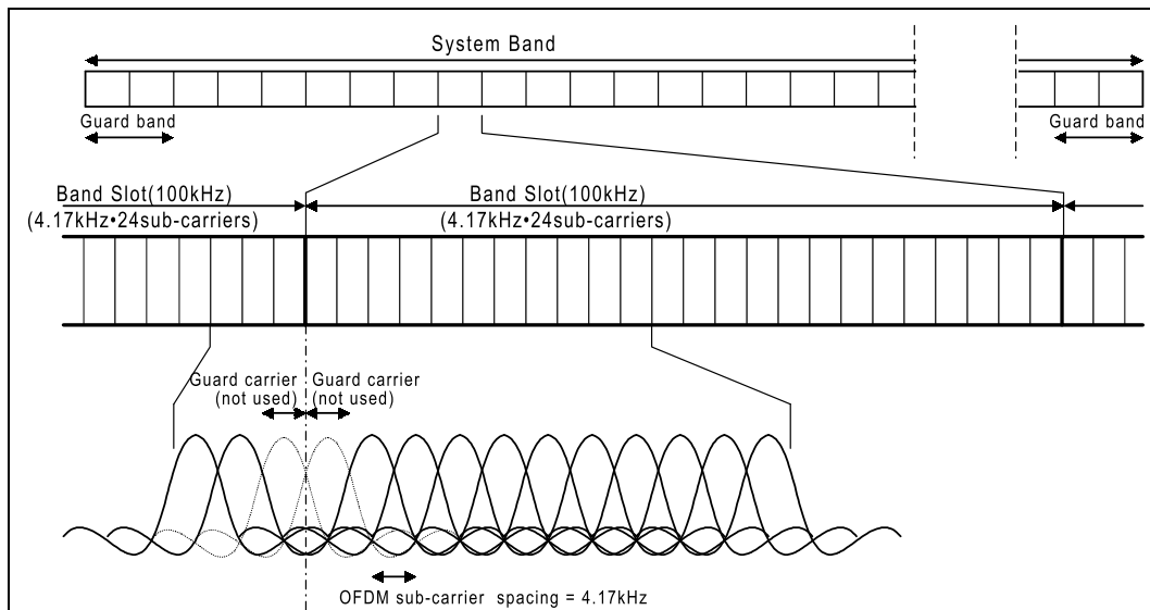
Figure 8: BDMA Frequency Structure
