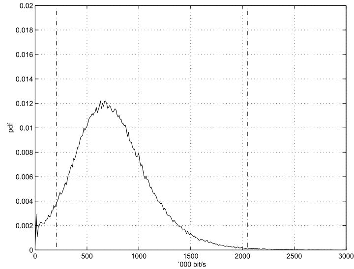
Figure 3. Histogram for session throughputs.
