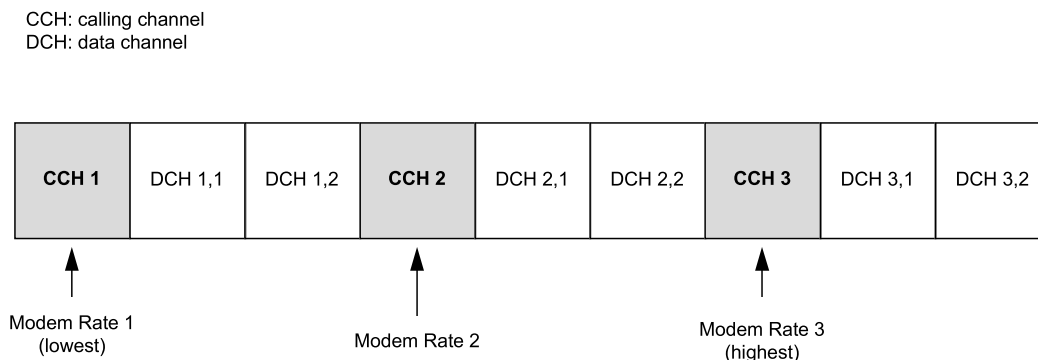
Figure 9. Logical Channels in ODMA.
