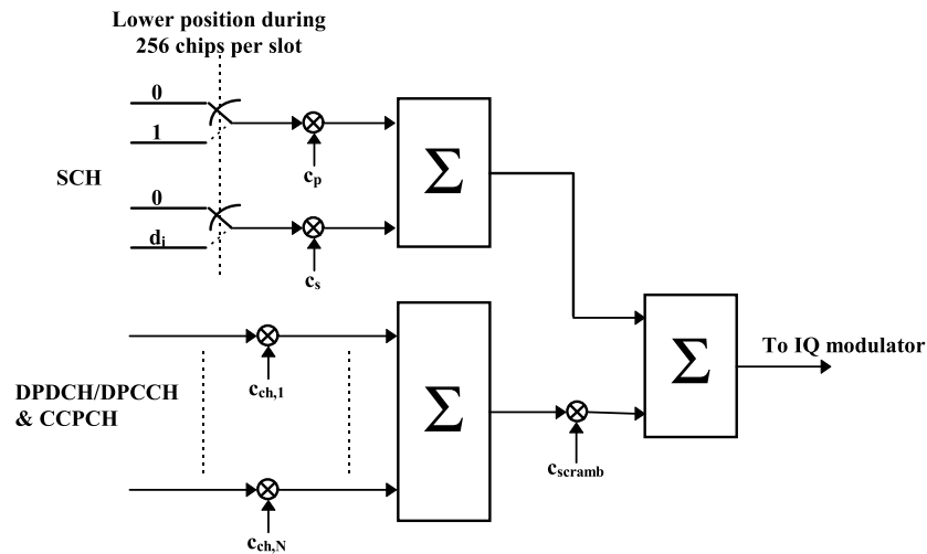
Figure 9 Multiplexing of SCH
