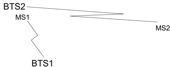
Figure 2 : Near-far effect for non-colocalised base stations
