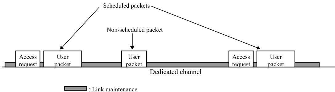
Figure 30 Multi-packet transmission on dedicated channel
