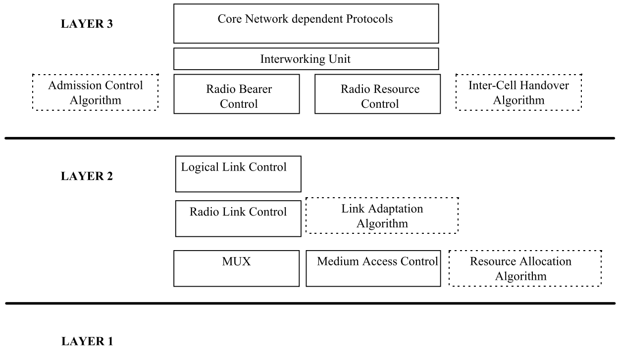
Figure 4-1. WB-TDMA Radio interface
