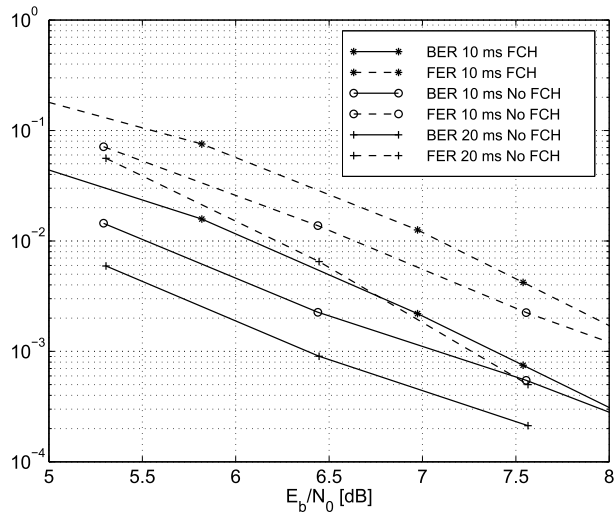
Figure 2. Speech, Indoor office A, without antenna diversity.
