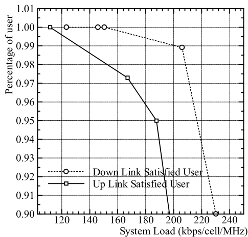
Figure 53: Satisfied User Rate
