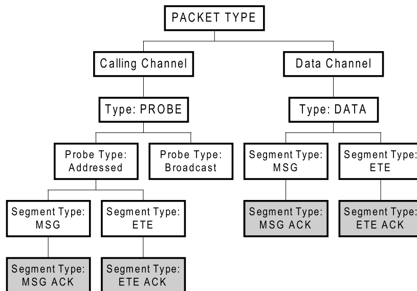
Figure 13 ODMA Packet Structures
