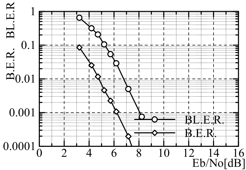
Figure 32 E_b/N_0 vs BL.E.R. ( Mode A, Vehicular)
