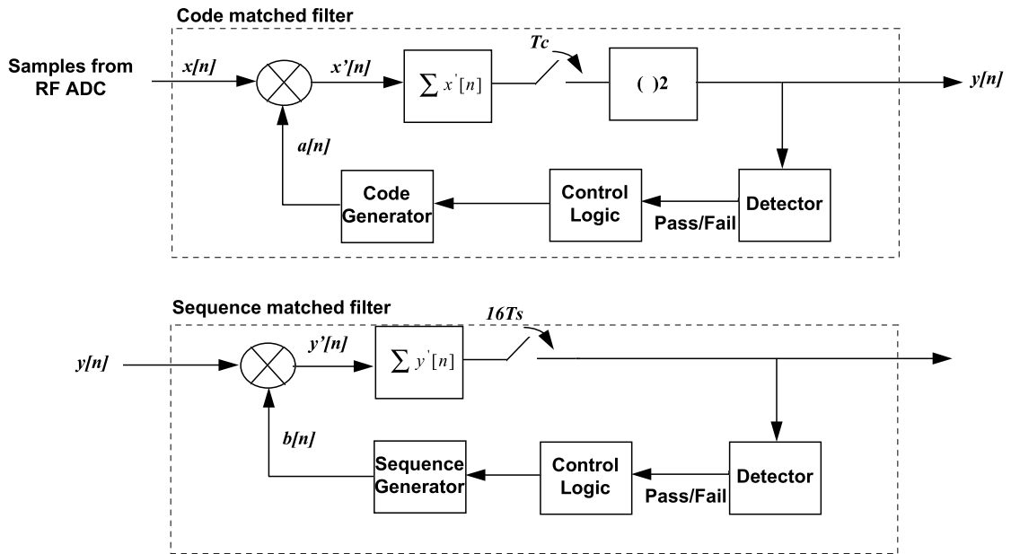
Figure 23 Receiver Matched Filters
