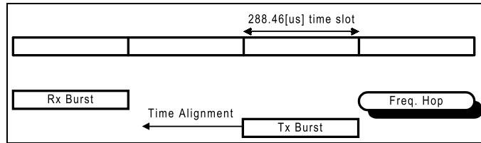
Figure 17: 4-TDMA frame and frequency hopping
