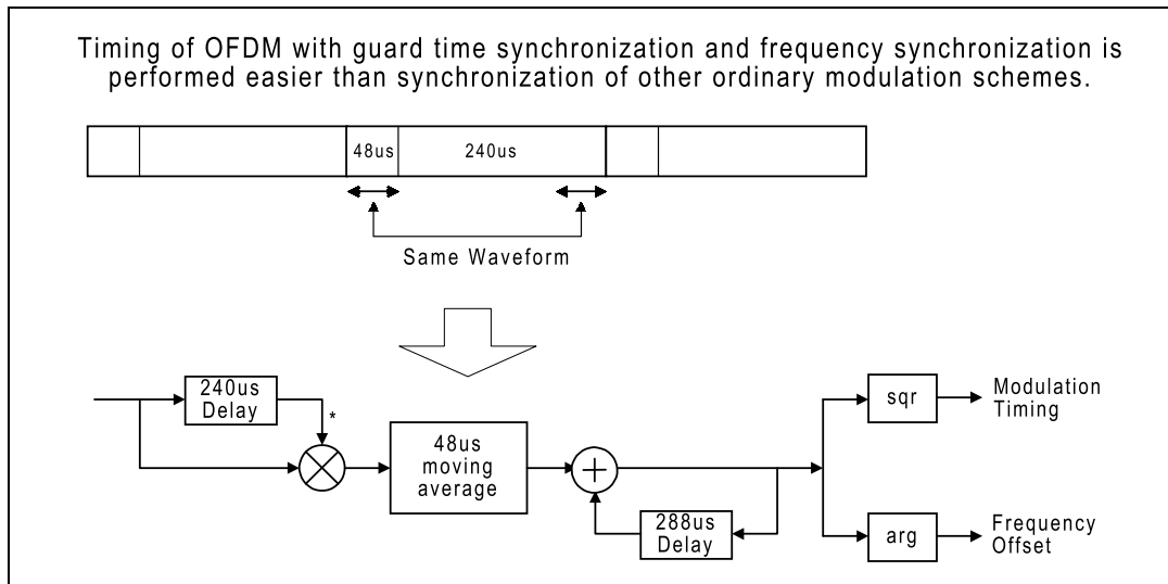
Figure 14: Synchronisation (Schematic)
