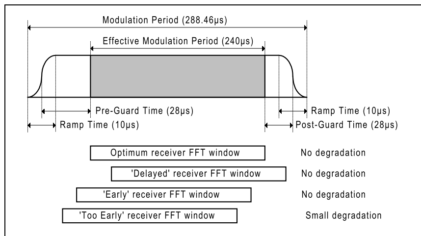
Figure 14: OFMDA burst and synchronisation requirements
