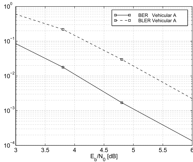
Figure 14. UDD 144, without antenna diversity.
