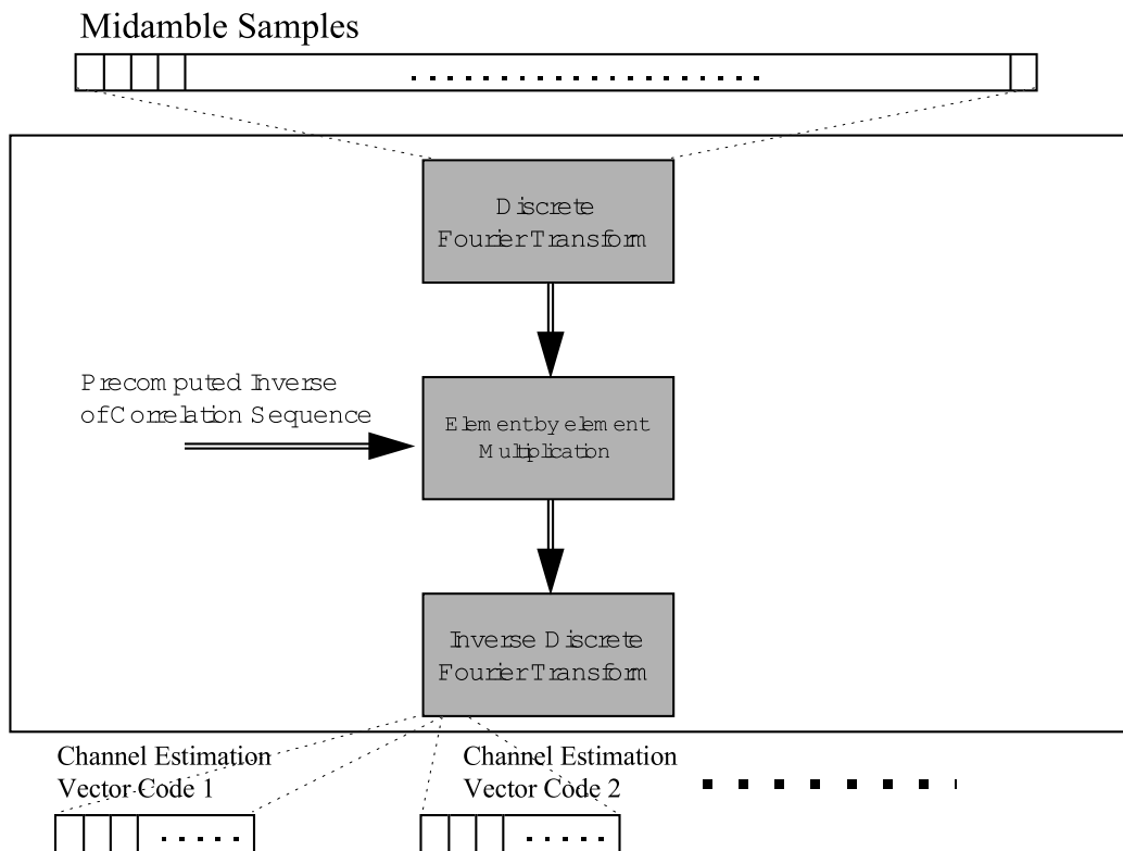
Figure 24 WB-TDMA/CDMA Fast Correlator
