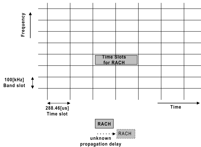
Figure 4: RACH Structure
