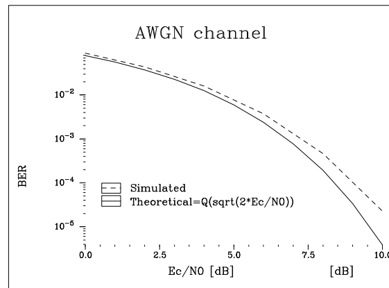
Simulated results compared to theoretical value in AWGN channel (overhead due to training sequence and tail bits is not to be taken into account in E_c/N_0 )
