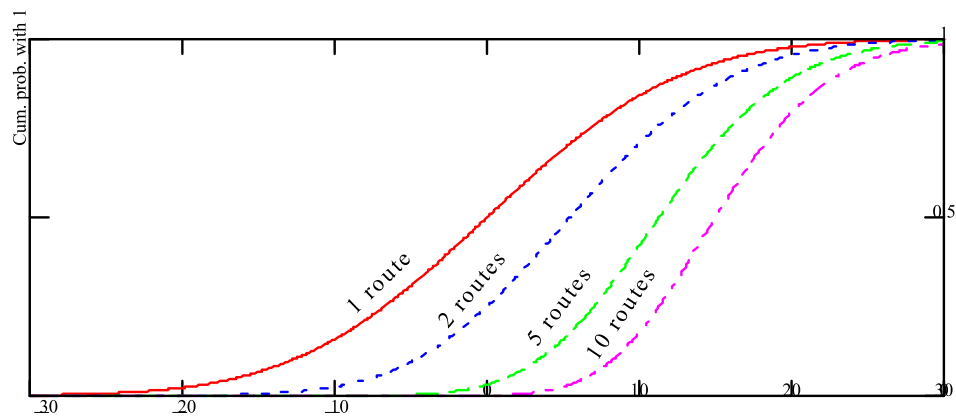
Figure 4 Benefits of Path Selection - Space Diversity
