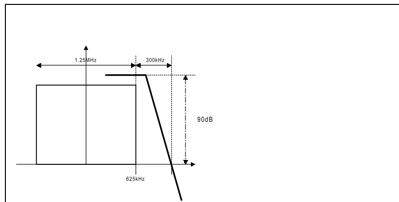
Figure 16: IS-95 filter requirements (for reference)
