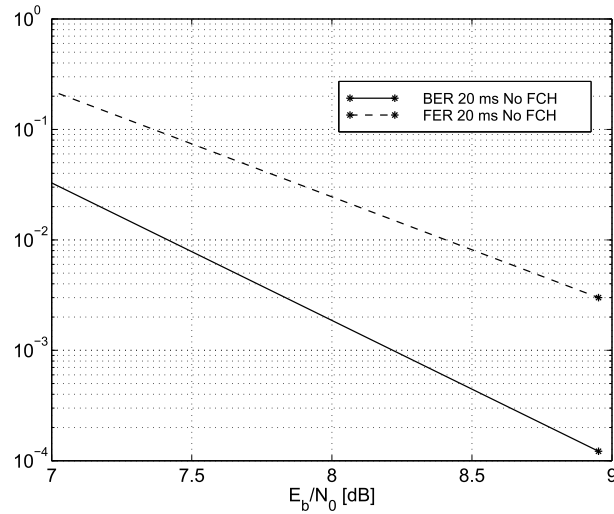
Figure 10. Speech, Vehicular B 250 km/h, without antenna diversity.
