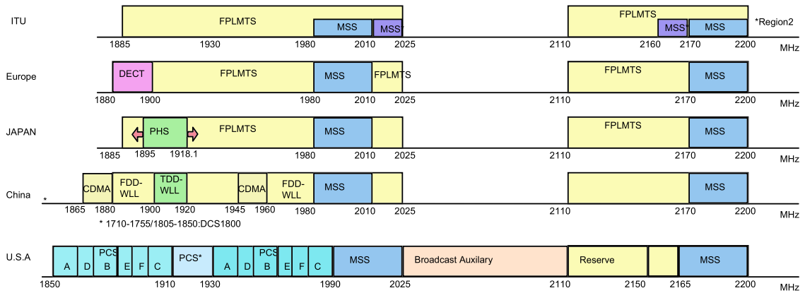
Figure 34 Frequency allocation around the world
