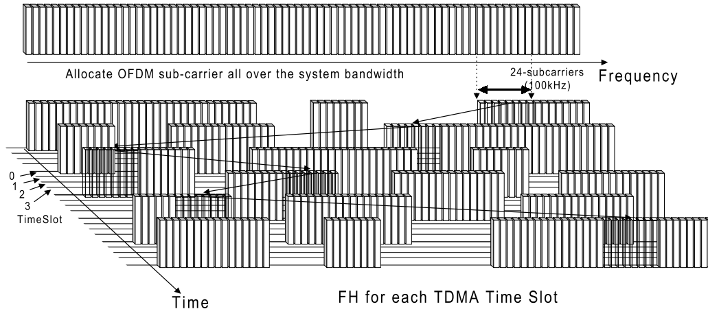
Figure 1: OFDMA Outline (SFH-TDMA)
