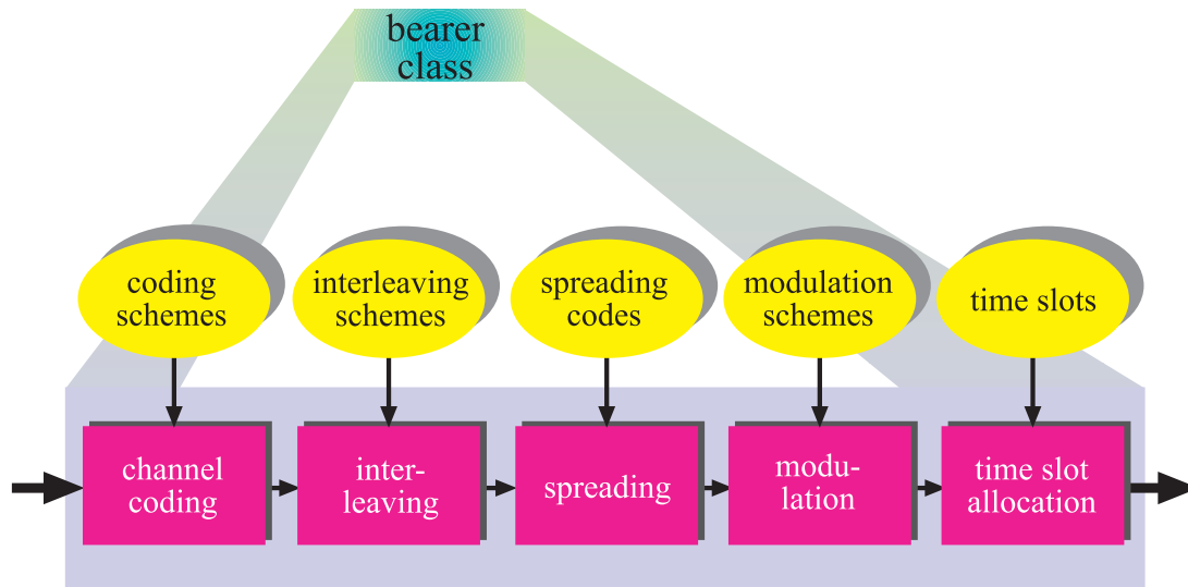
Figure 2.1 Bearer class
