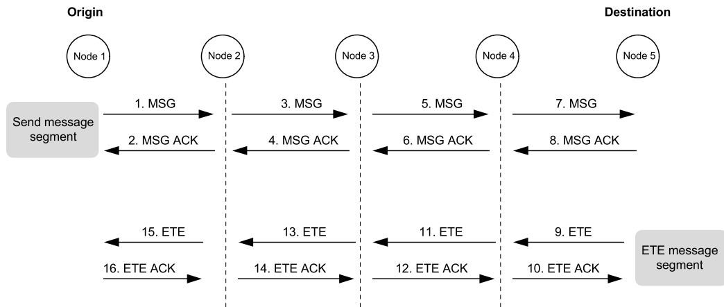
Figure 16. ODMA Layer 2 RLP.
