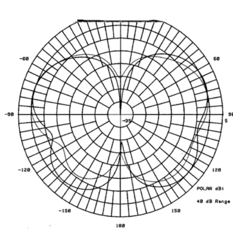
Figure 6: Antenna Pattern (Rod)
