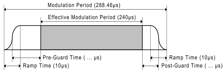
Figure 7: OFDM Modulation Burst
