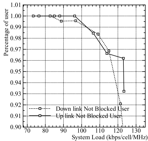
Figure 43: System Bandwidth 3.2MHz
