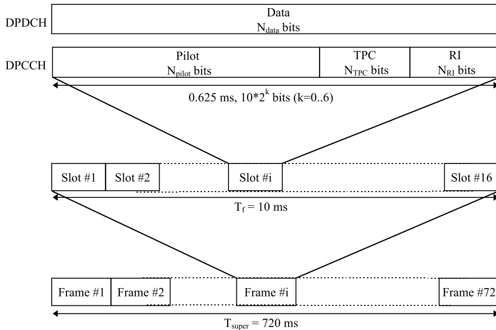
Figure 5 Frame structure for uplink dedicated physical channels
