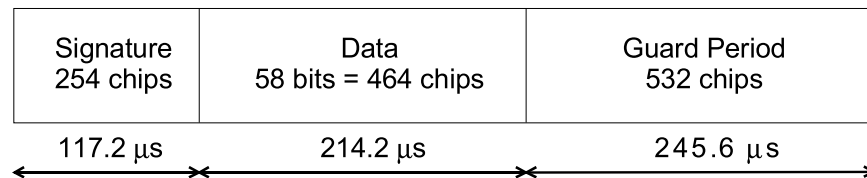
Figure 2 : Long access burst
