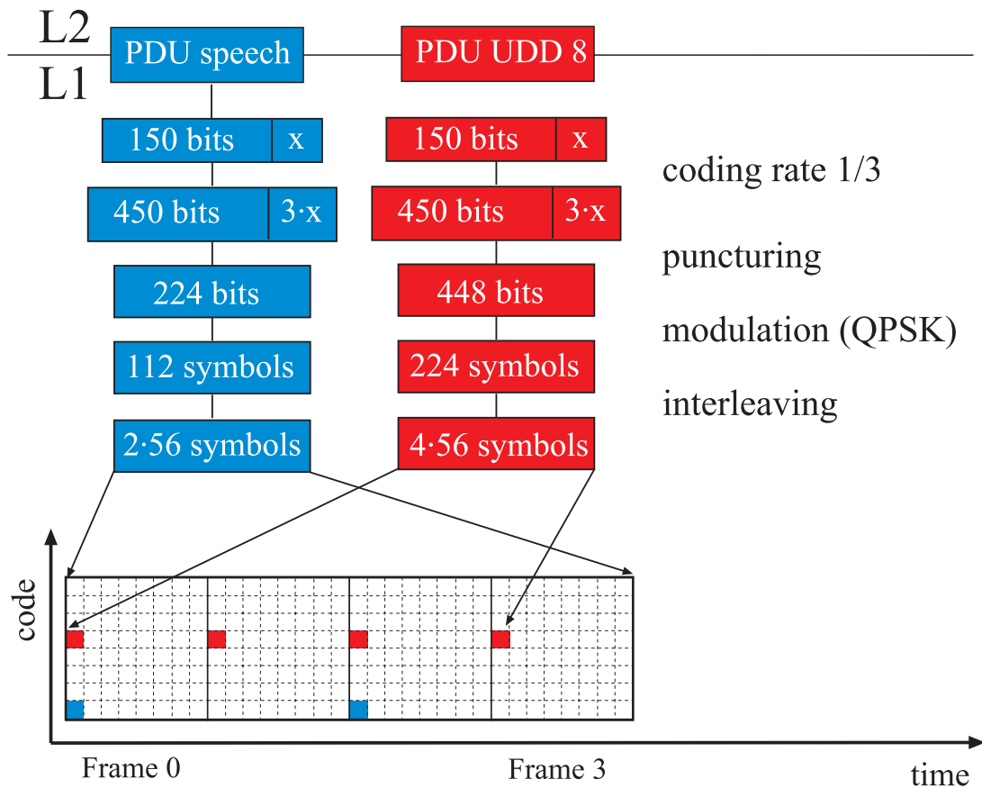
Figure 3.5 50% speech + 50% UDD 8 (short UDD 8 packets)
