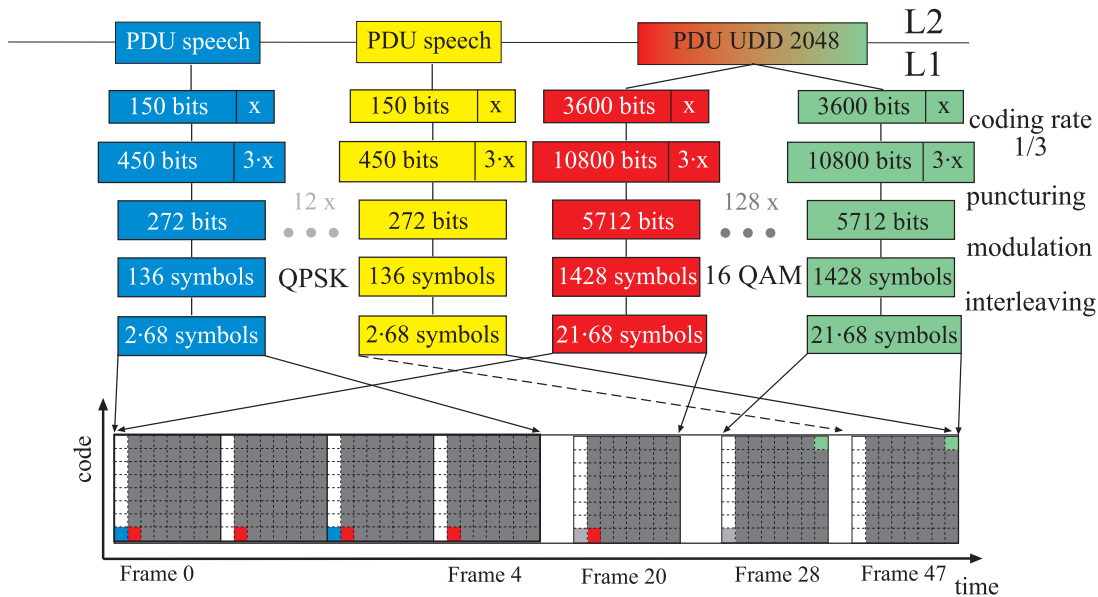
Figure 3.8 50% speech + 50% UDD 2048
