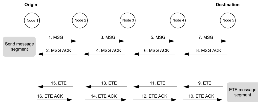
Figure 17. ODMA Layer 2 RLP.
