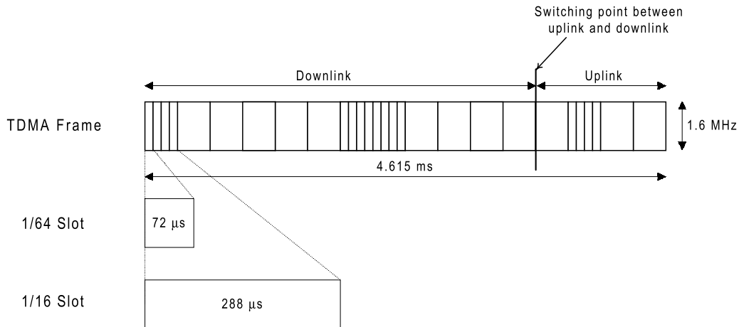
Figure 3-4 The unit TDD frame structure of WB-TDMA..
