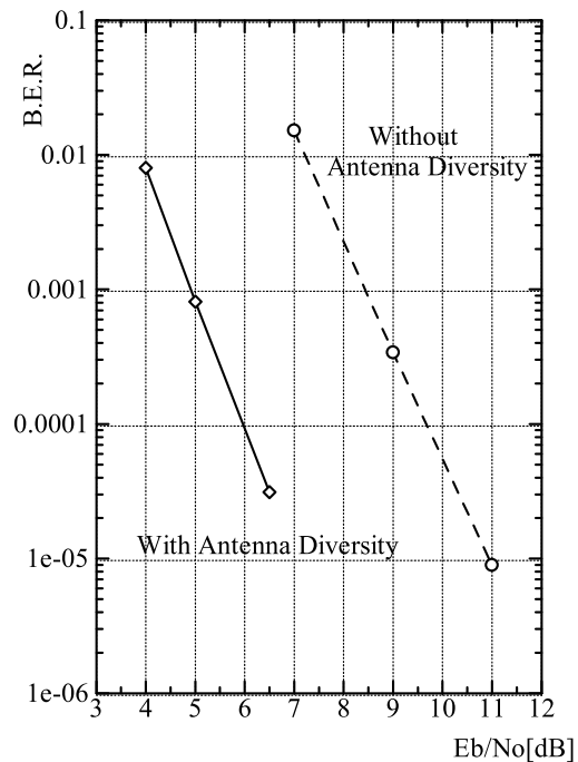
Figure 10: B.E.R. vs E_B/N_0
