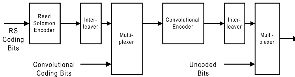
Figure 10: Encoder Structure
