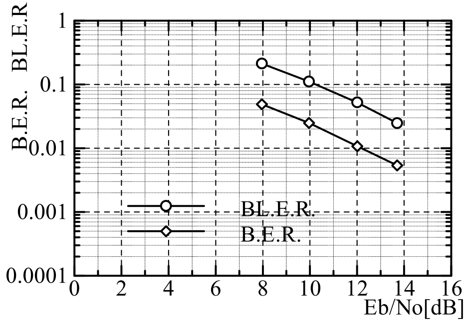
Figure 37 Eb/No vs BL.E.R. (UUD2048, Pedestrian)
