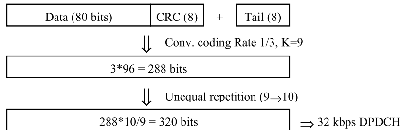
Figure 13 Channel coding and service mapping for an 8 kbps bearer (8 kbps speech service)
