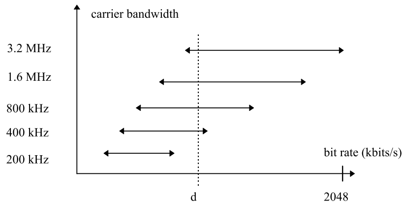
Figure 5-5 : bit rate range for each carrier type
