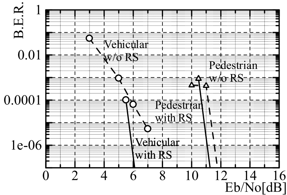
Figure 28: Eb/No vs BER (LCD 144)
