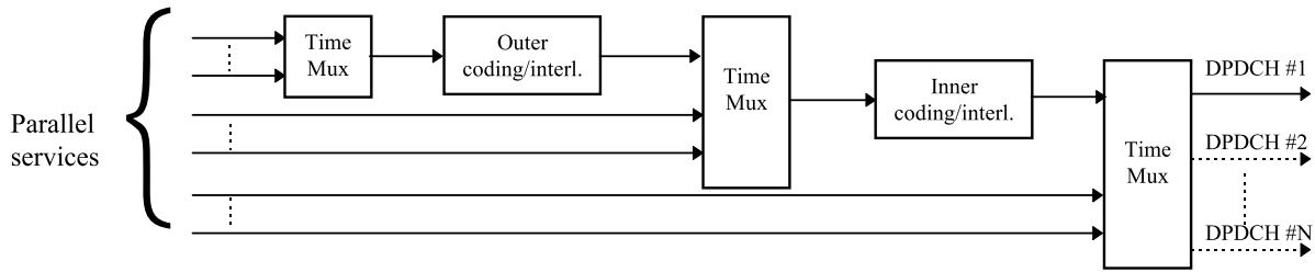
Figure 11 Service multiplexing of WCDMA
