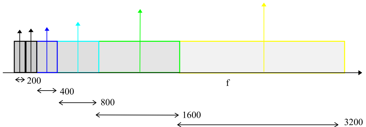
Figure 3-2 :- Multi-band TDMA system concept
