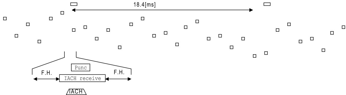
Figure 19 Puncturing Scheme (1 of 4 Time slot usage)
