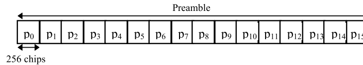
Figure 19 Structure of Random-Access burst preamble part
