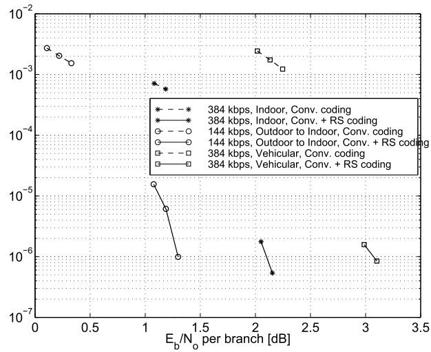
Figure 11. LCD 144 and LCD 384, with antenna diversity.
