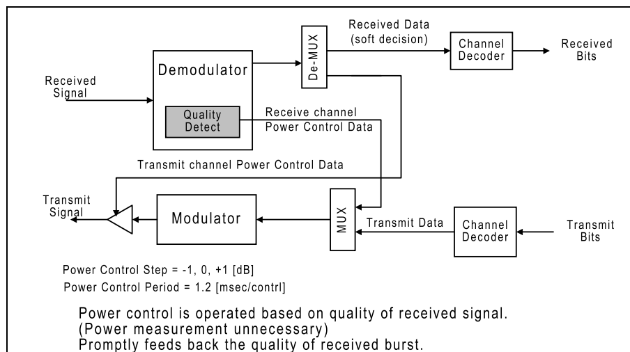
Figure 23: Operation of Power Control
