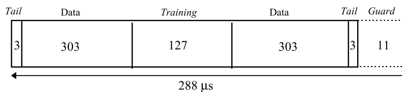
Figure 3-13 The 1/16-slot Synchronisation burst.
