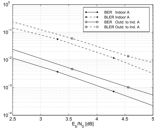
Figure 18. UDD 2048, information bit rate of 480 kbps, without antenna diversity.
