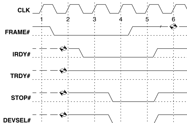
Figure 3-9: Retry
