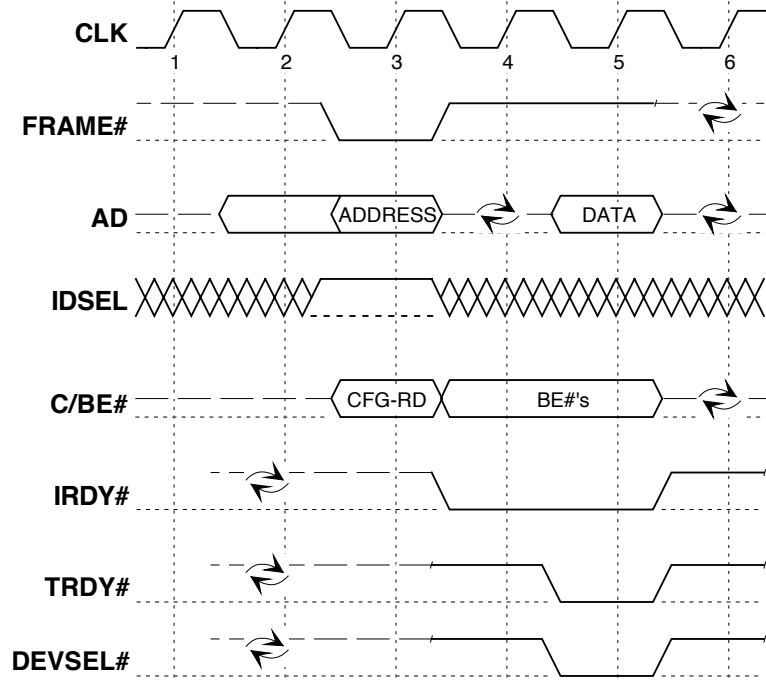
Figure 3-4: Configuration Read
