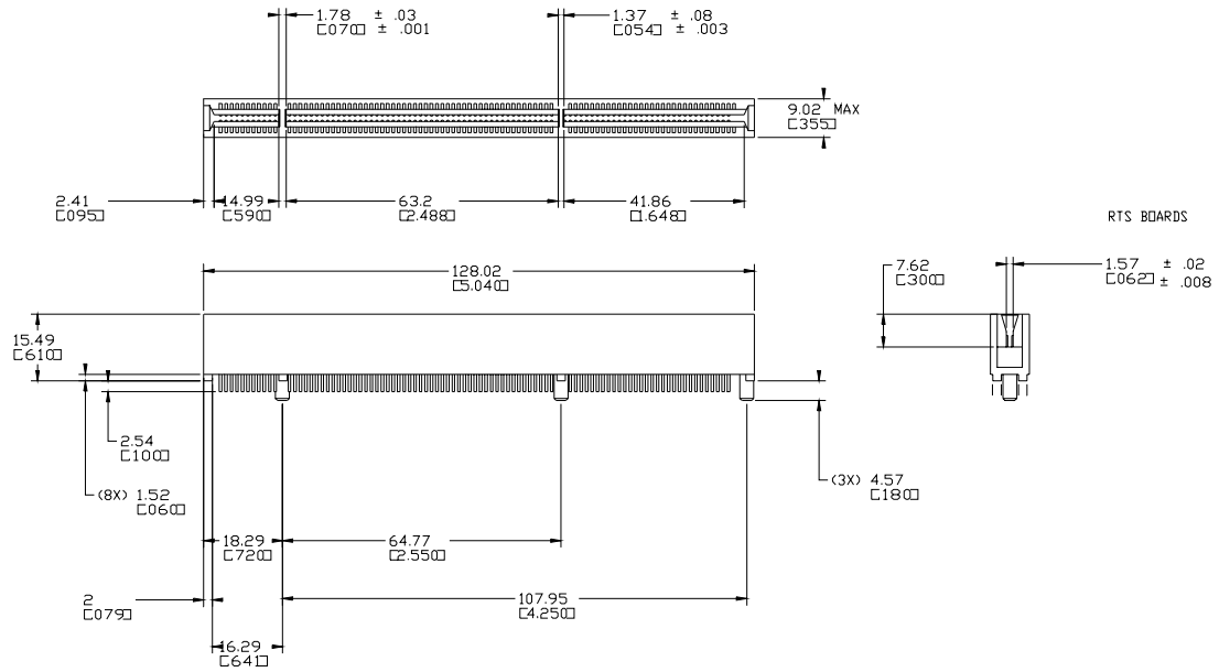
Figure 5-24: 3.3V/64-bit Connector
