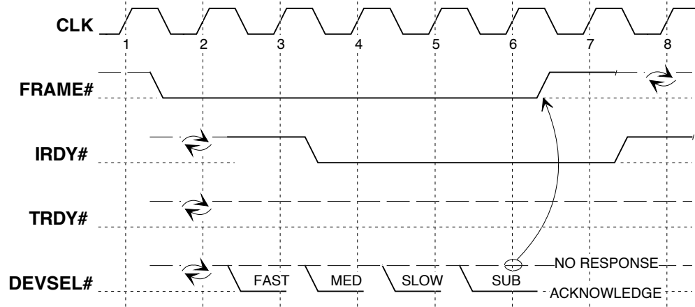
Figure 3-17: DEVSEL# Assertion
