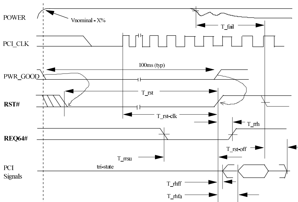
Figure 4-11: Reset Timing 34
