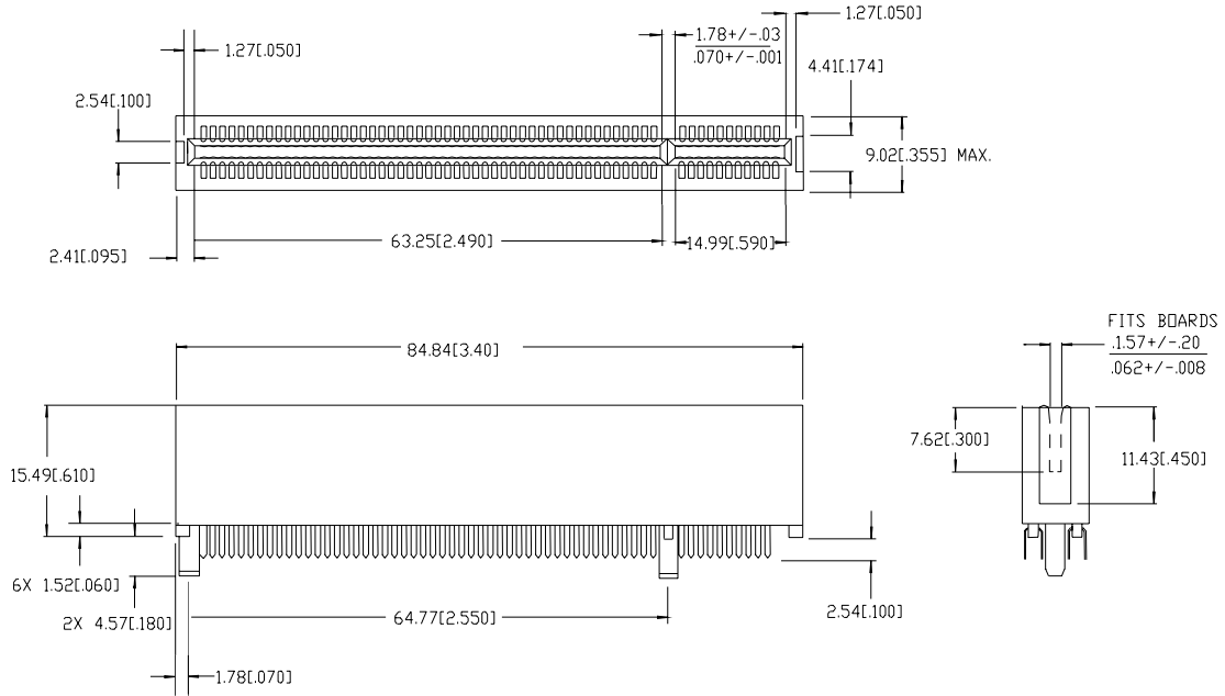
Figure 5-19: 32-bit Connector
