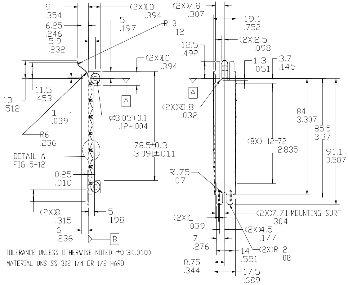
Figure 5-17: MC Bracket
