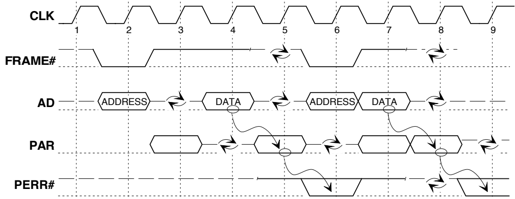
Figure 3-20: Parity Operation
