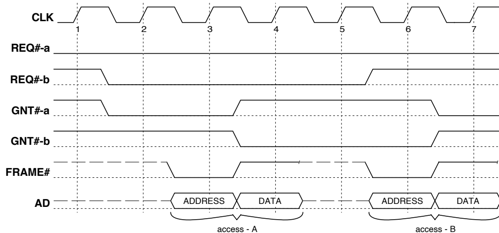
Figure 3-15: Basic Arbitration
