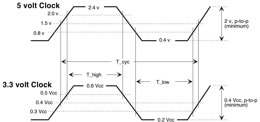
Figure 4-6: Clock Waveforms
