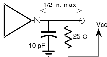
Figure 7-6: T_{val(max)} Falling Edge
