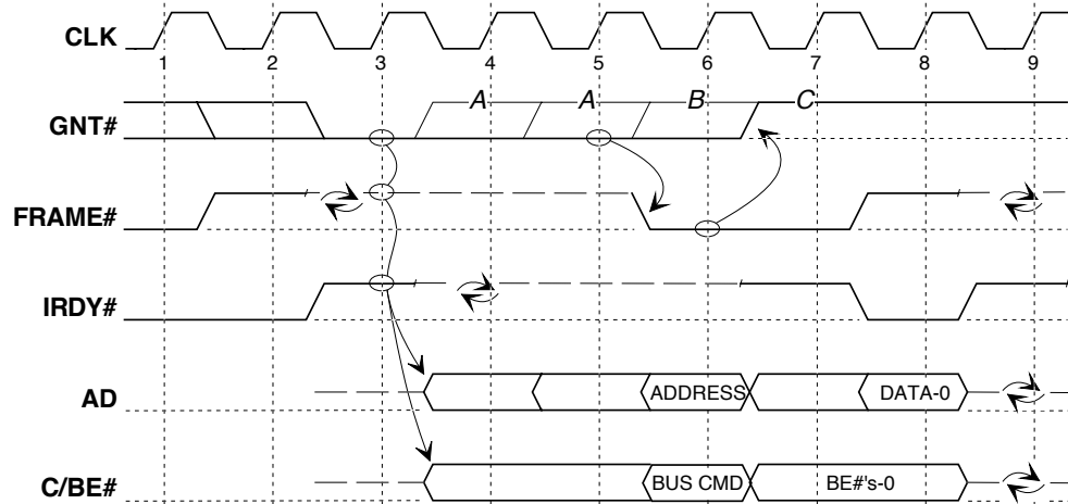
Figure 3-18: Address Stepping
