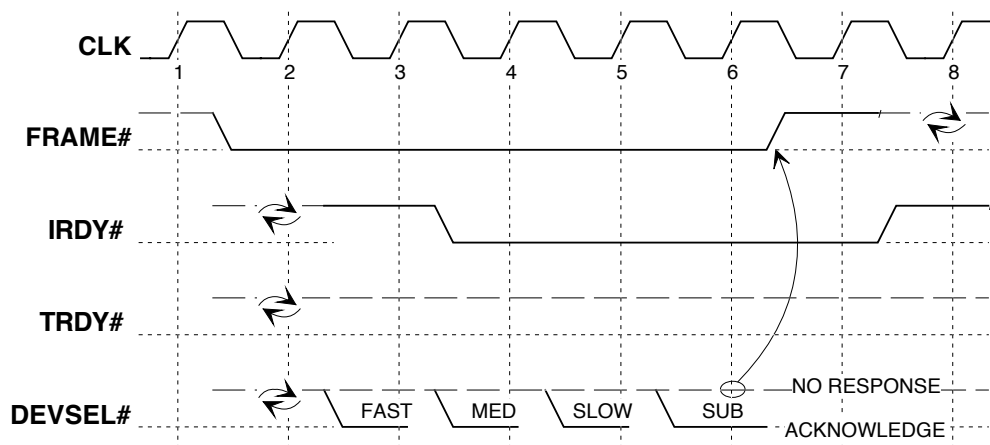
Figure 3-8: Master-Abort Termination
