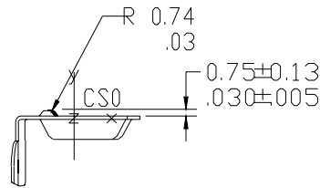
DETAIL A SCALE 3.000 12X
