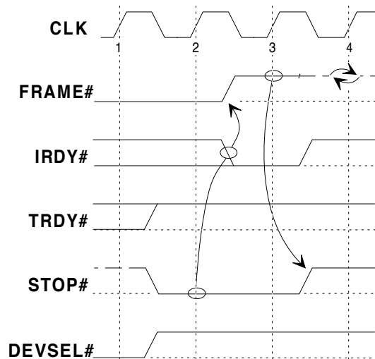
Figure 3-14: Target-Abort
