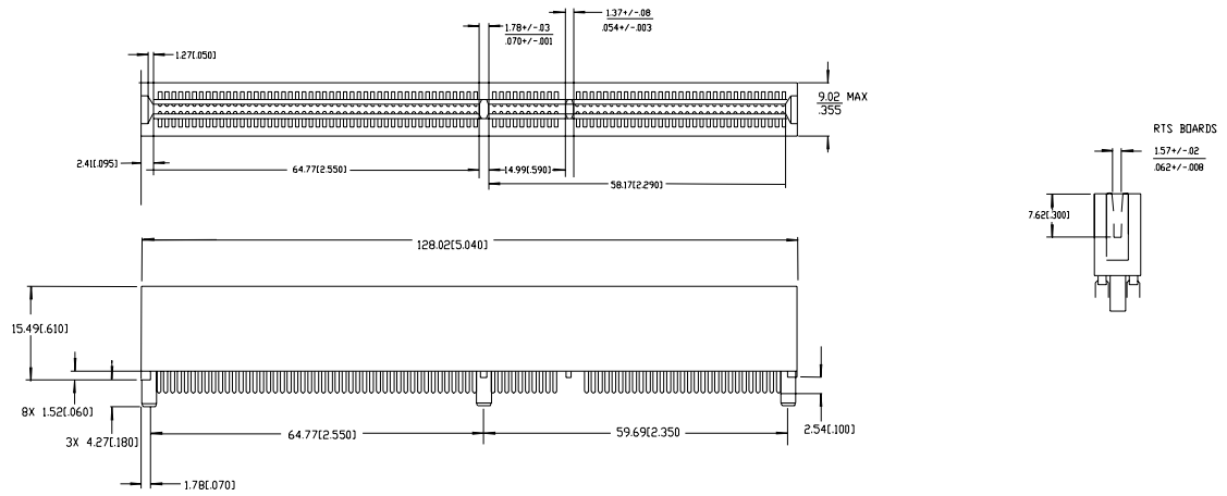
Figure 5-22: 5V/64-bit Connector
