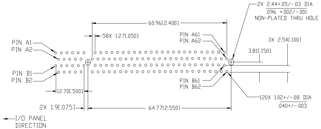
Figure 5-21: 3.3V/32-bit Connector Layout Recommendation
