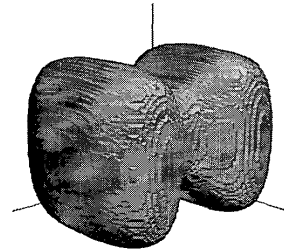
Figure 4 - Area of field strength greater than or equal to 4A/m created by two square coils carrying 24A
