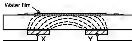
Figure 1-3 Fields With a Conductive Film
