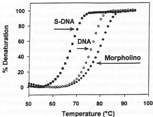
Fig. 3. Thermal transitions of 20-mer oligo/RNA duplexes. Oligo sequence: 5'-GGUGGUUCCUUCAGUCGG (T replaces U in DNA and S-DNA).
