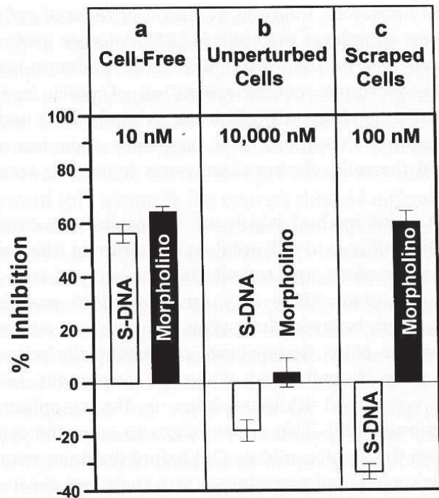
Fig. 7. Translational inhibition by 25-mer antisense oligos targeted against globin/luciferase mRNA: (a) in cell-free translation system with 10 nM oligo and 1 nM mRNA; (b) in unperturbed HeLa cells expressing globin/luciferase mRNA and treated with 10000 nM oligo for 16 h; (c) in HeLa cells expressing globin/luciferase mRNA and scrape-loaded in the presence of 100 nM antisense oligo. Oligo sequence: 5'-GGUGGU-UCCUUCUCAGUCGGACUGG.
