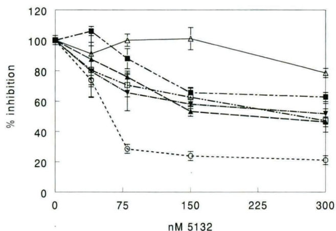
Figure 2. Inhibition of alternate structure clones by ISIS 5132. Cells were transfected with the luciferase reporter plasmids diagrammed in Figure 1, then treated in duplicate with oligonucleotide at doses ranging from 40 to 300 nM. Luciferase expression was measured the following day. Results are percent luciferase expression compared to the no oligonucleotide control. Open triangle, S20; open circle, S0; inverted closed triangle, S20-10-5; closed square, S20-10-3; closed triangle, S10-4; open square, S10-14.
