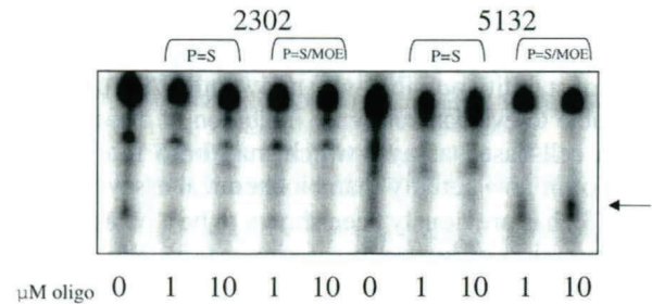
Figure 5. RNase cleavage of S20 targets. Forty-four base S20 RNA targets were synthesized and labeled as described in Materials and Methods. Targets were hybridized with unmodified deoxyphosphorothioate (P=S) or chimeric deoxyphosphorothioate/2'-O-methoxyethyl base (P=S/MOE) oligonucleotides complementary to the target sequences in 1× RNase H buffer at either 1 or 10 μM. Cleavage was initiated by the addition of 0.5 U RNase H. Cleaved target RNA was visualized by electrophoresis on a denaturing acrylamide gel. The arrow at the right of the figure indicates the position of the expected cleavage product.
