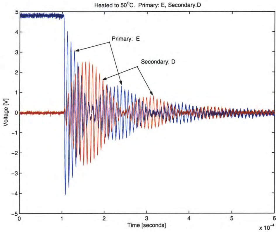
Figure 7-39: Output waveforms of heated coil and capacitor components. Operation at 50°C does not significantly affect operation.
