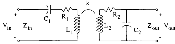
Figure 5-1: Schematic showing the coupled resonant circuits as well as their input and output ports.
