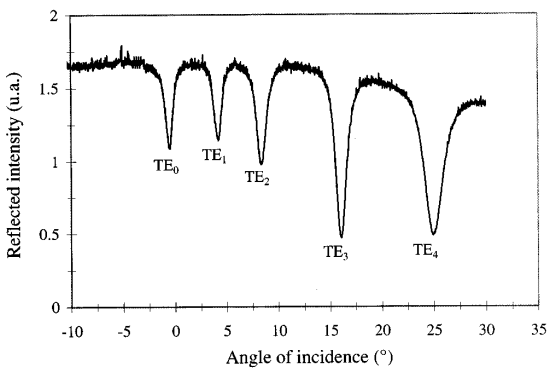
FIG 2 TE guided mode spectra obtained by measuring the reflected intensity vs the angle of incidence ( n_o excitation)
