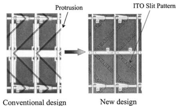
FIGURE 2-4 Real pixel design with protrusions or slits.
