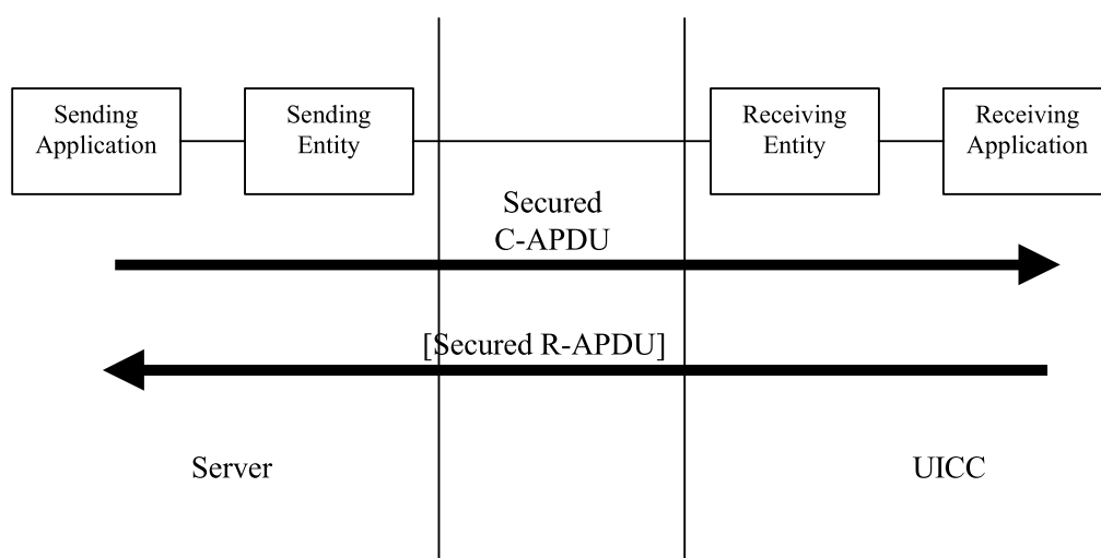
Figure 4.1: Remote management
