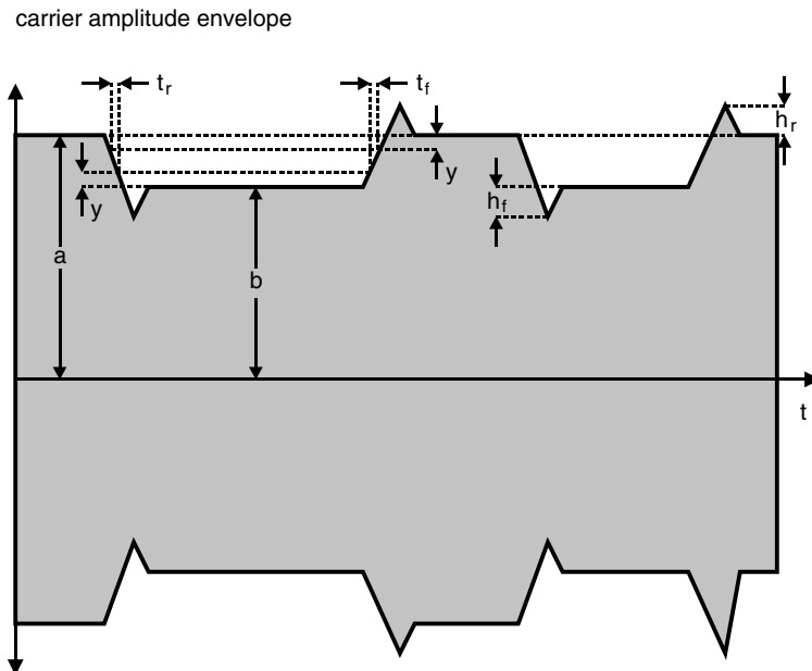
Figure 3.90 Type-B carrier modulation. A continuous supply of energy is made possible by the small modulation index (10 %). Here t_r, t_f \leq 2 \mu\text{s} , y = 0.1 \cdot (a - b) and h_f, h_r \leq 0.1 \cdot (a - b)
