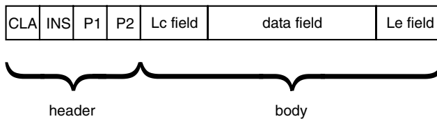
Figure 6.39 Structure of a command APDU
