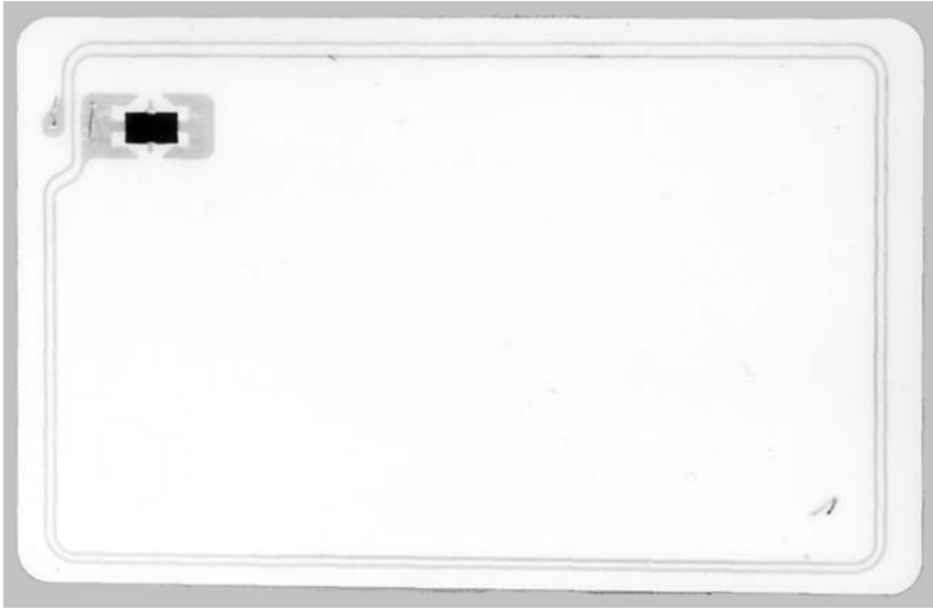
Figure 10.43 Printed coil for a contactless smart card
