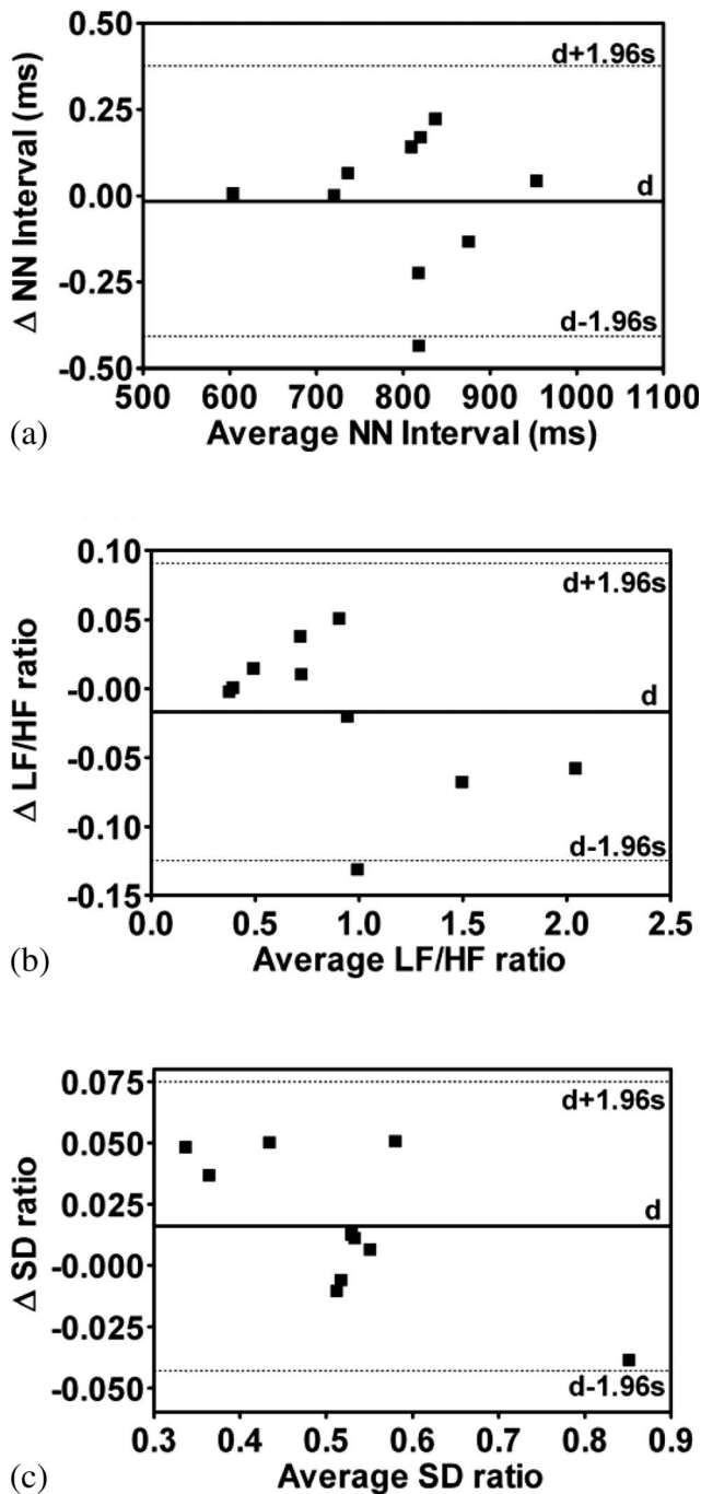
Figure 6. Bland-Altman agreement analysis between ECG and PPG methods showed higher agreement of HRV parameters: heart rate interval (a), LF/HF ratio (b) and SD ratio (c). Solid lines indicate mean difference and dotted lines refer to boundaries of 95% limits of agreement.
