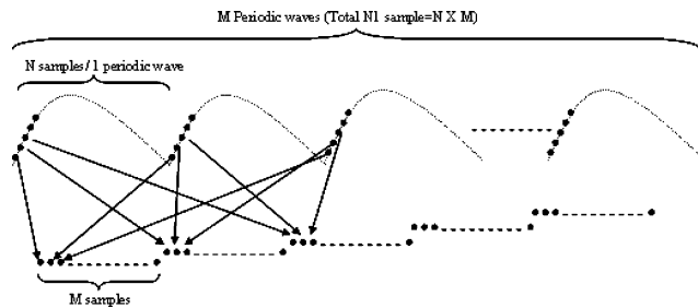
Fig. 2. Block interleaving.
