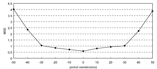
Fig. 4. MSE with respect to the amount of period mismatch.
