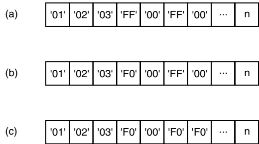
Figure 7.6 Example of write accesses to an EF with a transparent structure using the sequence of commands shown in Figure 7.5
