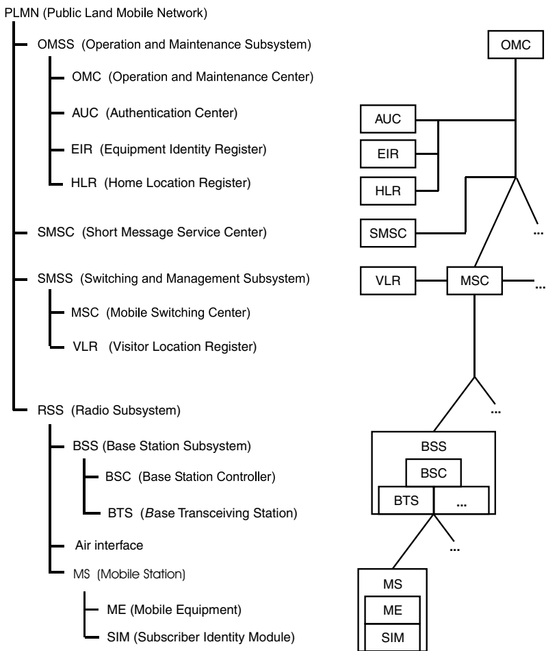
Figure 13.9 Basic architecture of a typical mobile telecommunications system compliant with the GSM 01.02 specification. In this example, the EIR and HLR databases are centralized. Since many aspects of the PLMN configuration are left to the operator of a particular network, the databases may be decentralized and distributed among several MSCs if necessary (e.g., due to high network loading). For ease of understanding, a link to a short message service center (SMSC) is also shown here, although this is not a direct GSM system component. One or more radio subsystems may be combined to form a location area (LA), and one or more network and switching subsystems may be combined to form a service area (SA)
