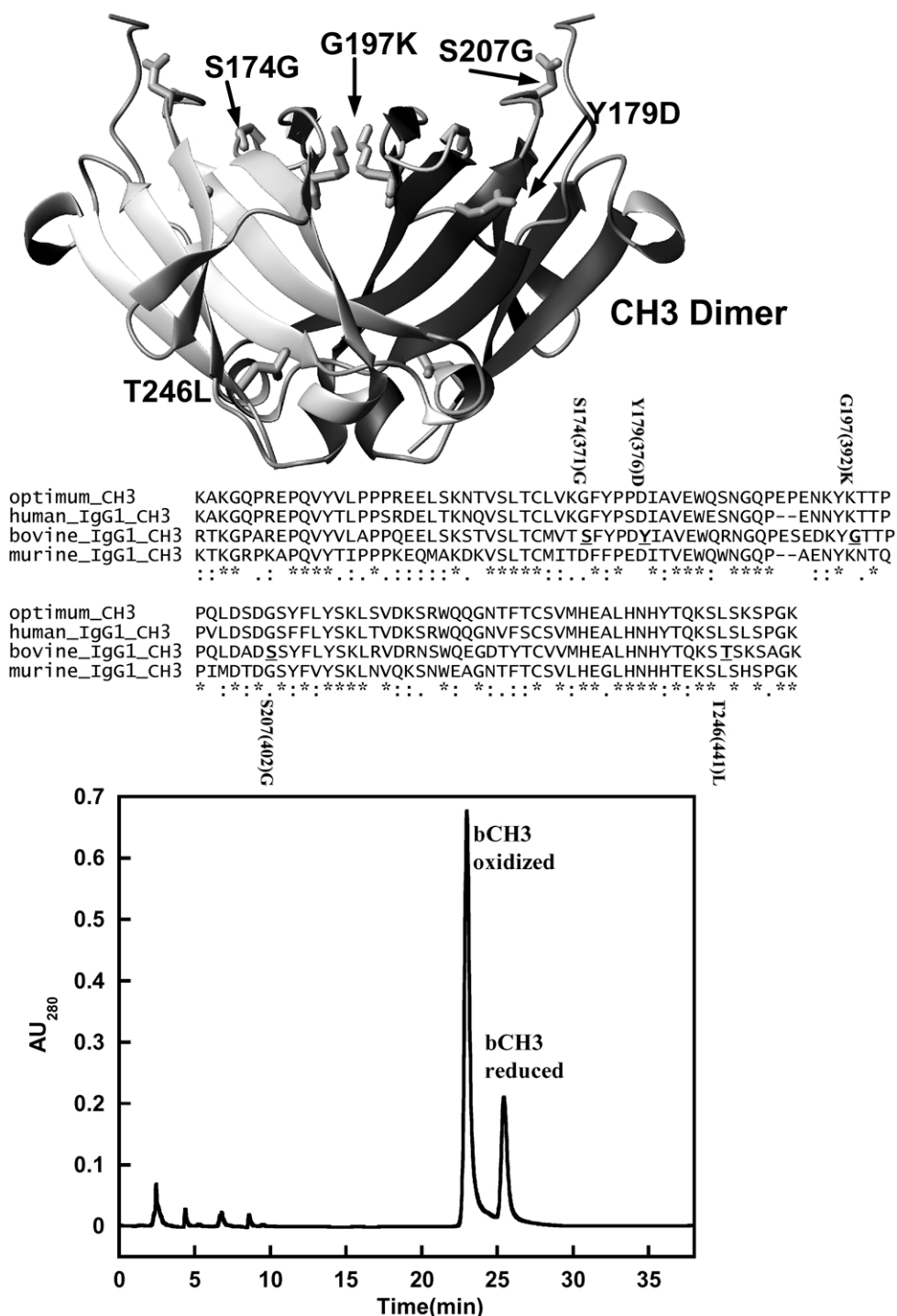
Figure 1. Top: A ribbon diagram of the X-ray crystal structure of human C H3 . 20,39 Residue positions identified as potential sites for optimization on the basis of residue frequency analysis are displayed in stick format. The ribbon diagram was rendered using MolMol. 32 Middle: Alignment of the consensus sequence from a non-redundant database of 36 NCBI mammalian IgG Fc sequences against the human, bovine and murine IgG1 C H3 sequences. The human C H3 domain was cloned from Genbank source #BC026038 purchased from the ATCC. Bovine C H3 was cloned from in-house bovine constructs derived from a bovine spleen cDNA library purchased from Stratagene. Murine C H3 was cloned from an in-house synthetic murine IgG1 gene based on the murine IgG1 Kabat database consensus sequence. 33 C H3 PCR inserts and commercial pET21a plasmid (Novagen) were digested using the designed Bam HI and Xho I restriction sites (enzymes from Invitrogen). Inserts were ligated into the vector using the H.C. T4 DNA ligase (Invitrogen). The QuickChange ® Site-Directed Mutagenesis kit (Stratagene) was used to create mutations in the bovine C H3 pET21a vector. Residue positions within the bovine C H3 domain where directed mutations were made are indicated. Below the alignments, (.), conservative variation; (:), strict variation; (*), no variation. All inserts and mutations were confirmed by DNA sequencing. BL21-trxB(DE3) (Novagen) was utilized as the host for IPTG-inducible cytoplasmic expression. BL21(DE3) did not yield significant amounts of oxidized protein and Rosetta-Gami (Novagen) had a significantly longer growth phase without providing a significant increase in C H3 oxidation over the BL21-trxB(DE3)
