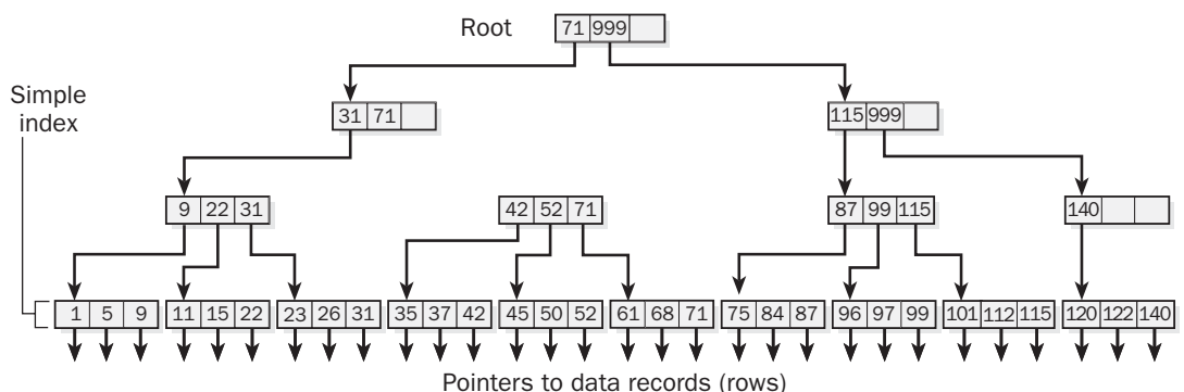
B-tree. A B-tree index structure.
