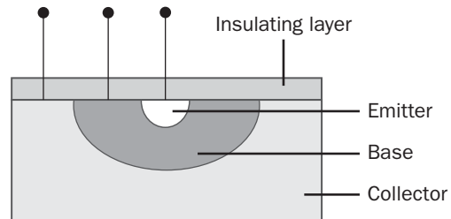
Planar transistor.
