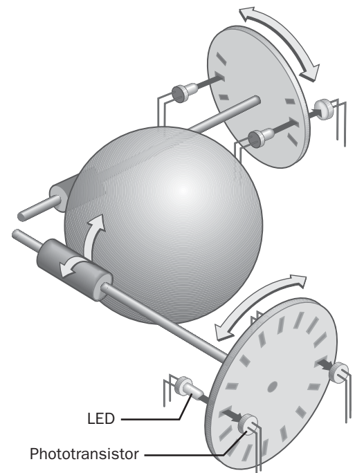
Optomechanical mouse.
