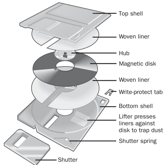
Exploded view.
