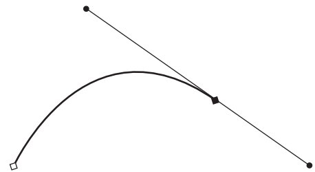
Bézier curve.
