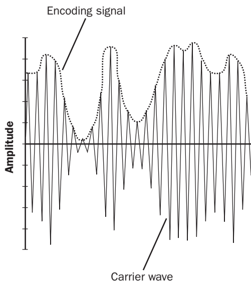
Amplitude modulation.
