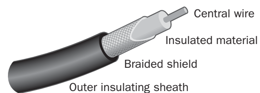
Coaxial cable.
