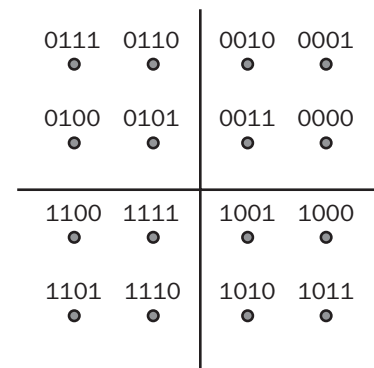
Constellation.
