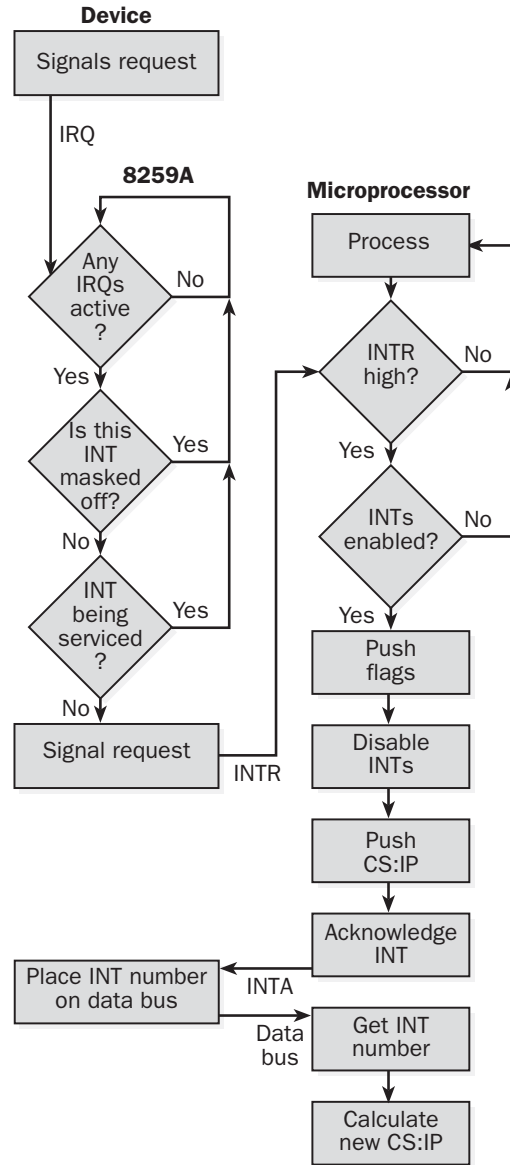
Flowchart.
