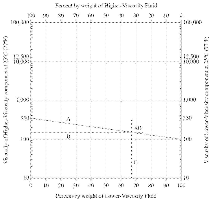
Figure 1: Blending chart for Dow Corning 360 Medical Fluid
