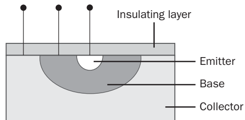
Planar transistor.
