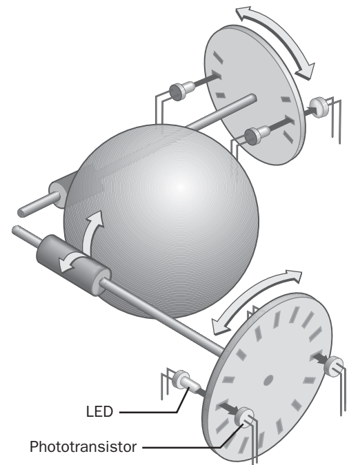
Optomechanical mouse.
