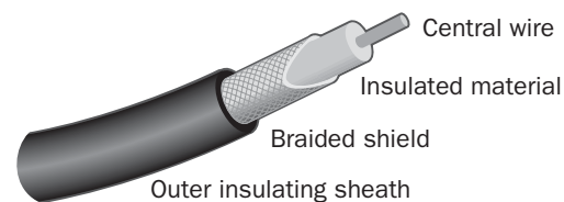
Coaxial cable.
