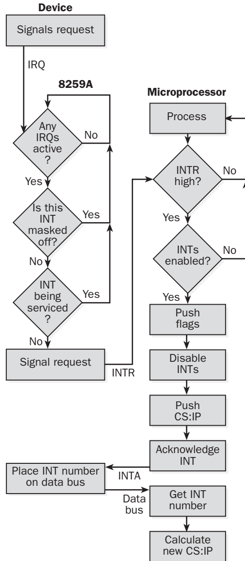
Flowchart.
