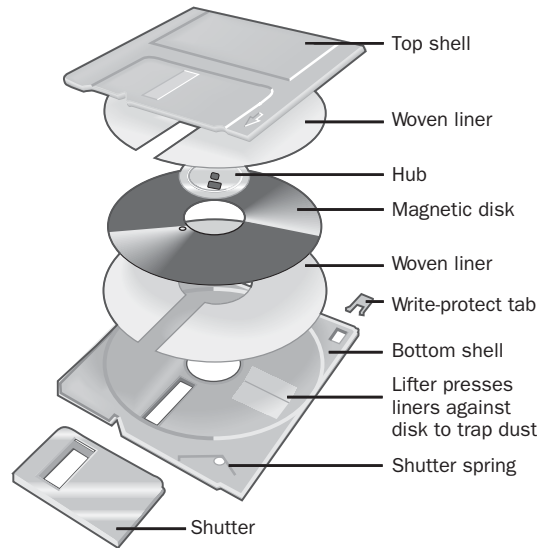
Exploded view.
