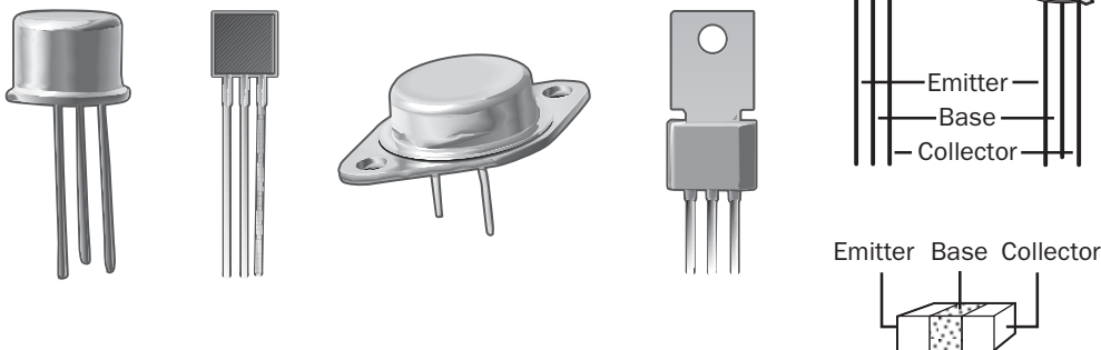
Transistor.
