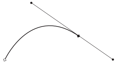
Bézier curve.
