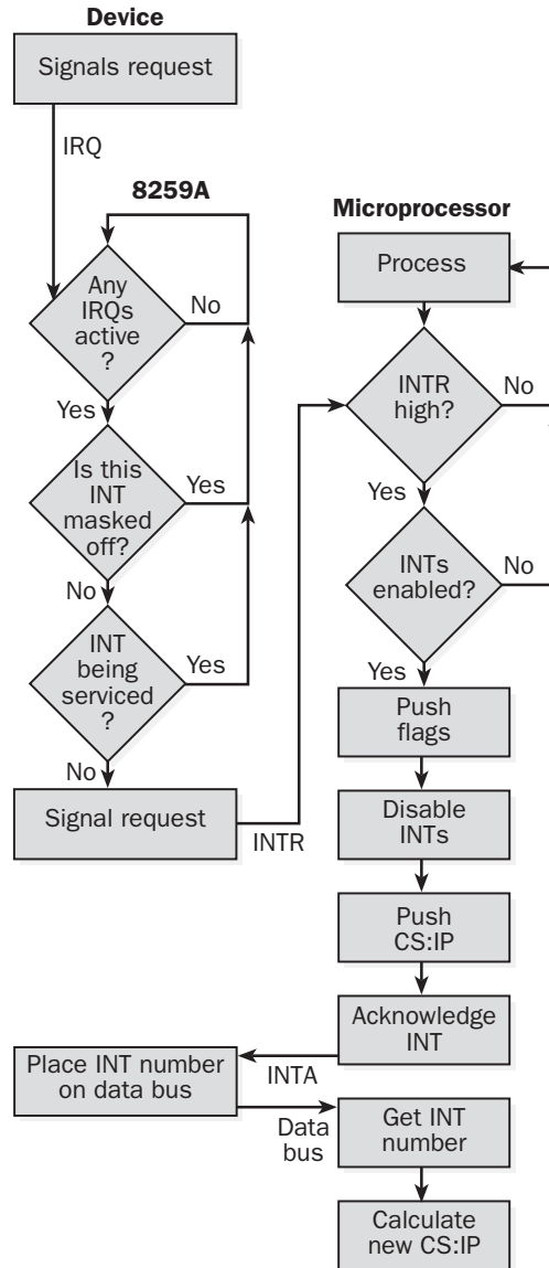
Flowchart.
