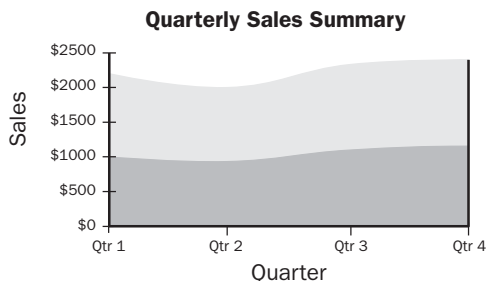
Area chart.
