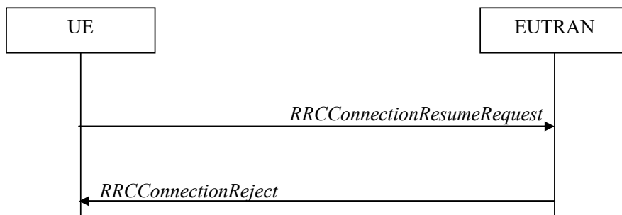
Figure 5: RRC connection resume, network reject or release
