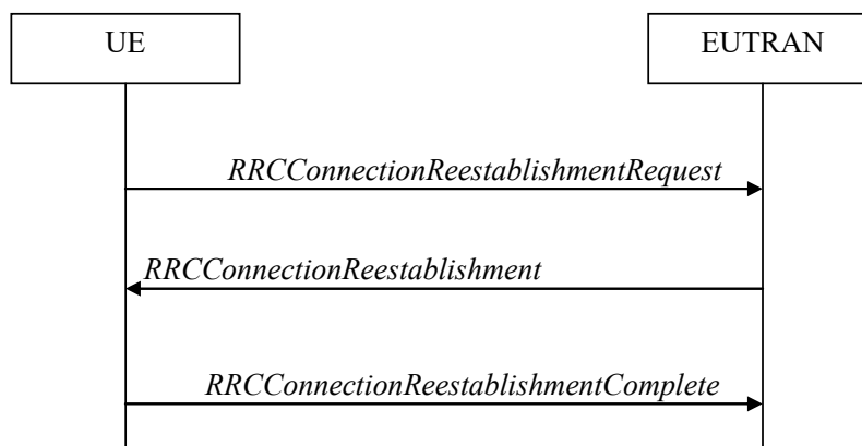
Figure 1: RRC connection re-establishment, successful
