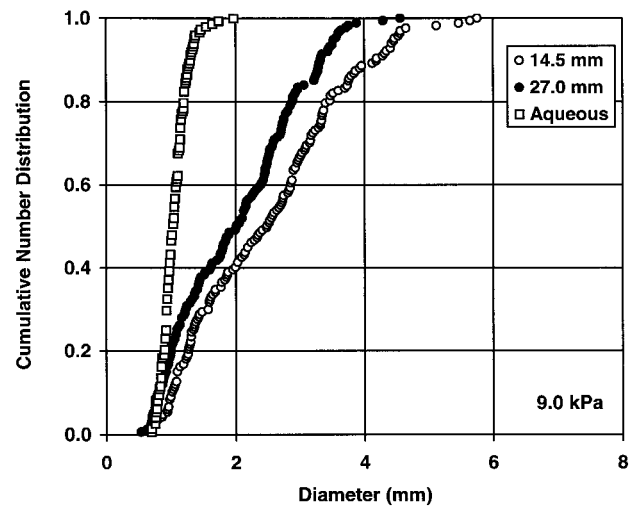
FIG. 4. Cumulative Size Distribution of Bubbles as Function of Particle Size
