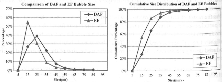
Figure 6 Comparison of DAF and EF bubble size distribution
