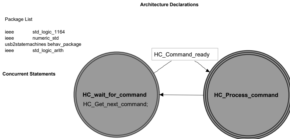
Figure 11-34. Host Controller
