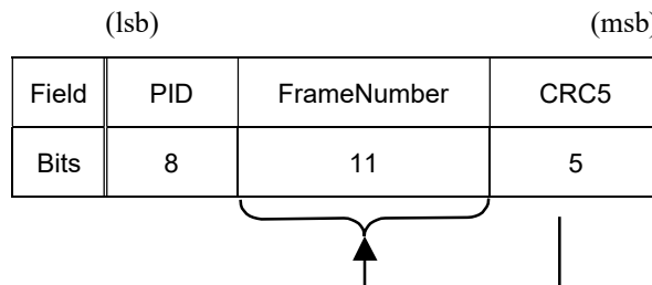
Figure 8-13. SOF Packet
