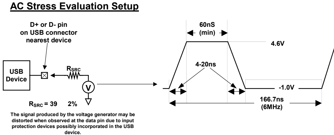
Figure 7-2. Maximum Input Waveforms for USB Signaling
