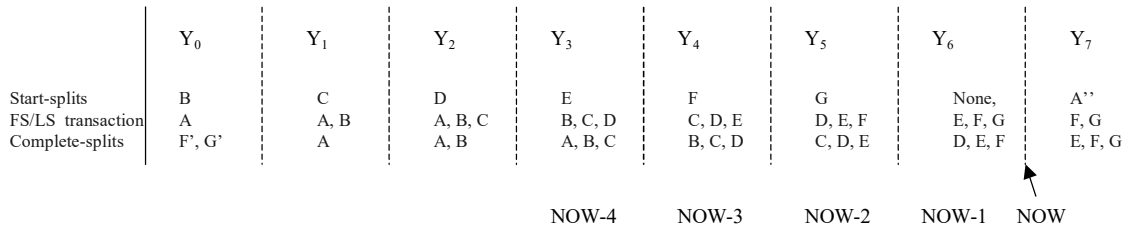
Figure 11-66. Microframe Pipeline
