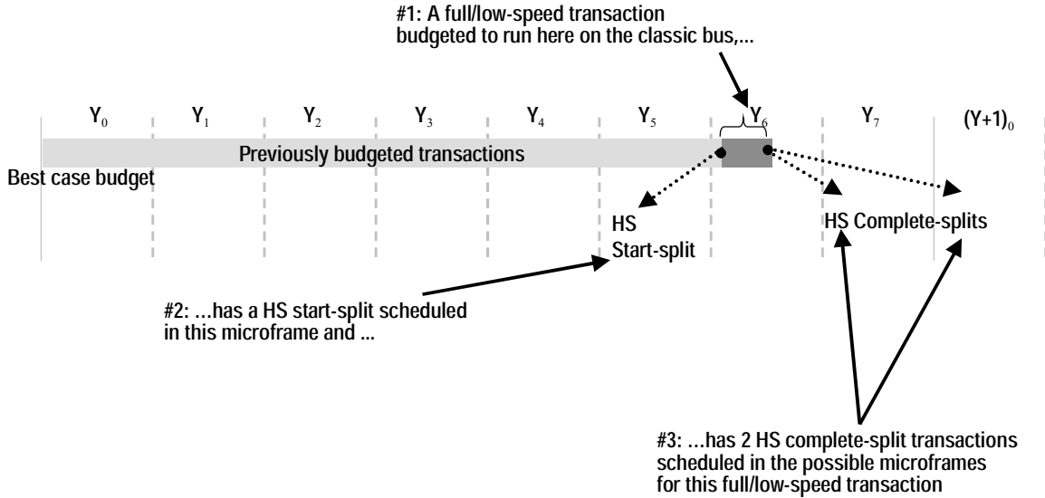
Figure 11-63. End of Frame TT Pipeline Scheduling Example
