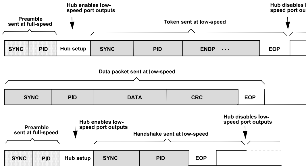
Figure 8-48. Low-speed Transaction
