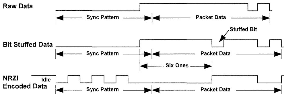
Figure 7-32. Bit Stuffing
