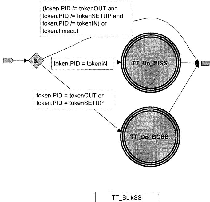
Figure 11-42. TT_BulkSS
