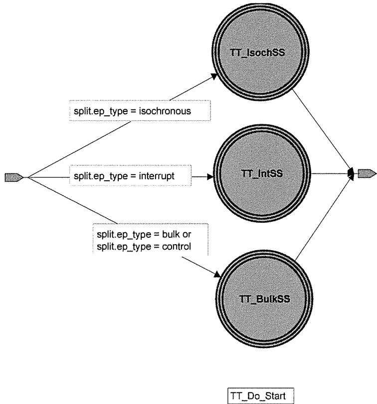
Figure 11-40. TT_Do_Start
