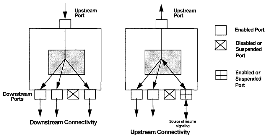
Figure 11-3. Resume Connectivity
