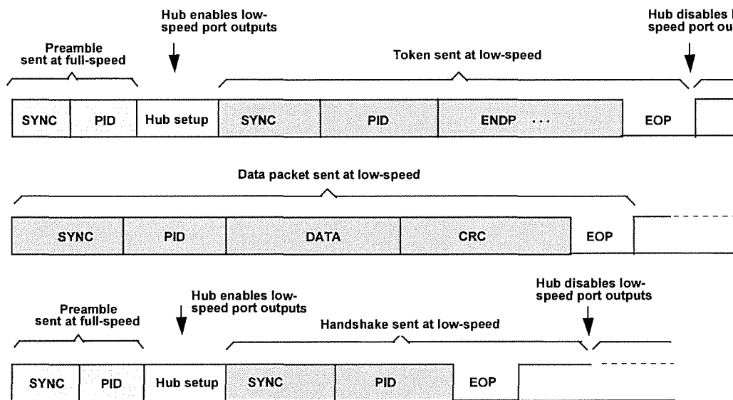
Figure 8-48. Low-speed Transaction
