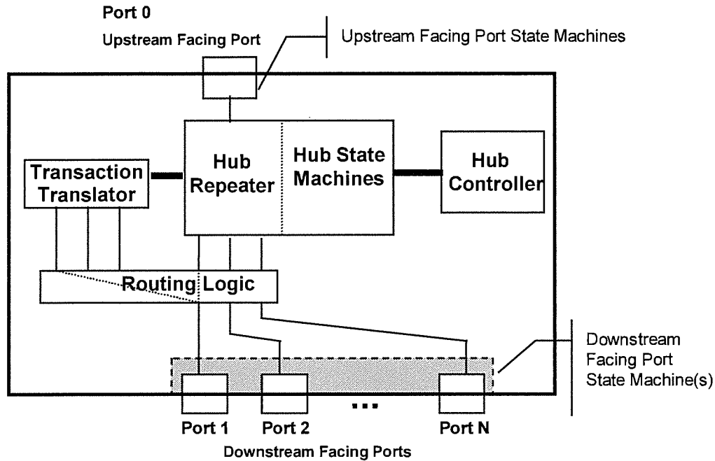
Figure 11-1. Hub Architecture
