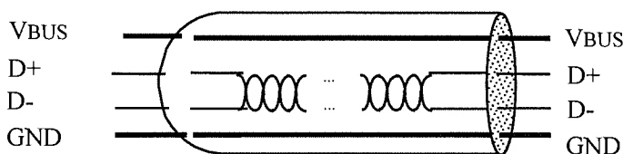
Figure 4-2. USB Cable
