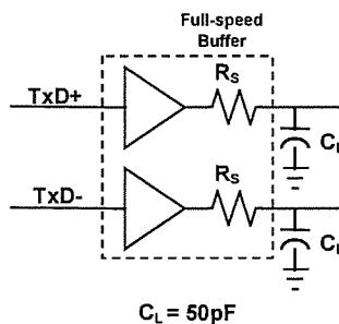
Figure 7-9. Full-speed Load
