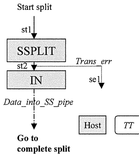
Figure 11-84. Isochronous IN Start-split Transaction Sequence
