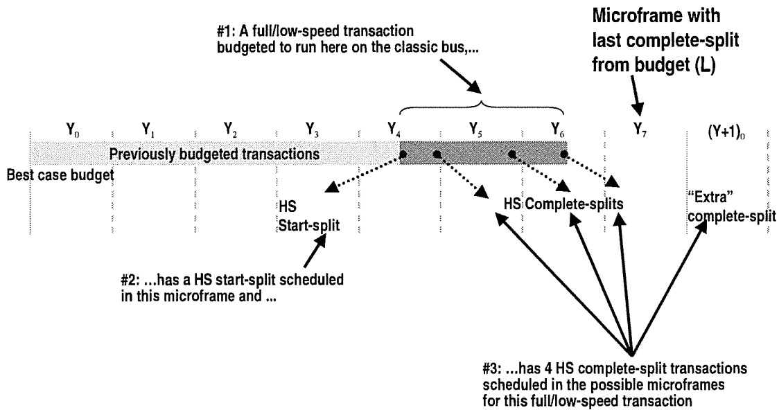
Figure 11-65. Isochronous IN Complete-split Schedule Example at L=Y
