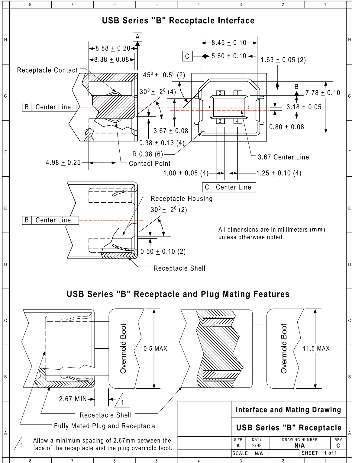
Figure 6-8. USB Series "B" Receptacle Interface and Mating Drawing
