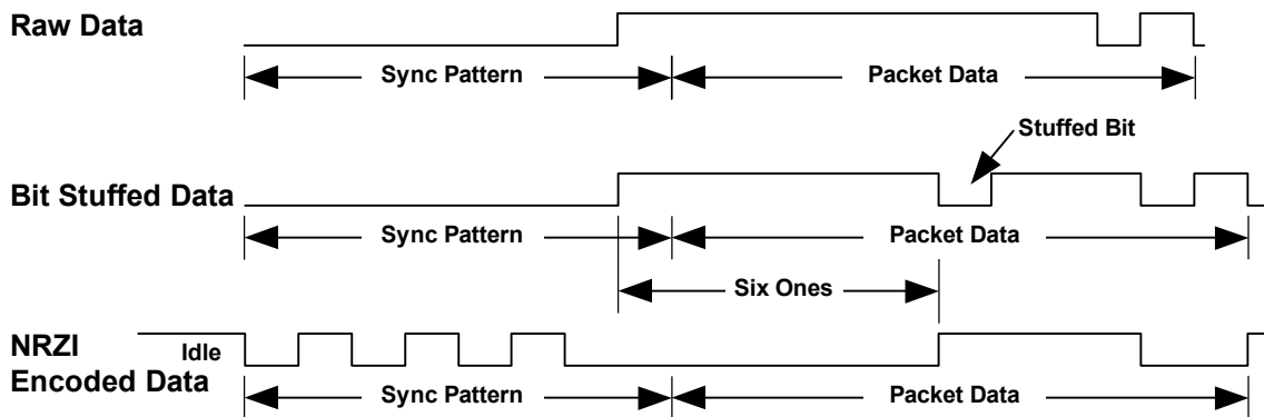
Figure 7-22. Bit Stuffing
