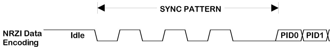
Figure 7-25. Sync Pattern
