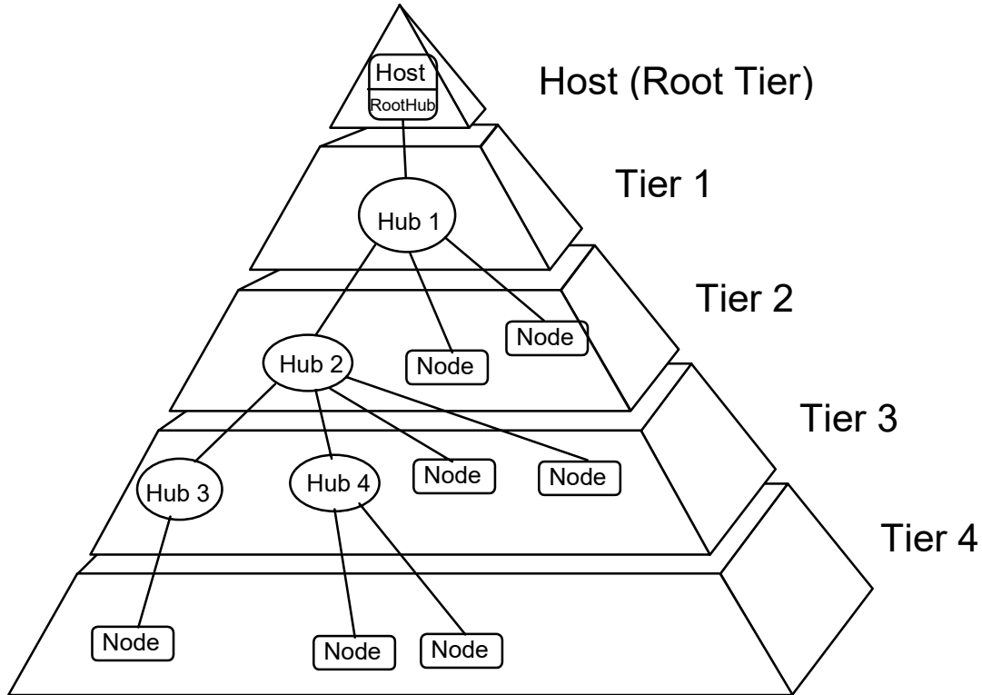
Figure 4-1. Bus Topology
