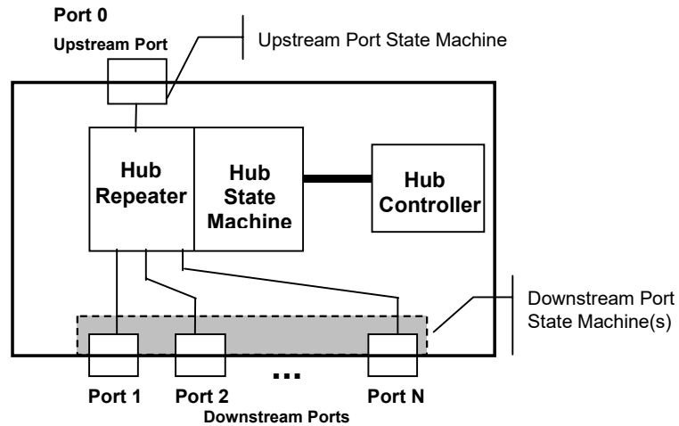
Figure 11-1. Hub Architecture
