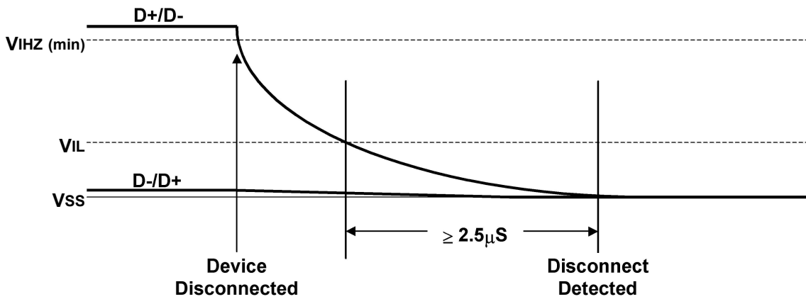
Figure 7-15. Disconnect Detection
