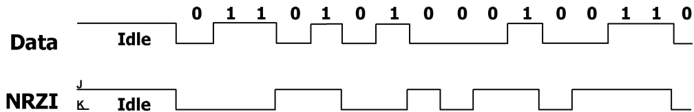
Figure 7-21. NRZI Data Encoding
