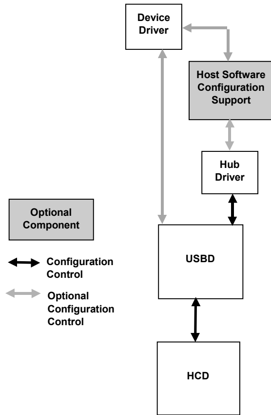
Figure 10-4. Configuration Interactions
