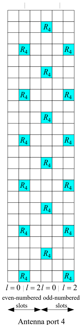
Figure 6.10.2.2-3: Mapping of MBSFN reference signals (extended cyclic prefix, \Delta f = 7.5 kHz)
