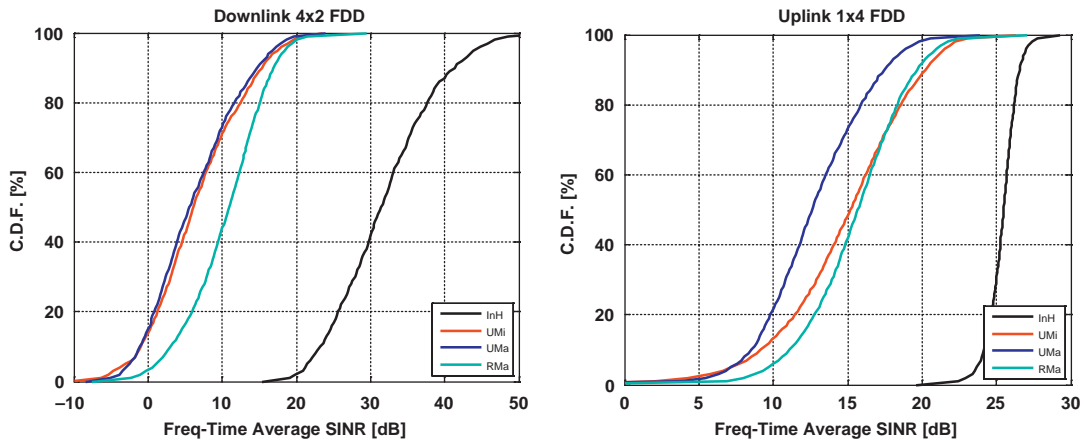
FIGURE 18.4 FDD SINR distributions (downlink and uplink).
