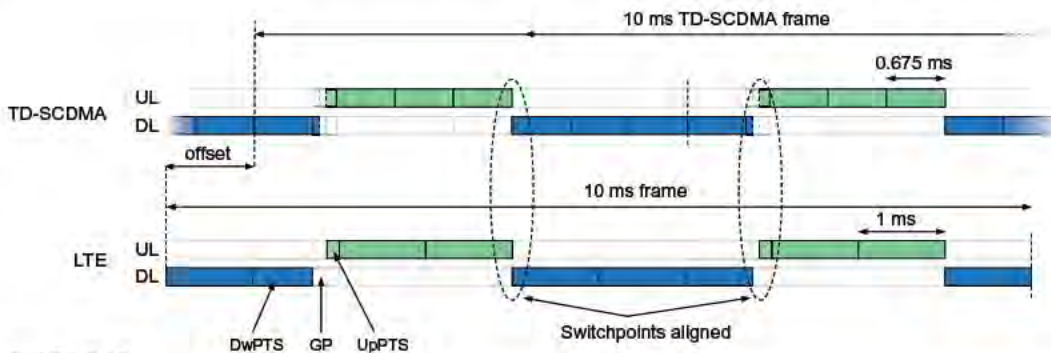
FIGURE 9.13 Coexistence between TD-SCDMA and LTE.
