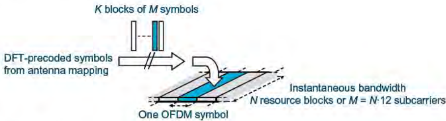
FIGURE 11.3 Mapping to the uplink physical resource.
