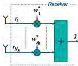
FIGURE 5.1 Linear receive-antenna combination.
