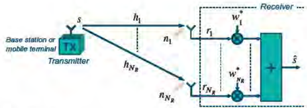
FIGURE 5.2 Channel gains together with linear receive-antenna combination.
