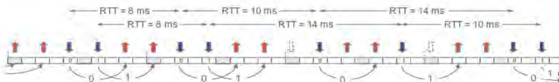
FIGURE 16.6 Example of hybrid-ARQ process numbering for FDD.
