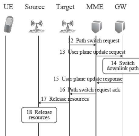
Figure 7.9 Handover completion
