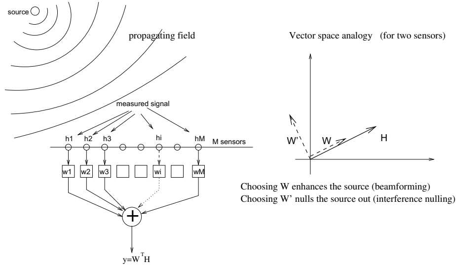
Figure 11.4: The beamforming and interference cancelling concepts.
