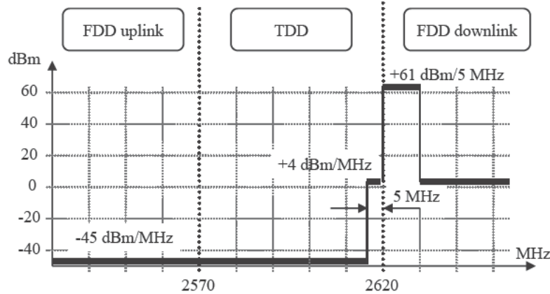
Figure 11.8 Out-of-block EIRP emission mask (BEM) for a 10 MHz FDD block above the TDD band allocation
