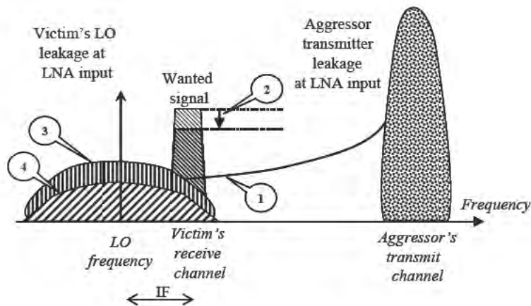
Figure 11.24 Desensitization mechanisms
