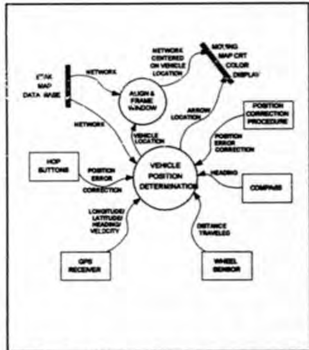
Figure 31. Vehicle navigation data flow.
