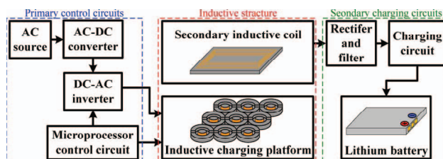
Figure 1. The framework of contactless inductive charging platform.
