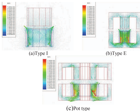
Figure 3. The simulation of magnetic field for each core type.
