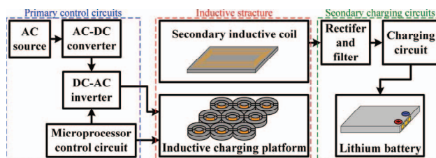
Figure 1. The framework of contactless inductive charging platform.
